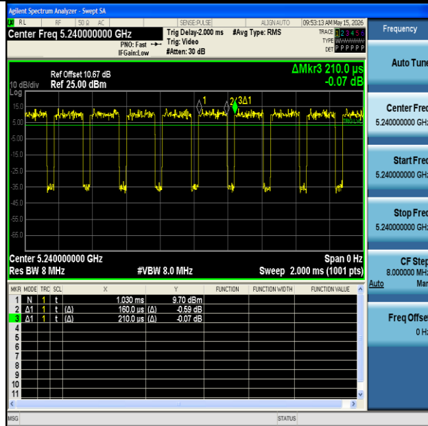
NTNV-11AC20MIMO-Ant1-5240
