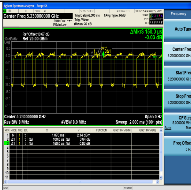
NTNV-11AC40MIMO-Ant2-5230
