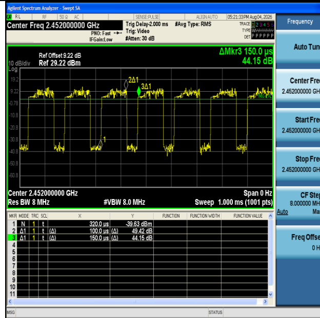
NTNV-11N40MIMO-Ant1-2452
