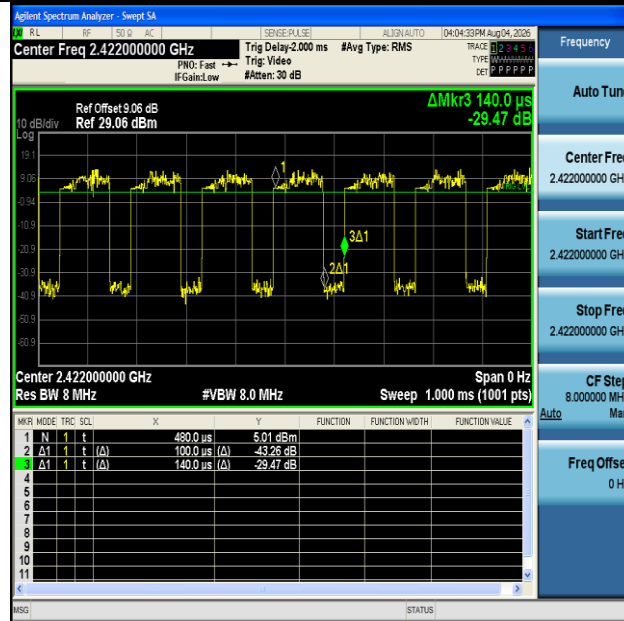
NTVN-11N40MIMO-Ant1-2422
