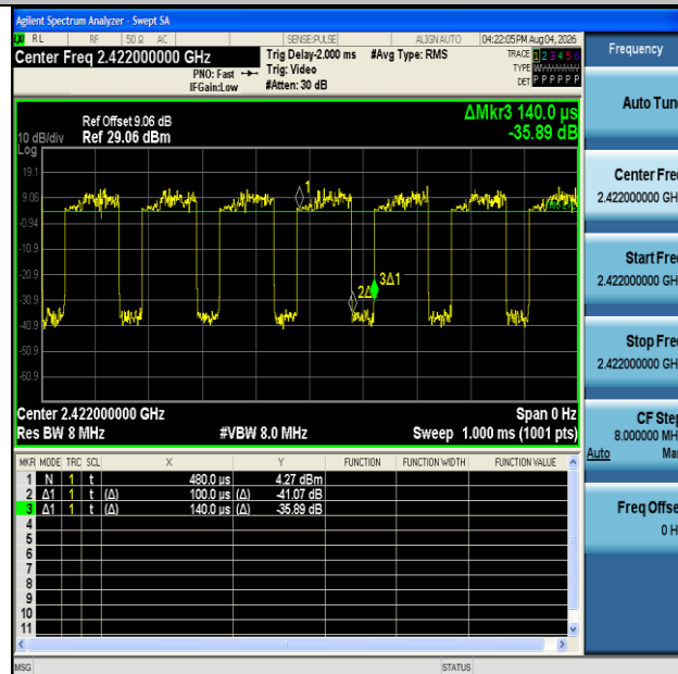
NTVN-11N40MIMO-Ant2-2422
