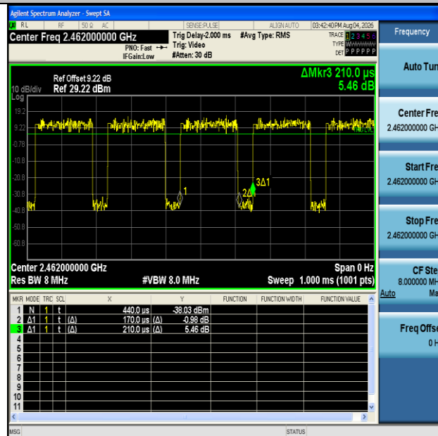
NTNV-11N20MIMO-Ant2-2462
