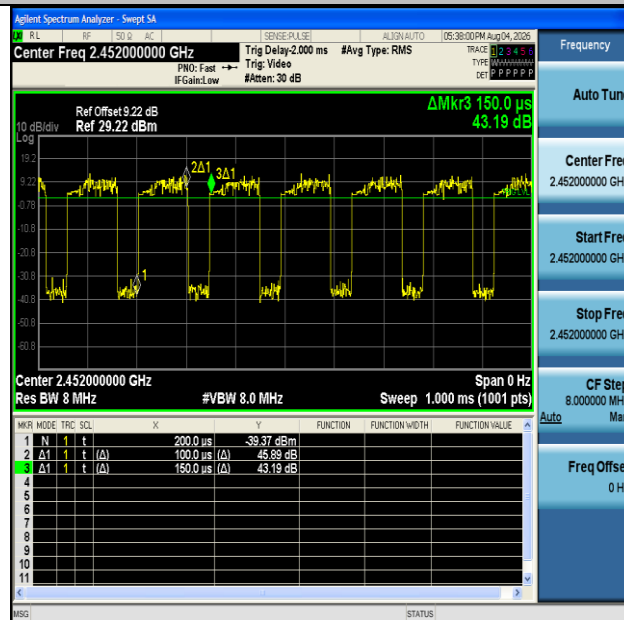
NTNV-11N40MIMO-Ant2-2452
