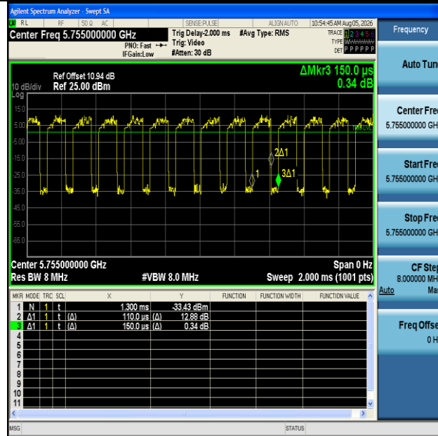
NTNV-11AC40MIMO-Ant1-5755
