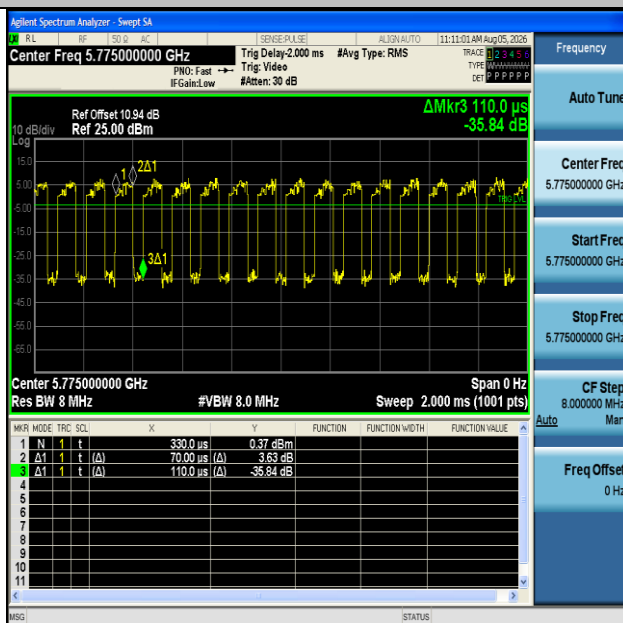
NTNV-11AC80MIMO-Ant2-5775
