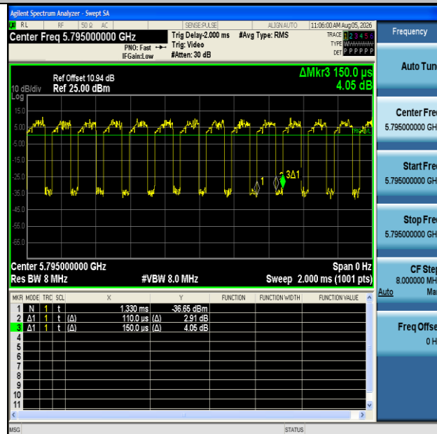
NTNV-11AC40MIMO-Ant2-5795
