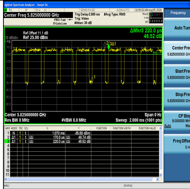
NTNV-11AC20MIMO-Ant1-5825
