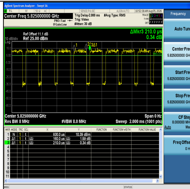
NTNV-11AC20MIMO-Ant2-5825
