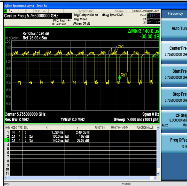
NTNV-11AC40MIMO-Ant2-5755
