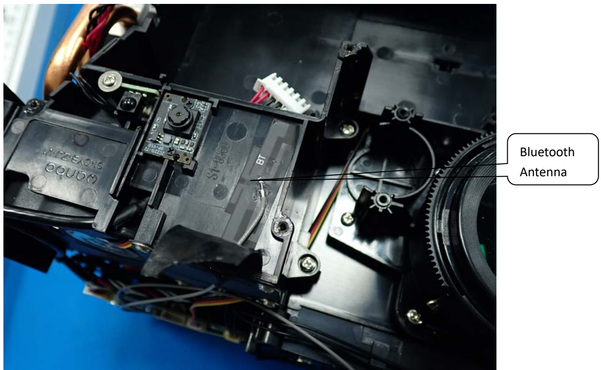
Internal Photo 6
