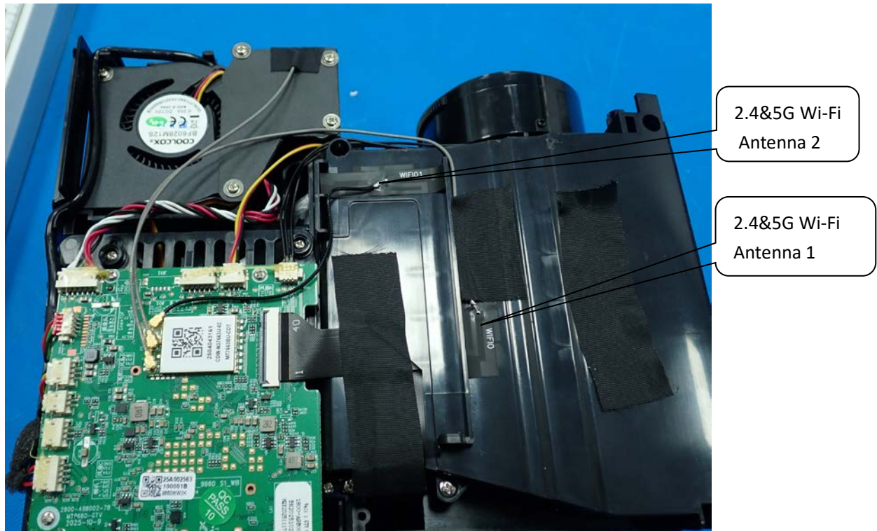
Internal Photo 5
