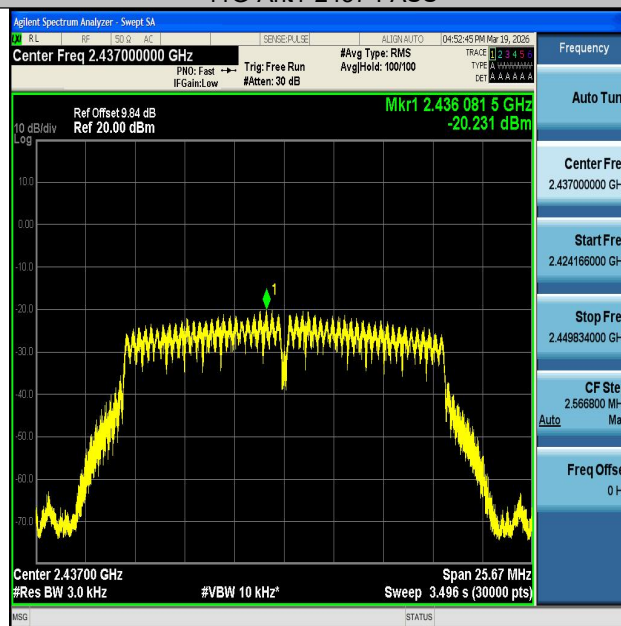
11G-Ant2-2437-PASS
