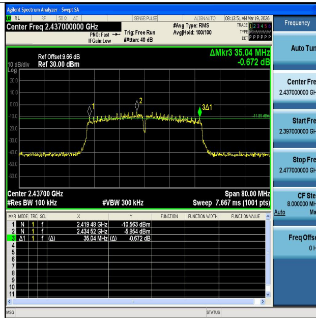
11N40MIMO-Ant1-2437-PASS
