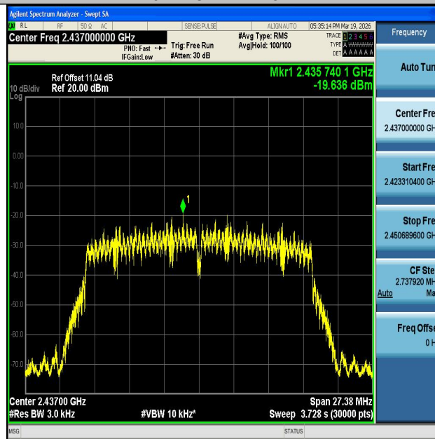
11N20MIMO-Ant2-2437-PASS
