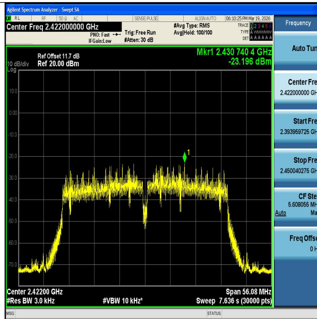
11N40MIMO-Ant1-2422-PASS
