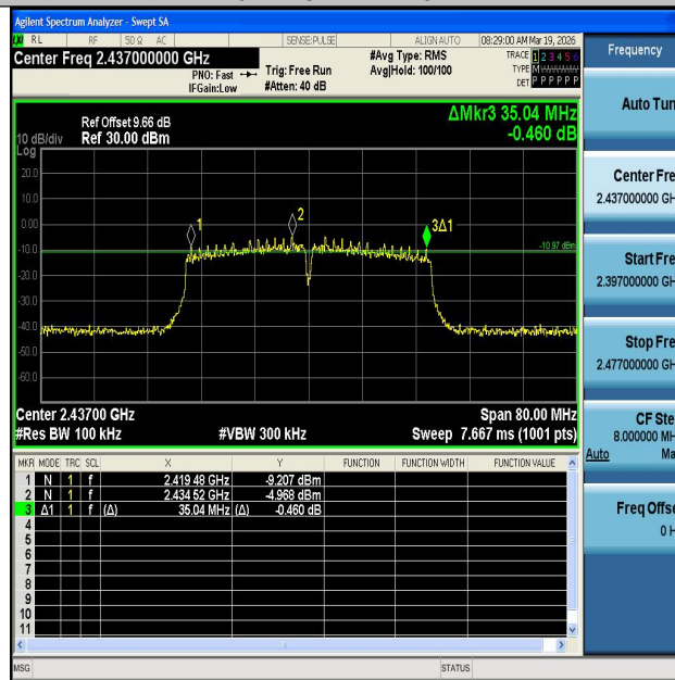
11N40MIMO-Ant2-2437-PASS
