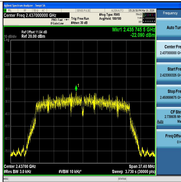
11N20MIMO-Ant1-2437-PASS
