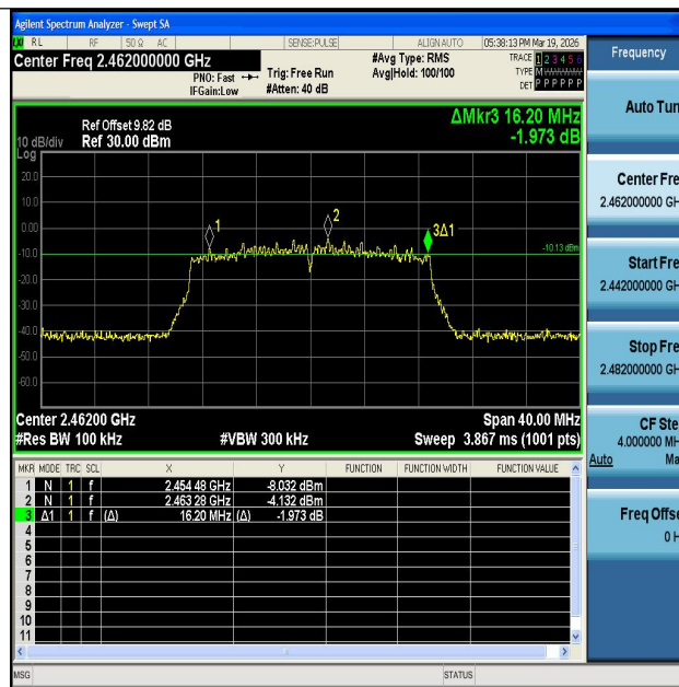
11N20MIMO-Ant1-2462-PASS
