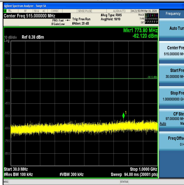
11B-Ant2-2412-30~1000-PASS
