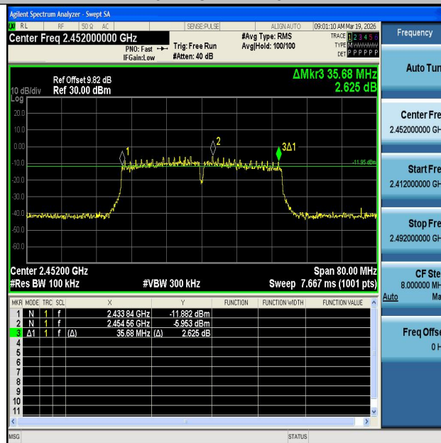
11N40MIMO-Ant2-2452-PASS
