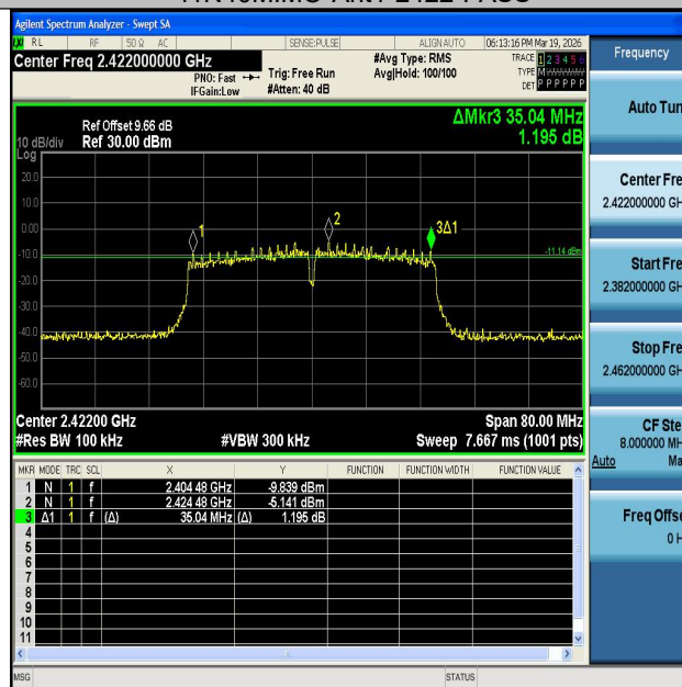
11N40MIMO-Ant2-2422-PASS
