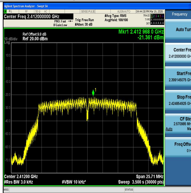
11G-Ant2-2412-PASS
