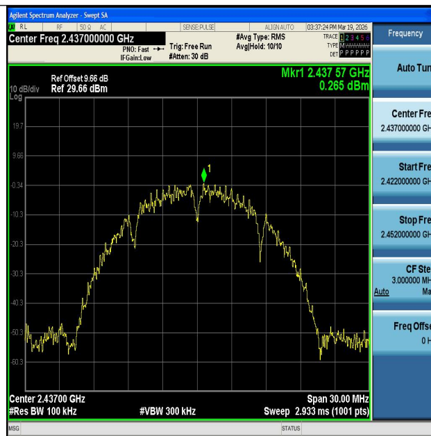
11B-Ant1-2437-0~Reference-PASS
