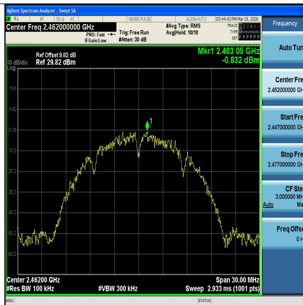
11B-Ant1-2462-0~Reference-PASS
