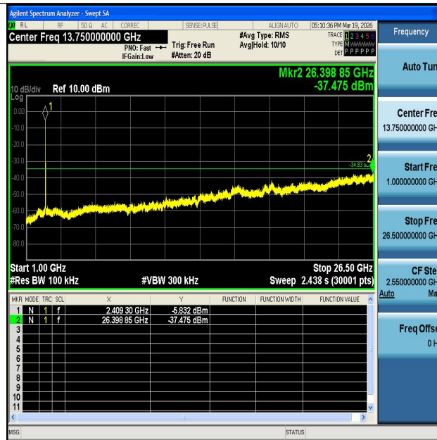
11N20MIMO-Ant1-2412-1000~26500-PASS
