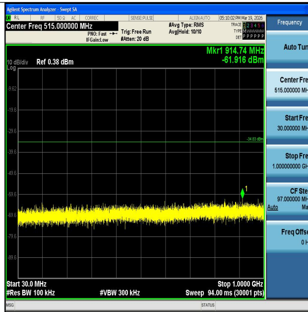
11N20MIMO-Ant1-2412-30~1000-PASS
