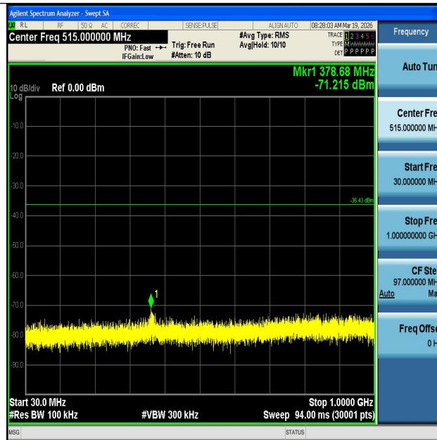
11N40MIMO-Ant1-2437-30~1000-PASS
