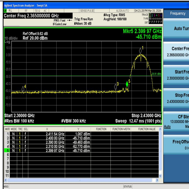
11B-Ant2-2412-PASS
