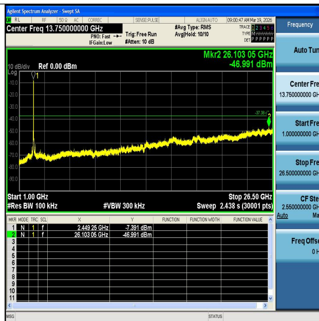
11N40MIMO-Ant1-2452-1000~26500-PASS
