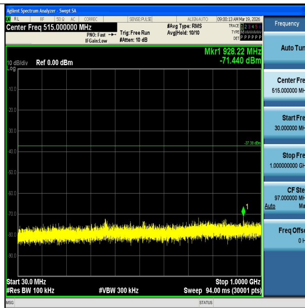
11N40MIMO-Ant1-2452-30~1000-PASS
