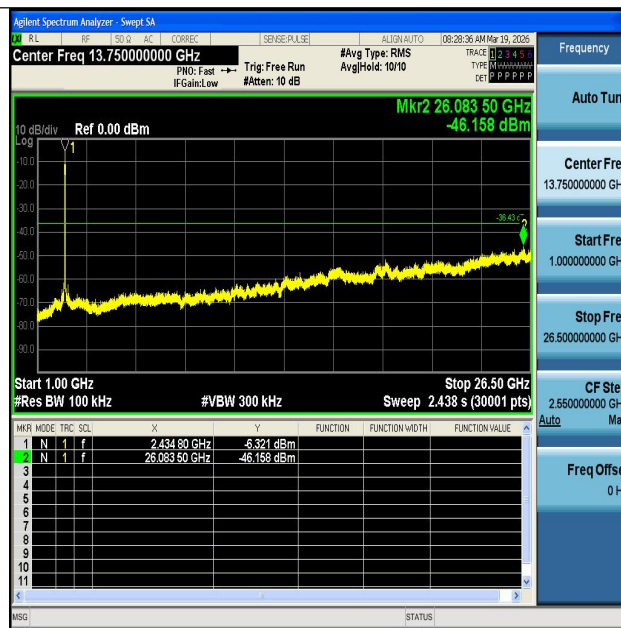
11N40MIMO-Ant1-2437-1000~26500-PASS
