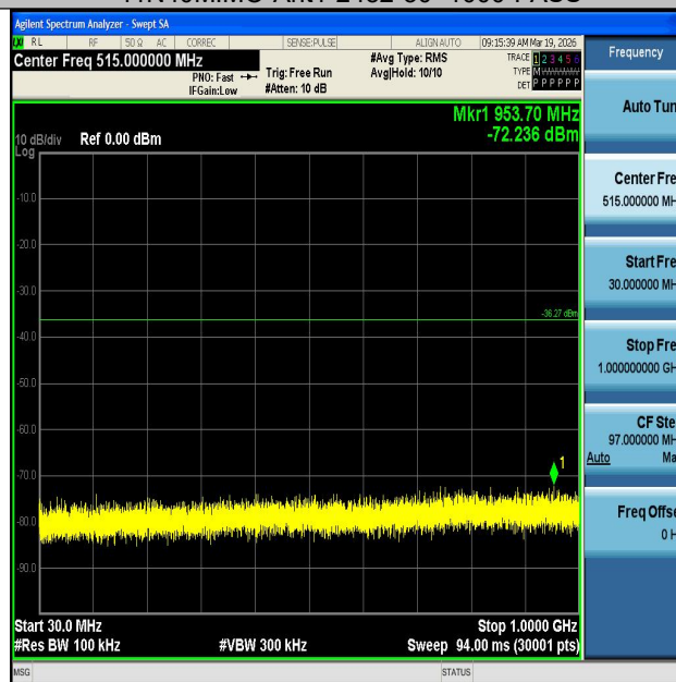
11N40MIMO-Ant2-2452-30~1000-PASS
