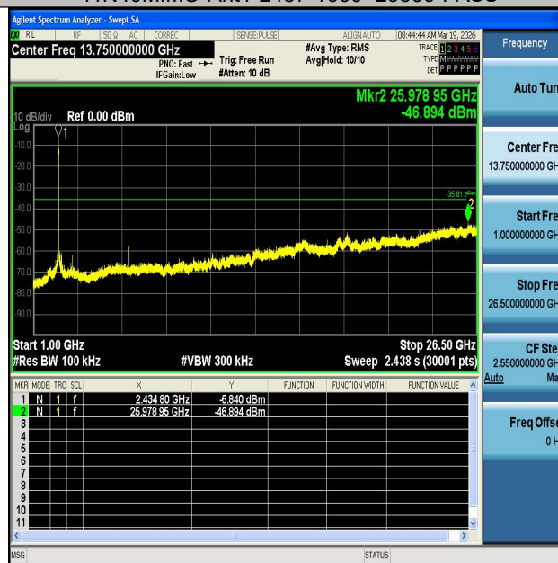
11N40MIMO-Ant2-2437-1000~26500-PASS
