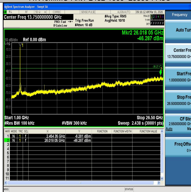
11N40MIMO-Ant2-2452-1000~26500-PASS
