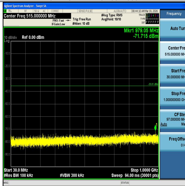
11N40MIMO-Ant2-2437-30~1000-PASS
