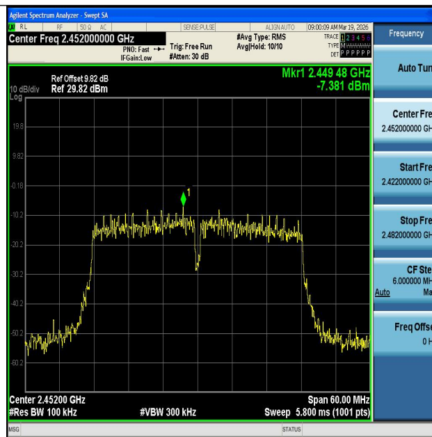
11N40MIMO-Ant1-2452-0~Reference-PASS
