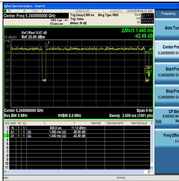
NTNV-11A-Ant2-5240
