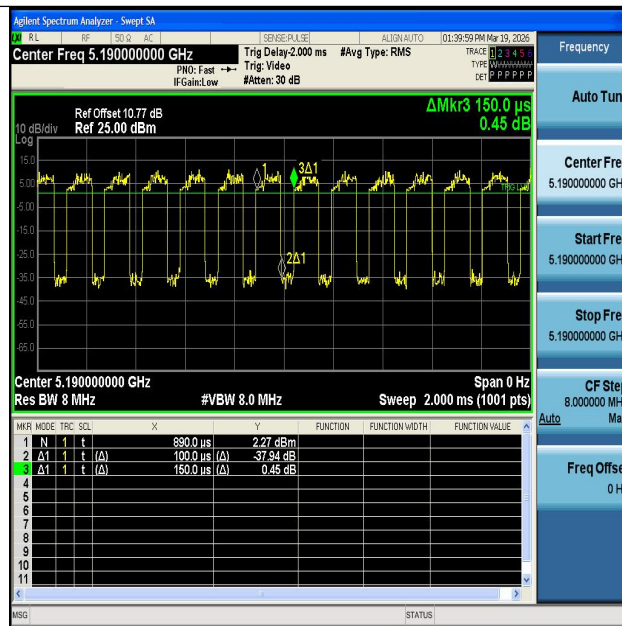
NTNV-11N40MIMO-Ant2-5190
