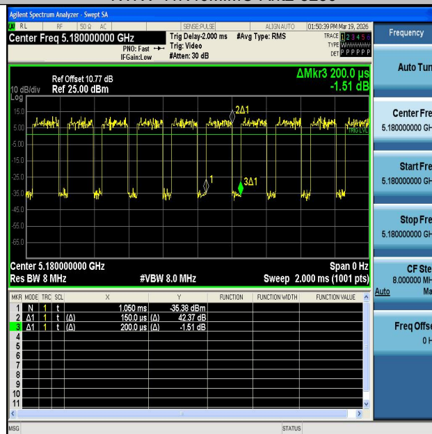
NTNV-11AC20MIMO-Ant1-5180
