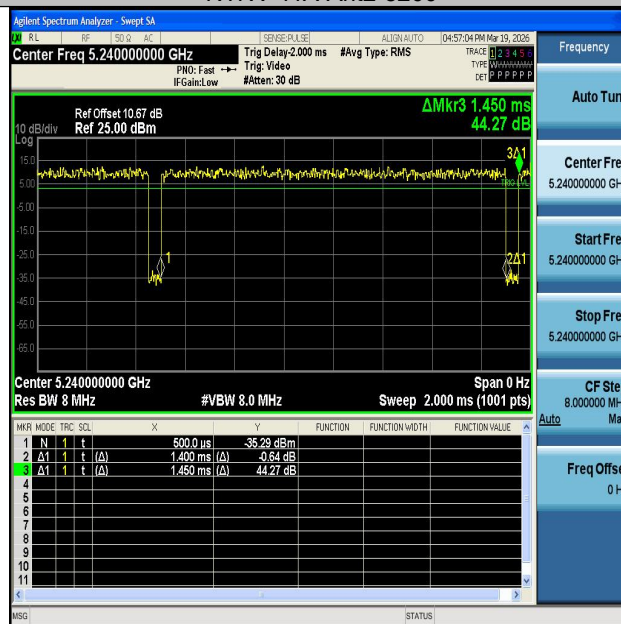
NTNV-11A-Ant1-5240
