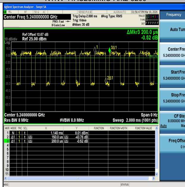
NTNV-11AC20MIMO-Ant1-5240
