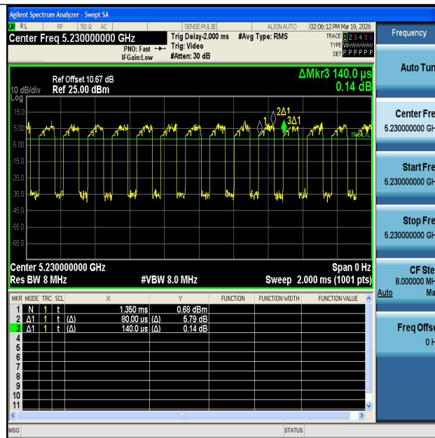
NTNV-11AC40MIMO-Ant2-5230
