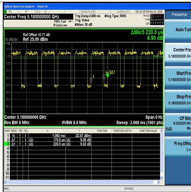
NTNV-11N20MIMO-Ant2-5180
