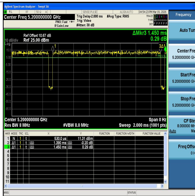
NTNV-11A-Ant2-5200
