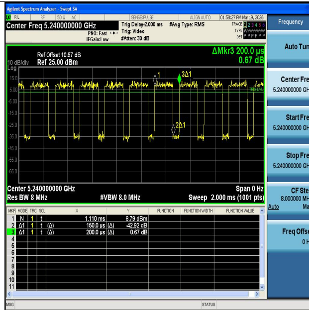
NTNV-11AC20MIMO-Ant2-5240
