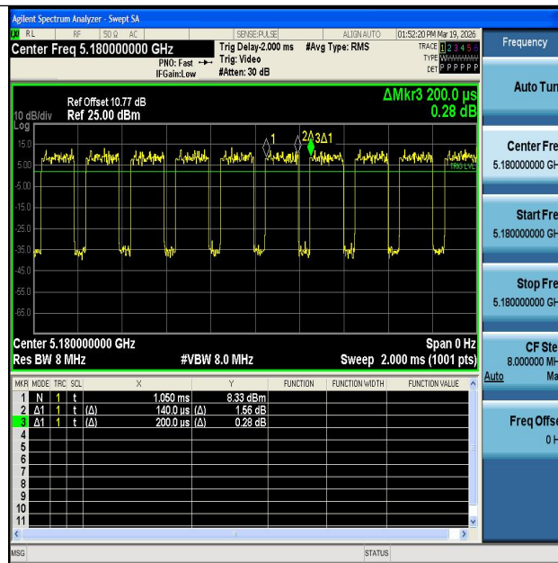
NTNV-11AC20MIMO-Ant2-5180
