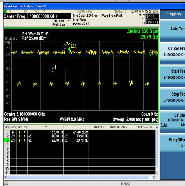
NTNV-11N20MIMO-Ant1-5180
