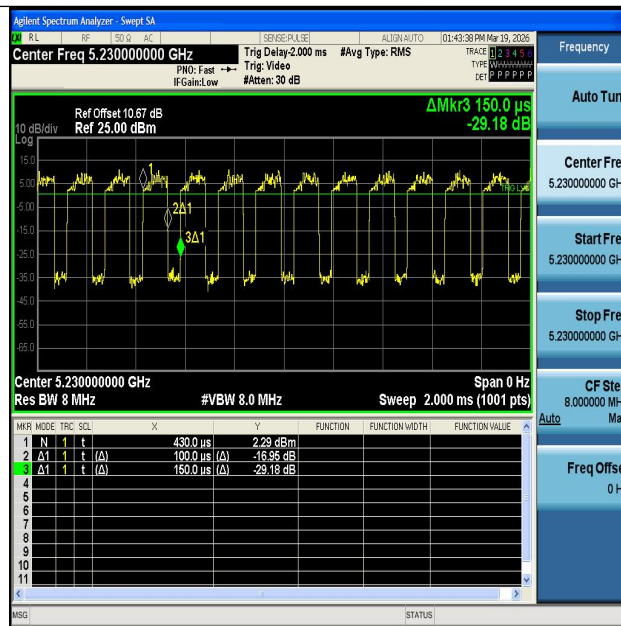
NTNV-11N40MIMO-Ant2-5230
