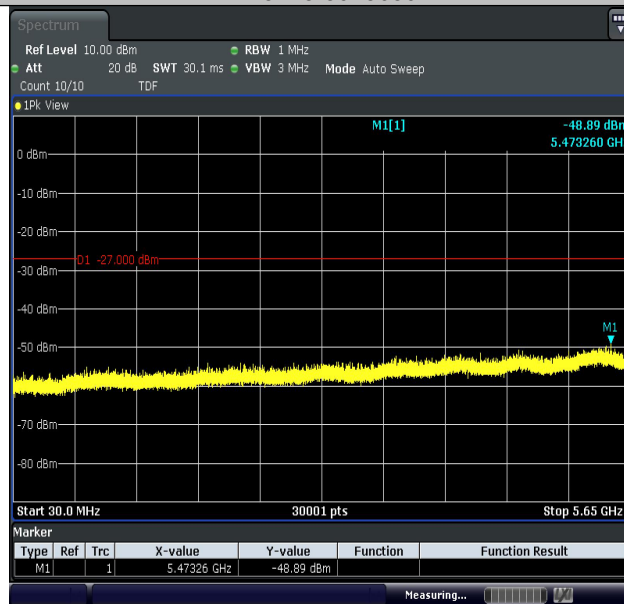
11A-Ant2-5745-30~5650-PASS
