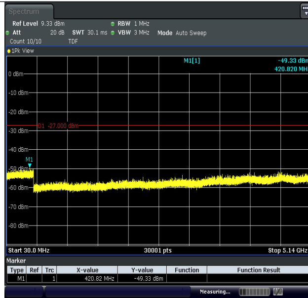
11AC80MIMO-Ant1-5210-30~5140-PASS
