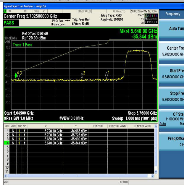
11AC20MIMO-Ant2-5745-PASS
