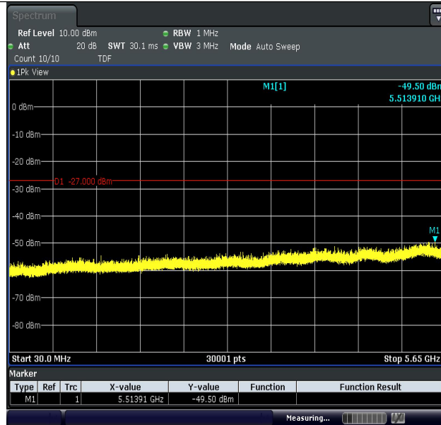
11A-Ant1-5745-30~5650-PASS
