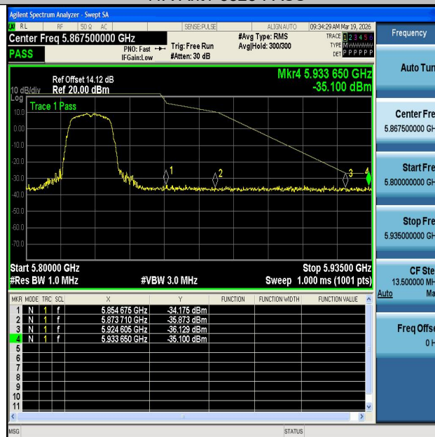
11A-Ant2-5825-PASS
