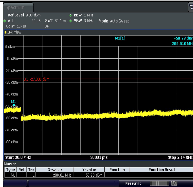
11AC80MIMO-Ant2-5210-30~5140-PASS
