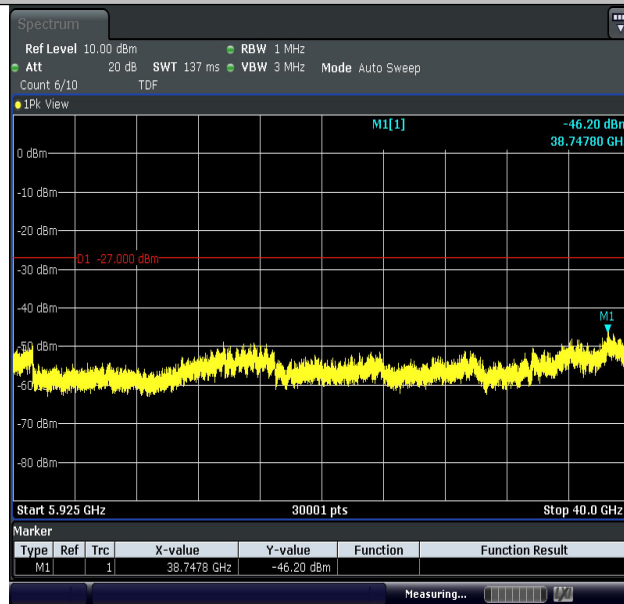
11AC20MIMO-Ant2-5745-5925~40000-PASS
