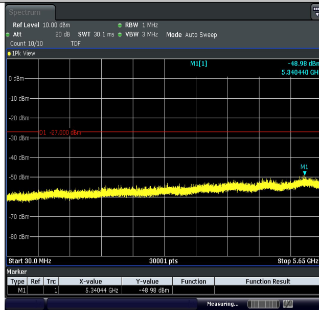
11AC20MIMO-Ant2-5745-30~5650-PASS
