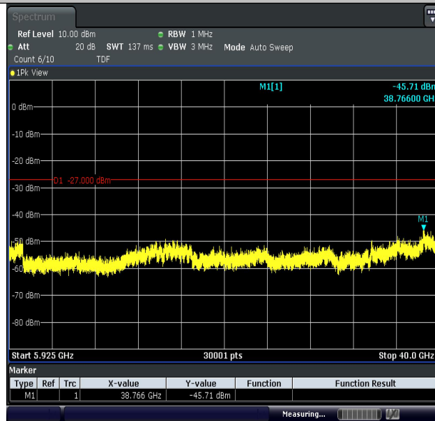
11AC20MIMO-Ant2-5785-5925~40000-PASS
