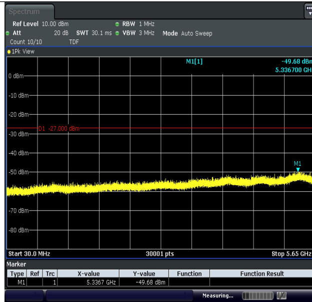
11AC20MIMO-Ant1-5785-30~5650-PASS
