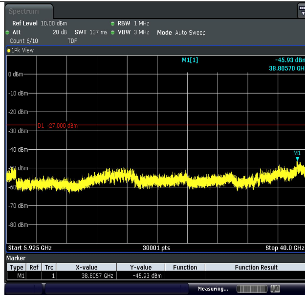
11AC40MIMO-Ant1-5755-5925~40000-PASS
