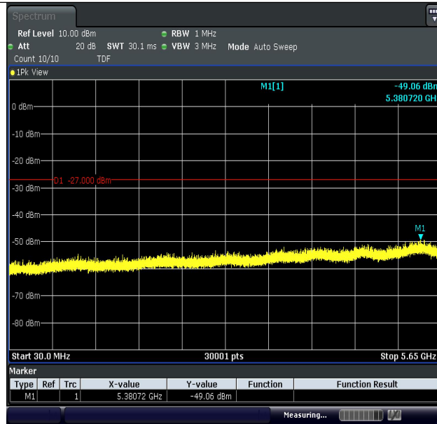
11AC40MIMO-Ant1-5795-30~5650-PASS
