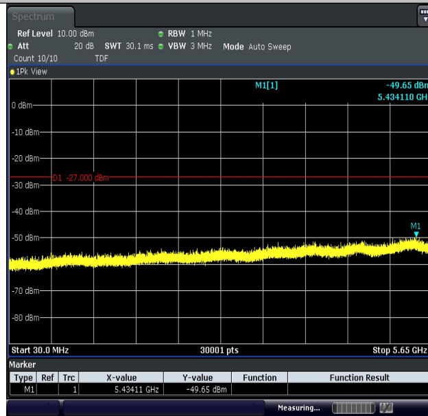
11AC20MIMO-Ant2-5785-30~5650-PASS
