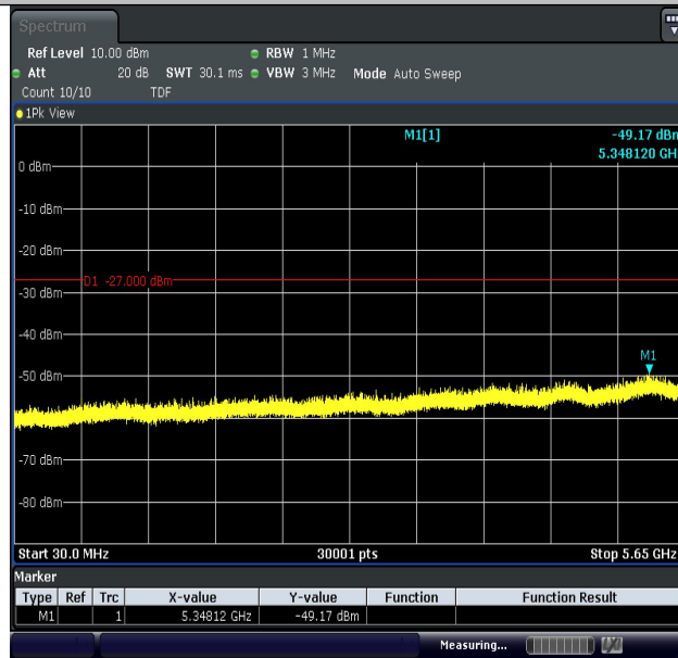
11AC40MIMO-Ant2-5795-30~5650-PASS
