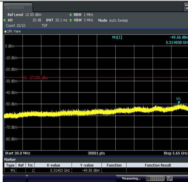
11AC80MIMO-Ant2-5775-30~5650-PASS
