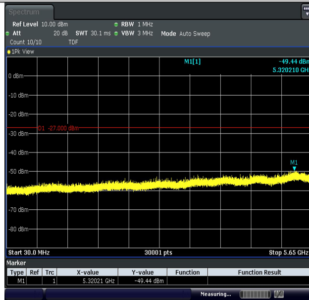
11AC40MIMO-Ant2-5755-30~5650-PASS
