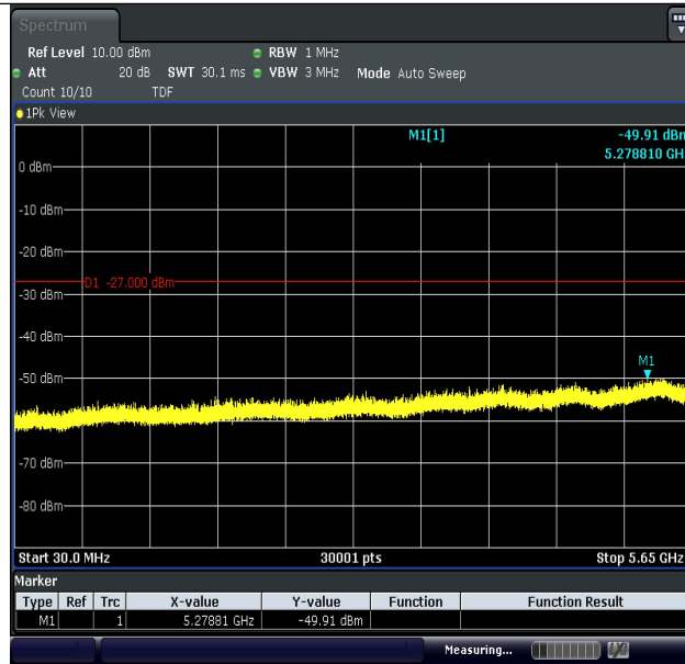
11AC20MIMO-Ant1-5745-30~5650-PASS
