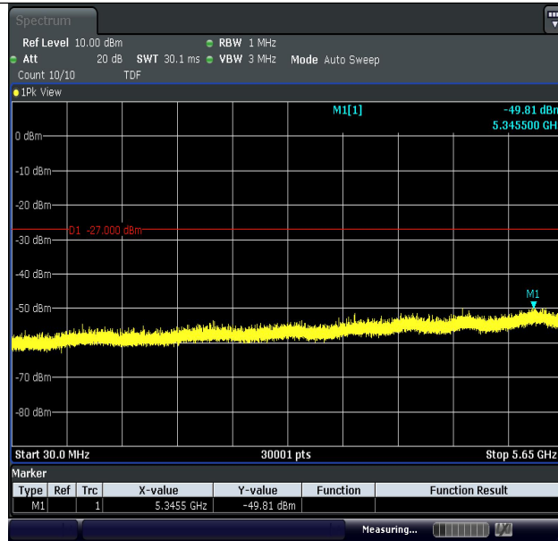
11AC20MIMO-Ant1-5825-30~5650-PASS
