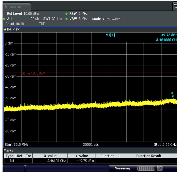
11AC40MIMO-Ant1-5755-30~5650-PASS
