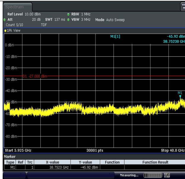
11AC20MIMO-Ant1-5825-5925~40000-PASS
