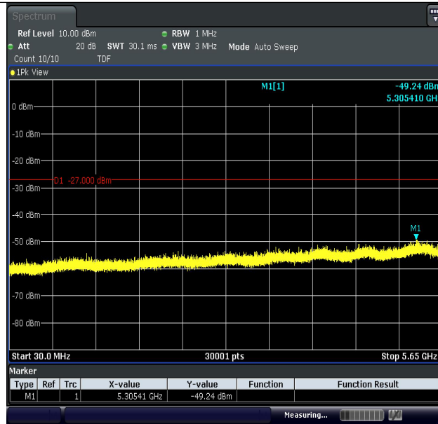
11AC80MIMO-Ant1-5775-30~5650-PASS
