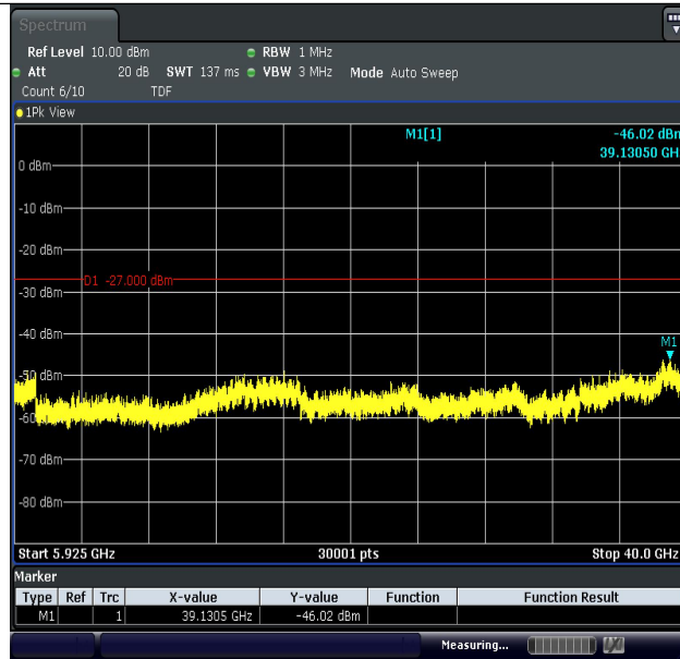
11AC20MIMO-Ant1-5785-5925~40000-PASS
