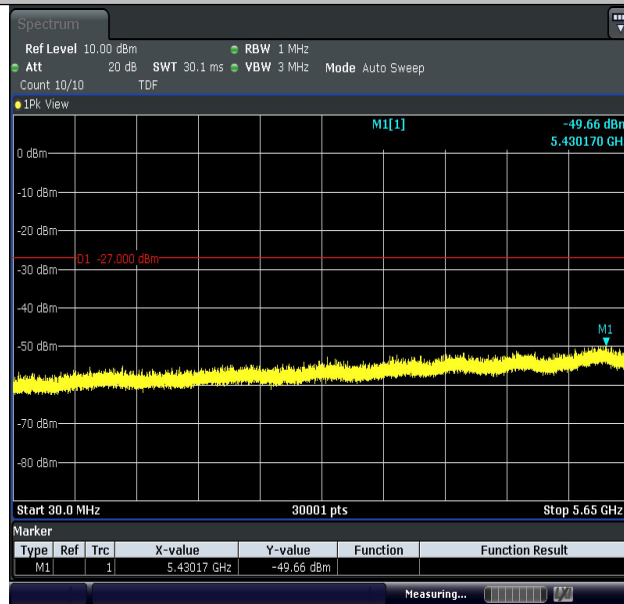
11AC20MIMO-Ant2-5825-30~5650-PASS
