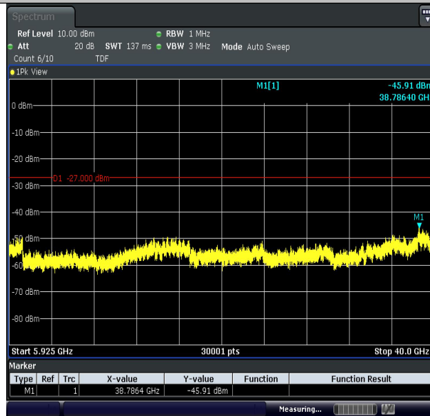
11AC20MIMO-Ant2-5825-5925~40000-PASS
