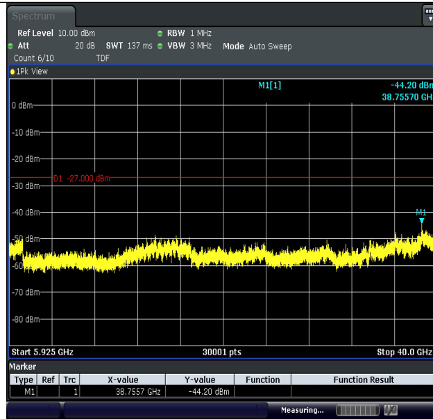
11AC80MIMO-Ant1-5775-5925~40000-PASS
