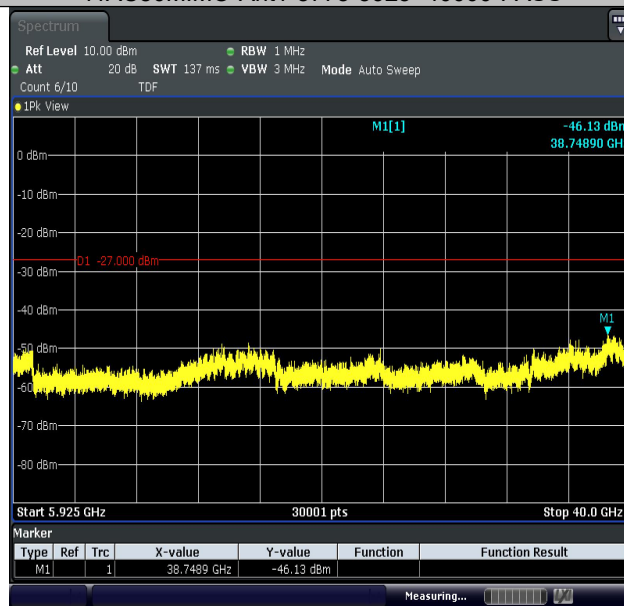
11AC80MIMO-Ant2-5775-5925~40000-PASS
