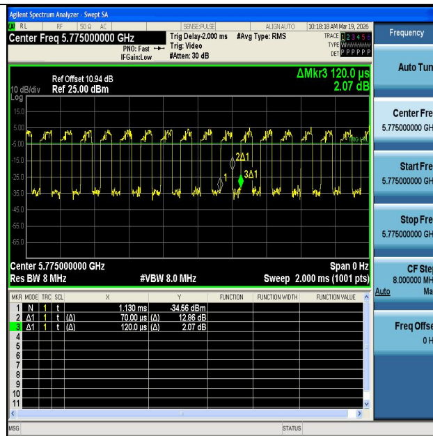
NTNV-11AC80MIMO-Ant1-5775
