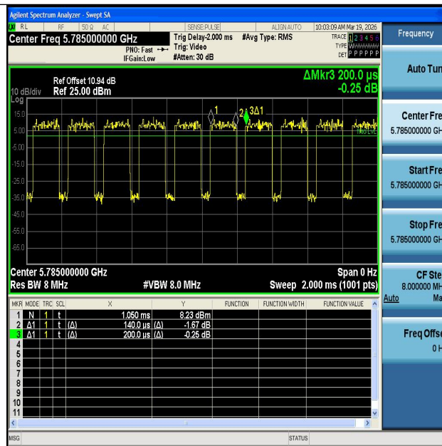
NTNV-11AC20MIMO-Ant1-5785
