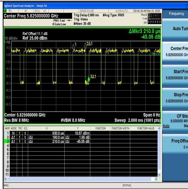
NTNV-11N20MIMO-Ant2-5825
