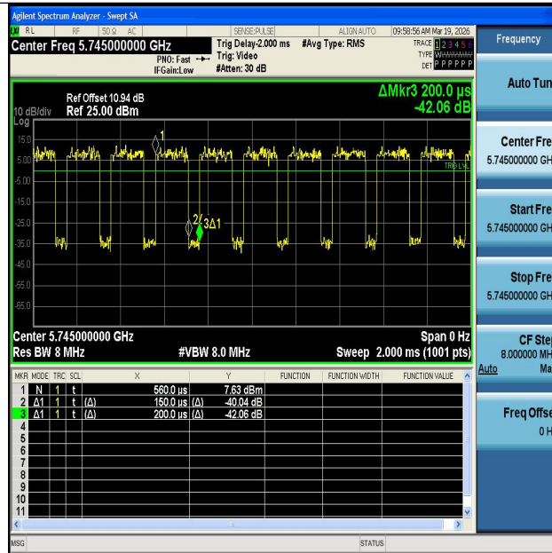
NTNV-11AC20MIMO-Ant1-5745
