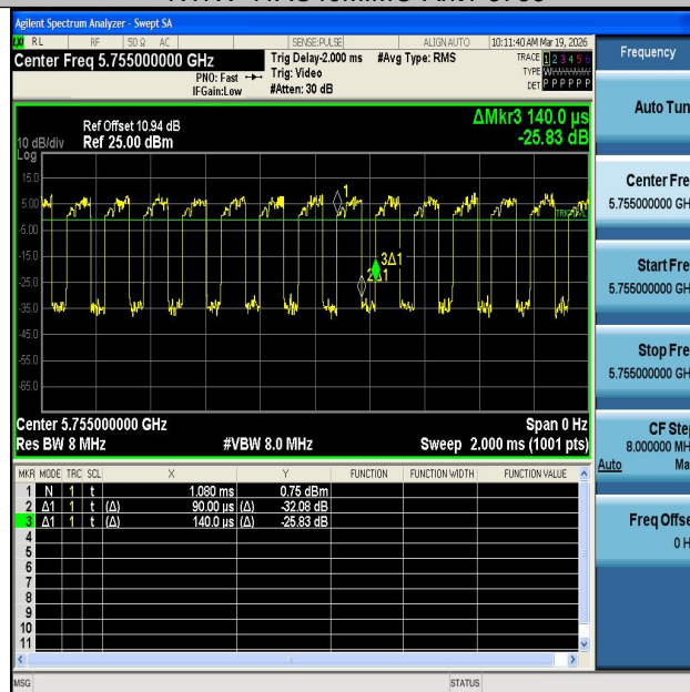
NTNV-11AC40MIMO-Ant2-5755
