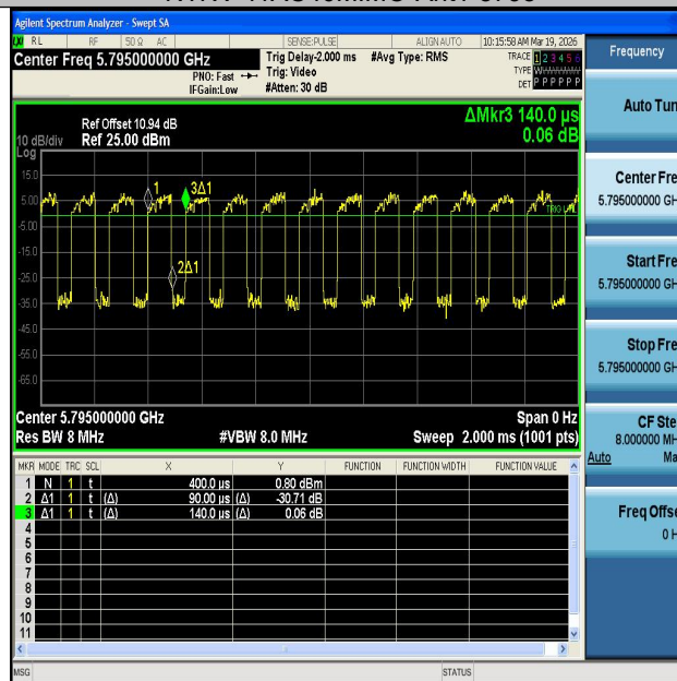
NTNV-11AC40MIMO-Ant2-5795
