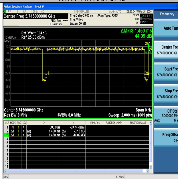
NTNV-11A-Ant2-5745
