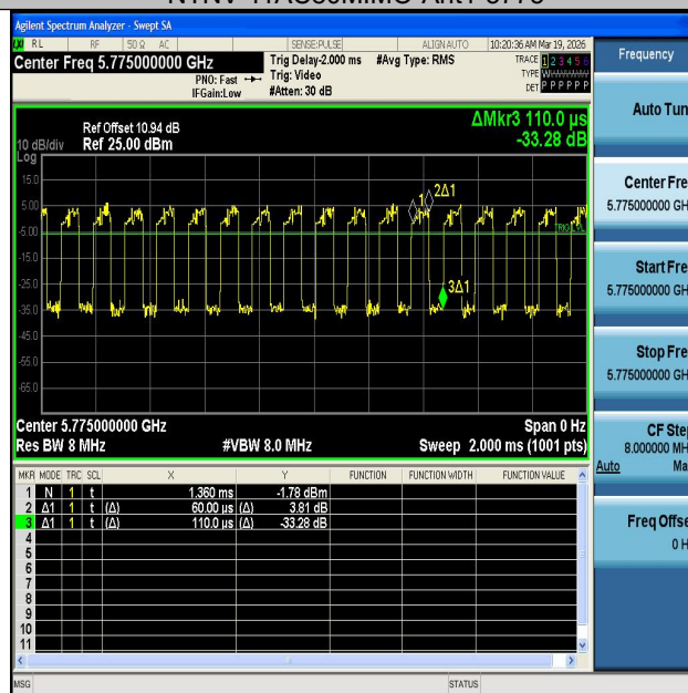
NTNV-11AC80MIMO-Ant2-5775
