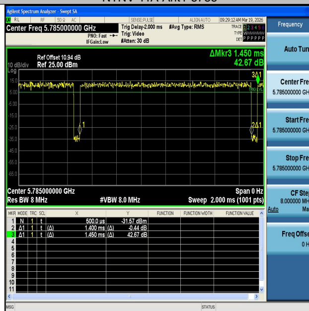
NTNV-11A-Ant2-5785
