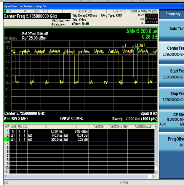
NTNV-11AC20MIMO-Ant2-5785
