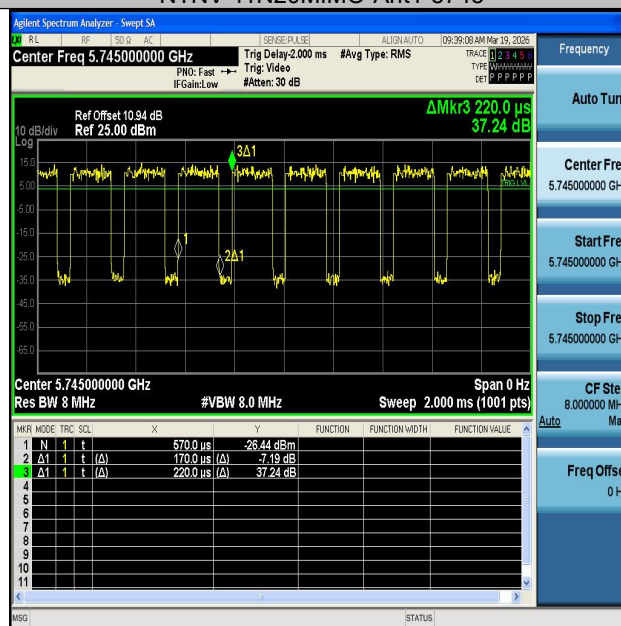
NTNV-11N20MIMO-Ant2-5745
