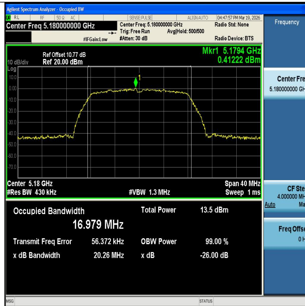
11A-Ant1-5180
