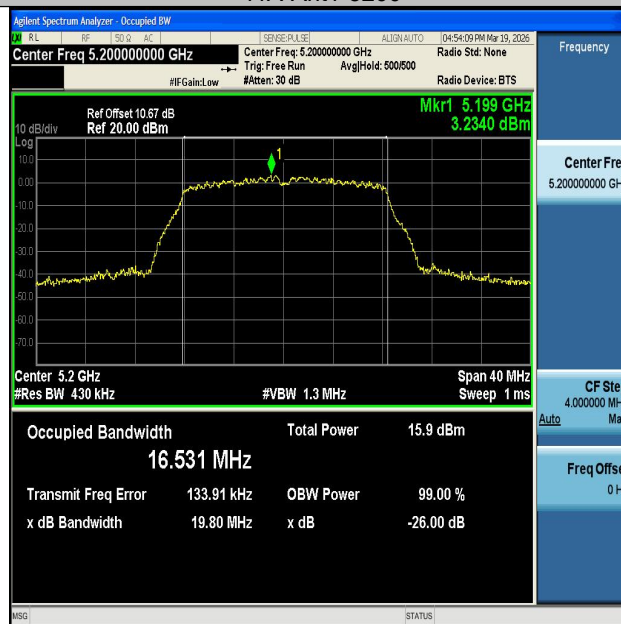
11A-Ant2-5200
