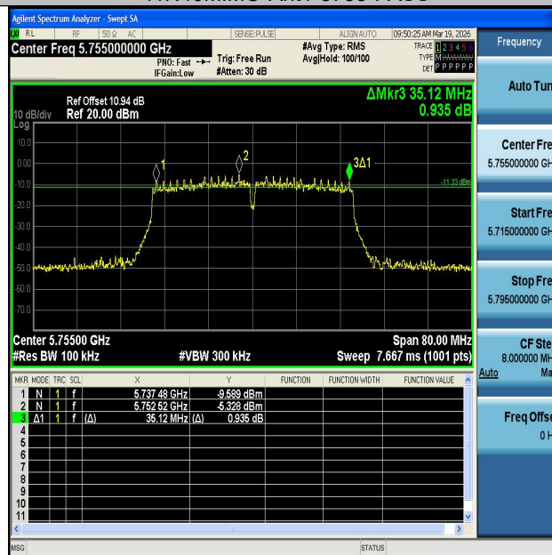
11N40MIMO-Ant2-5755-PASS
