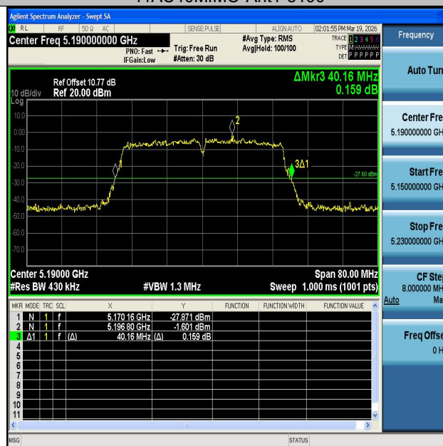
11AC40MIMO-Ant2-5190
