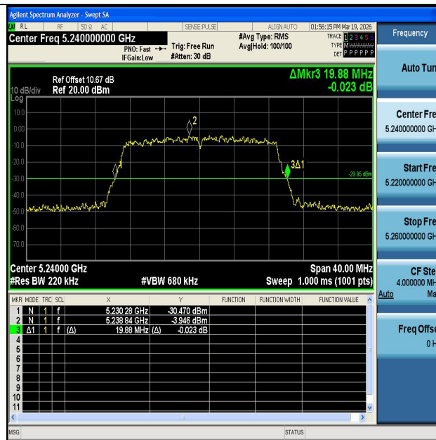
11AC20MIMO-Ant1-5240
