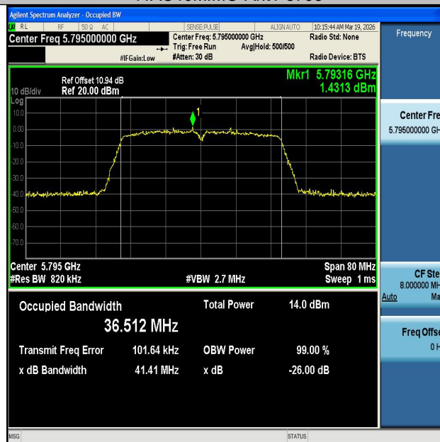
11AC40MIMO-Ant2-5795
