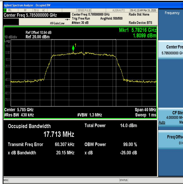
11N20MIMO-Ant1-5785
