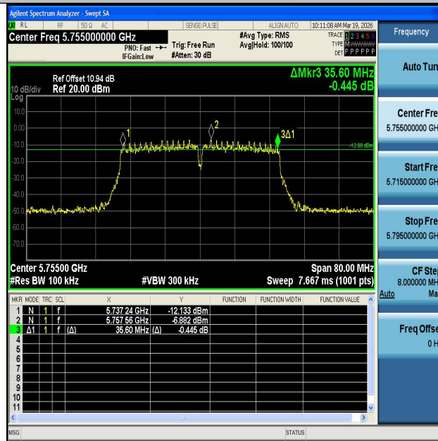
11AC40MIMO-Ant2-5755-PASS
