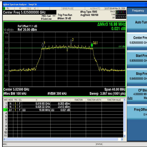
11AC20MIMO-Ant2-5825-PASS
