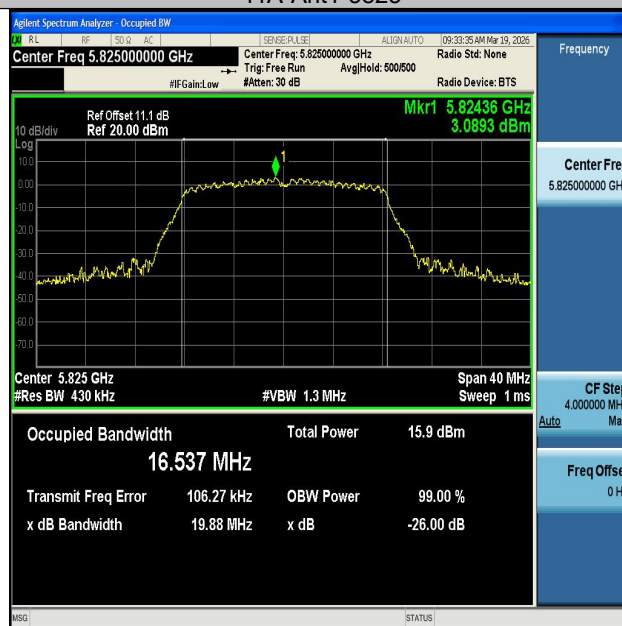
11A-Ant2-5825
