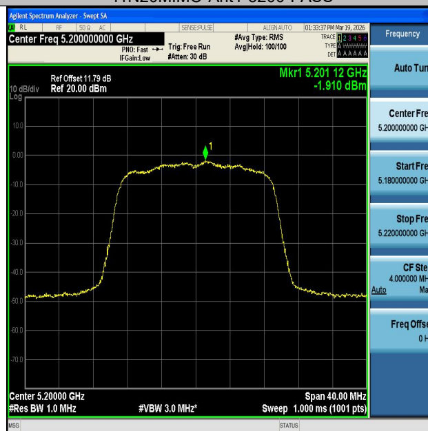
11N20MIMO-Ant2-5200-PASS
