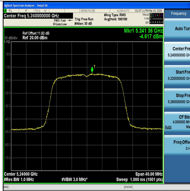
11AC20MIMO-Ant1-5240-PASS
