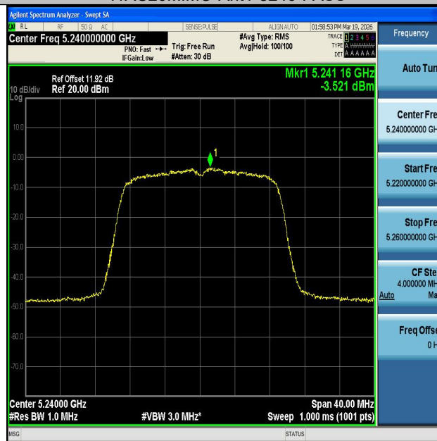
11AC20MIMO-Ant2-5240-PASS
