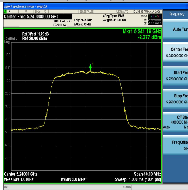
11N20MIMO-Ant2-5240-PASS
