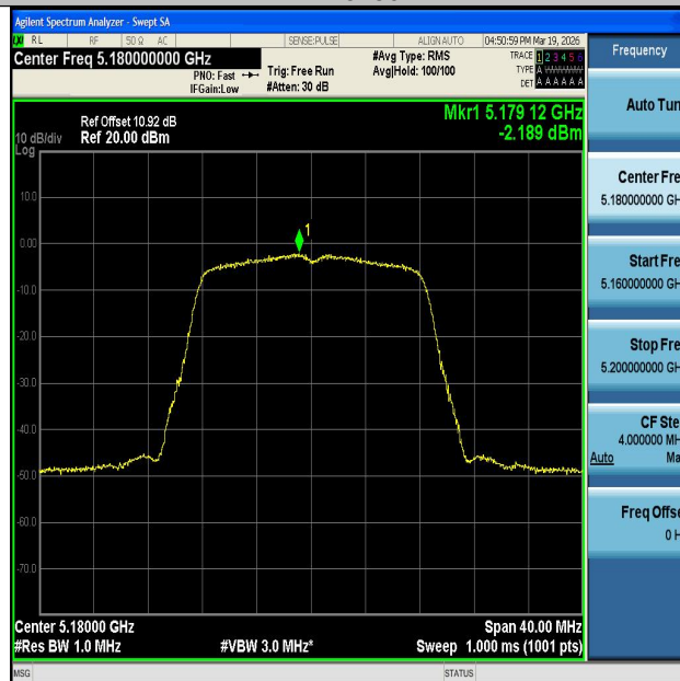
11A-Ant2-5180-PASS
