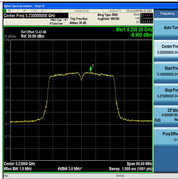
11N40MIMO-Ant1-5230-PASS
