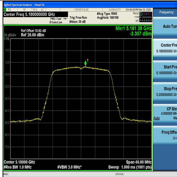
11A-Ant1-5180-PASS
