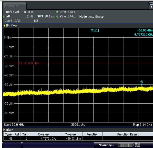
11A-Ant2-5240-30~5140-PASS
