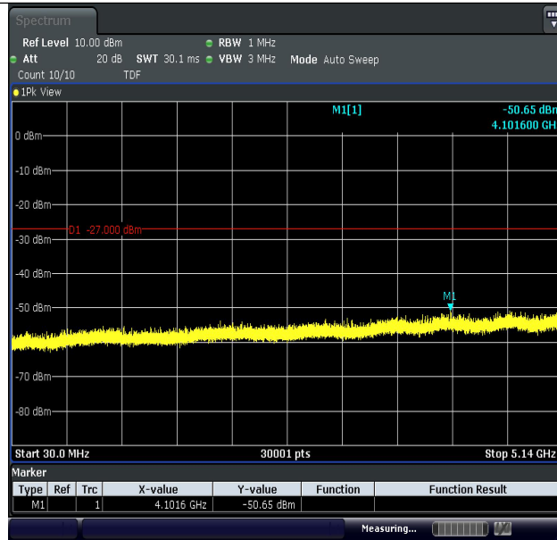
11A-Ant1-5200-30~5140-PASS
