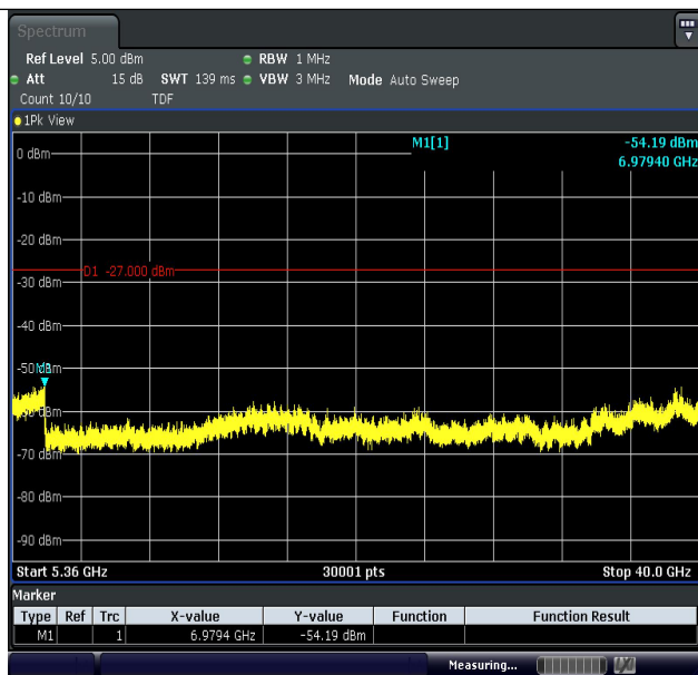
11N20MIMO-Ant1-5240-5360~40000-PASS
