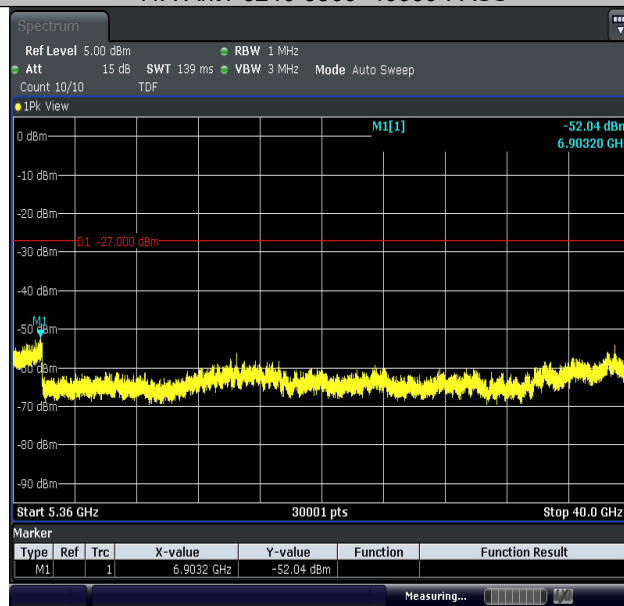
11A-Ant2-5240-5360~40000-PASS
