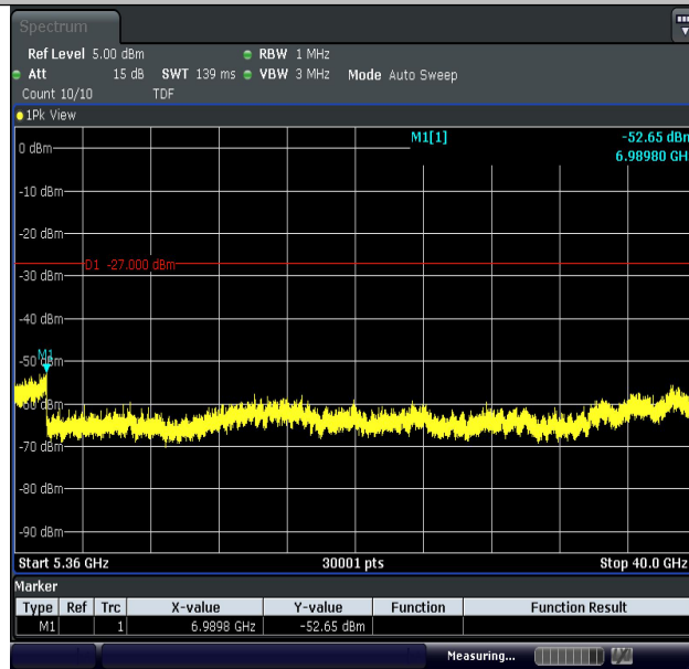
11A-Ant2-5200-5360~40000-PASS
