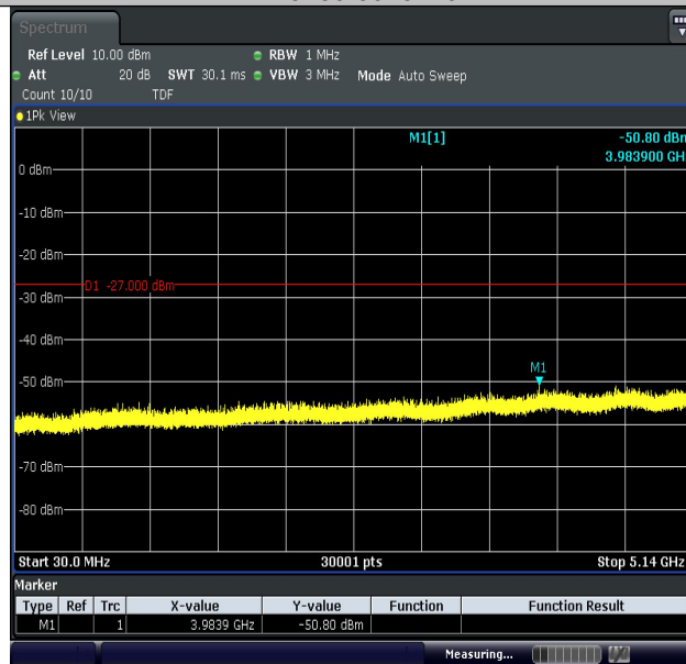
11A-Ant2-5180-30~5140-PASS
