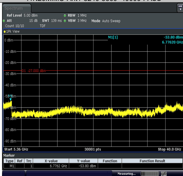
11N20MIMO-Ant2-5240-5360~40000-PASS
