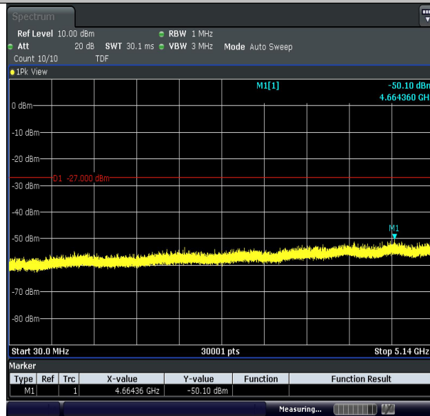
11A-Ant2-5200-30~5140-PASS
