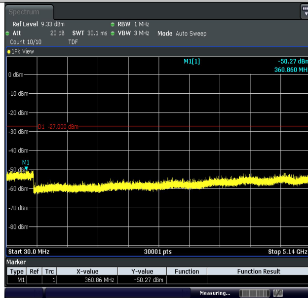
11AC20MIMO-Ant2-5240-30~5140-PASS
