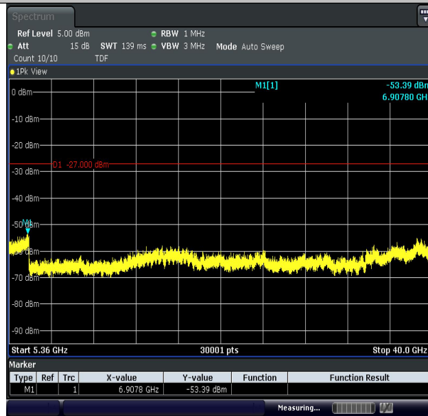
11AC20MIMO-Ant2-5180-5360~40000-PASS
