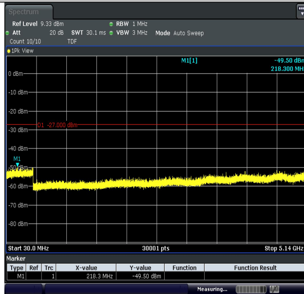
11AC40MIMO-Ant2-5230-30~5140-PASS
