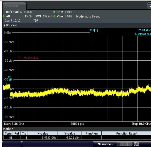
11AC40MIMO-Ant2-5190-5360~40000-PASS
