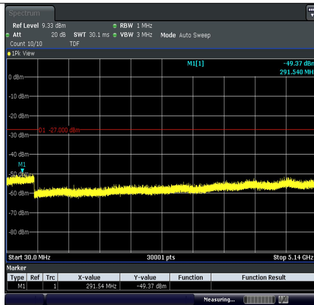
11AC20MIMO-Ant1-5200-30~5140-PASS
