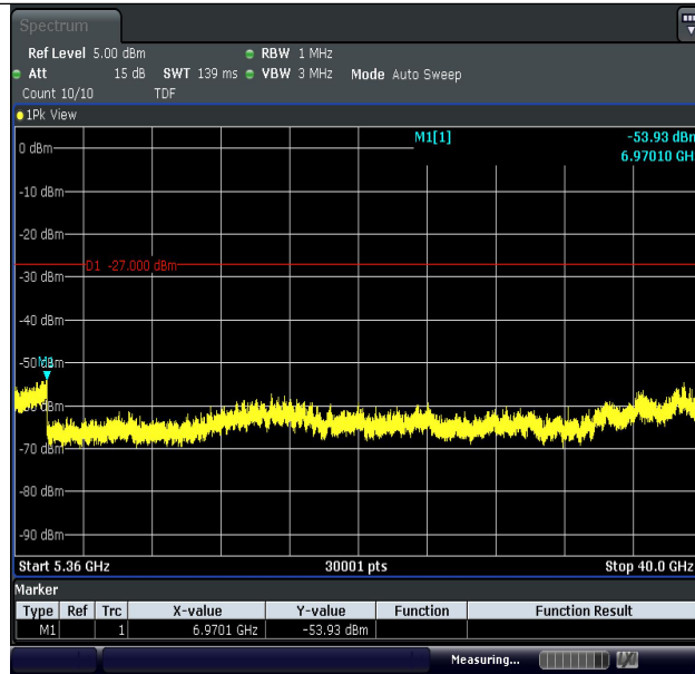
11AC40MIMO-Ant1-5190-5360~40000-PASS
