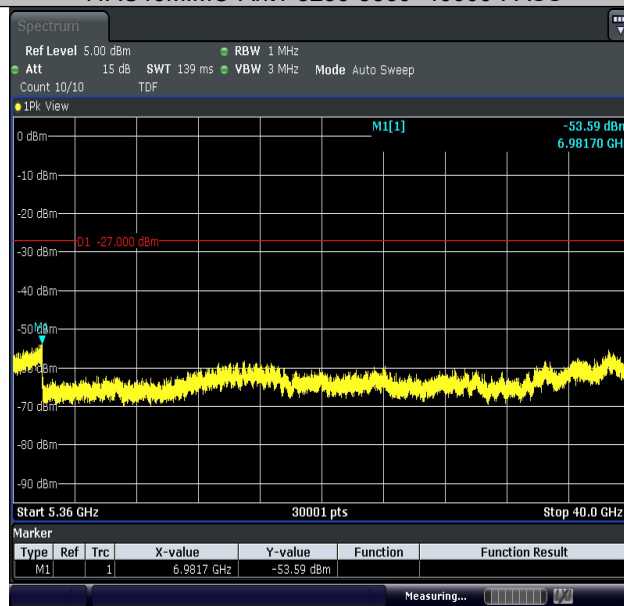
11AC40MIMO-Ant2-5230-5360~40000-PASS
