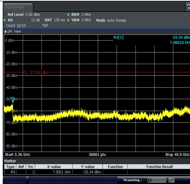
11AC40MIMO-Ant1-5230-5360~40000-PASS
