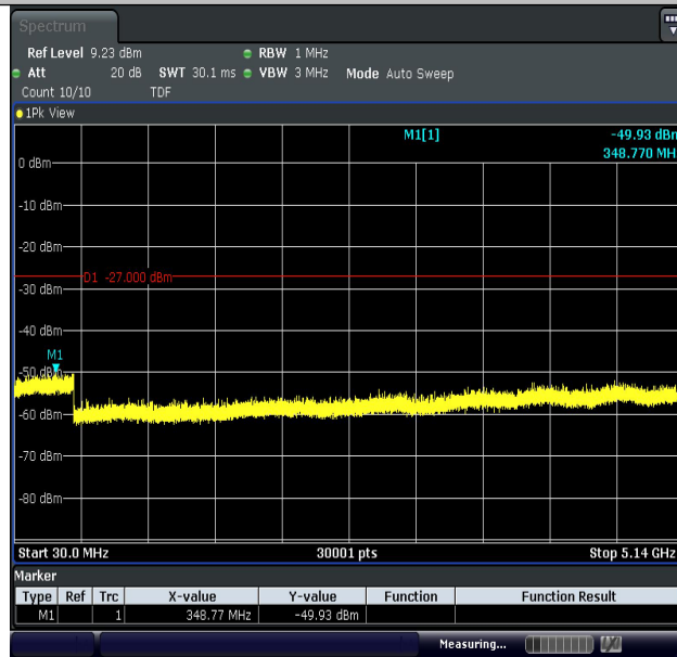
11AC20MIMO-Ant2-5180-30~5140-PASS
