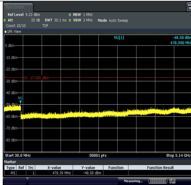
11AC20MIMO-Ant1-5180-30~5140-PASS
