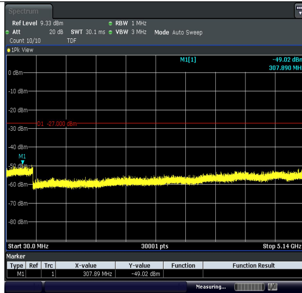
11AC40MIMO-Ant1-5230-30~5140-PASS
