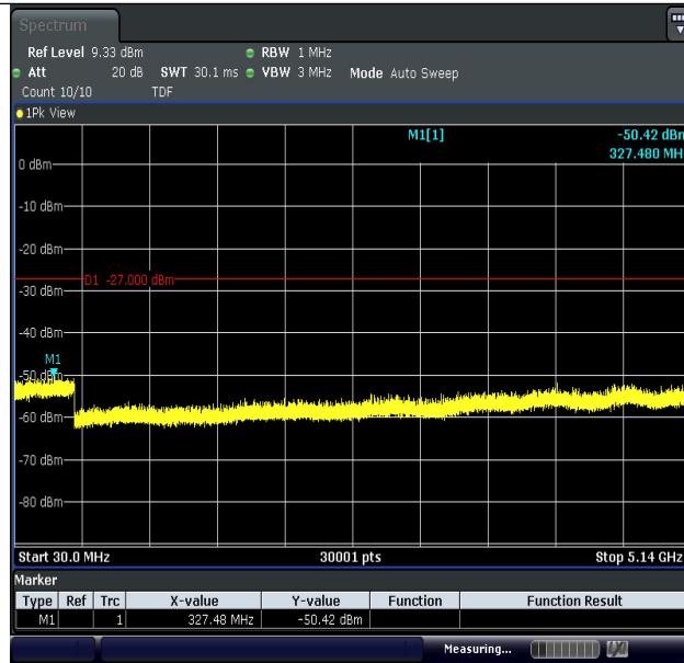
11AC20MIMO-Ant1-5240-30~5140-PASS
