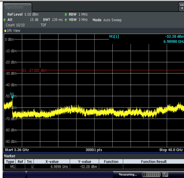
11N40MIMO-Ant2-5190-5360~40000-PASS
