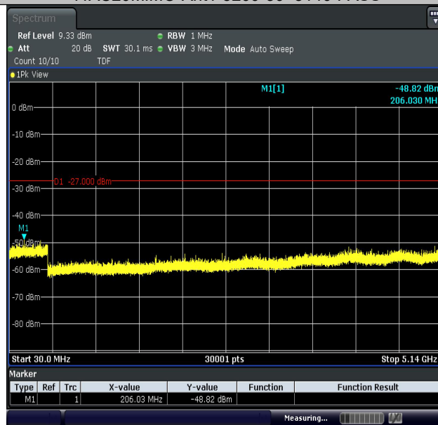
11AC20MIMO-Ant2-5200-30~5140-PASS
