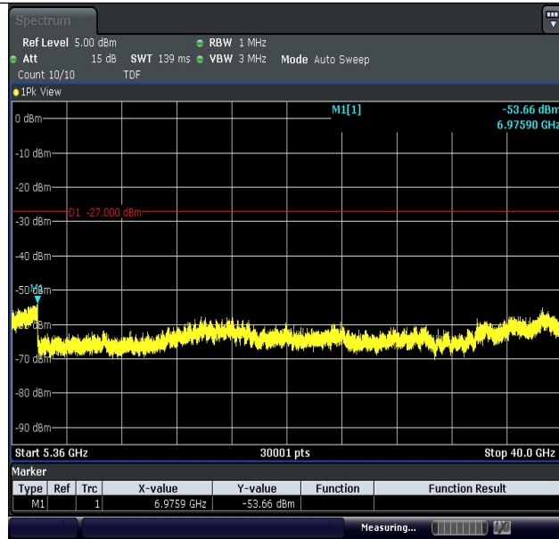
11N40MIMO-Ant1-5190-5360~40000-PASS
