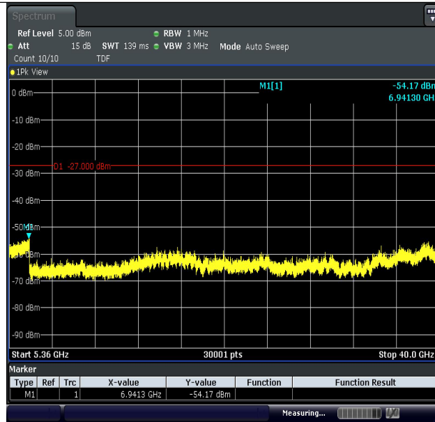
11AC20MIMO-Ant1-5180-5360~40000-PASS
