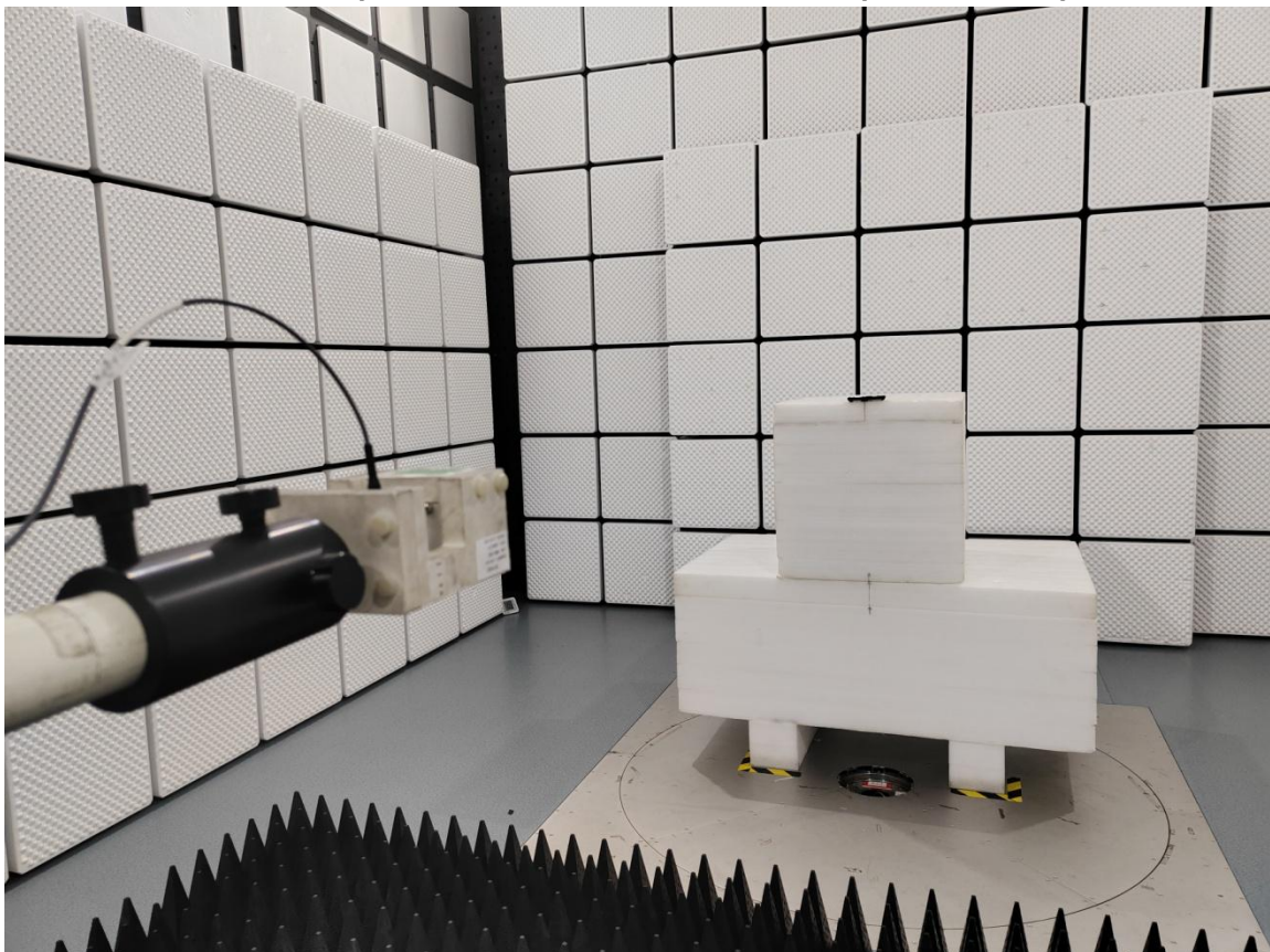
Radiated Spurious Emissions Test Front View (18GHz-25GHz)
