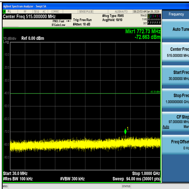
11N40MIMO-Ant1-2422-30~1000-PASS
