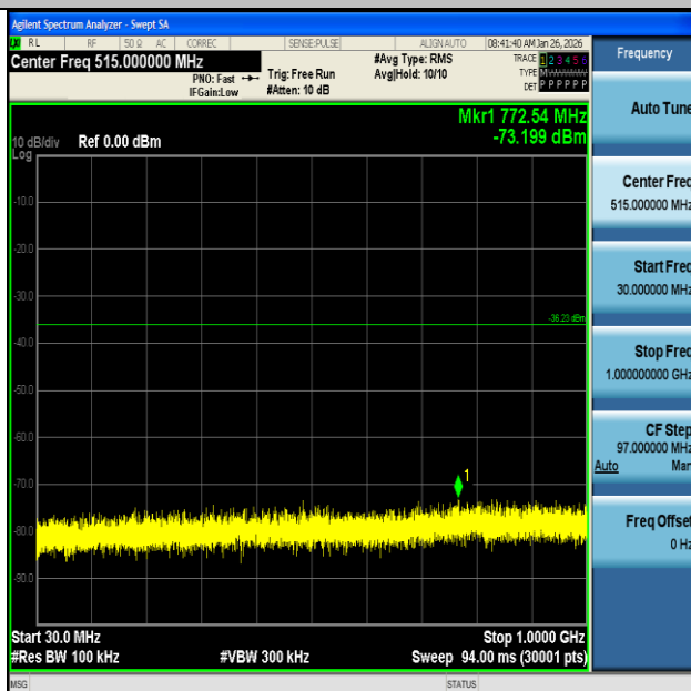
11N40MIMO-Ant2-2422-30~1000-PASS
