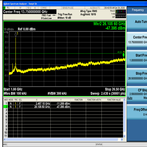
11N40MIMO-Ant1-2452-1000~26500-PASS
