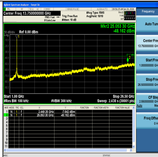
11N40MIMO-Ant2-2452-1000~26500-PASS
