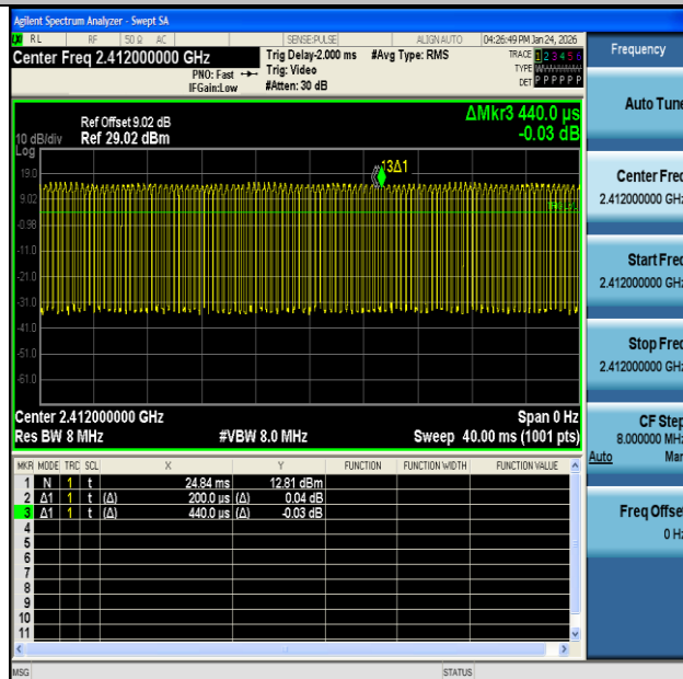
NTNV-11N20MIMO-Ant2-2412
