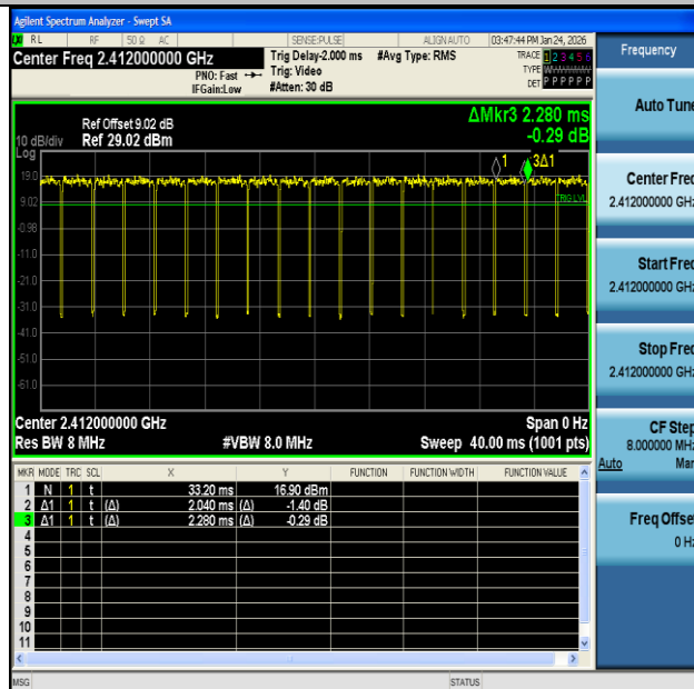
NTNV-11G-Ant2-2412
