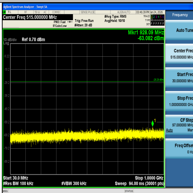
11B-Ant2-2462-30~1000-PASS
