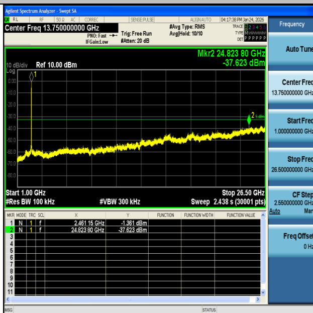
11G-Ant2-2462-1000~26500-PASS
