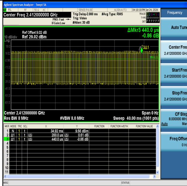
NTNV-11N20MIMO-Ant1-2412
