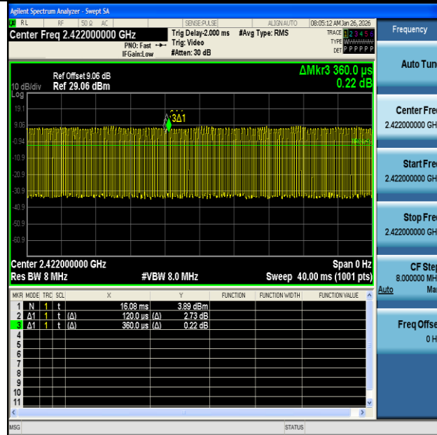
NTNV-11N40MIMO-Ant1-2422
