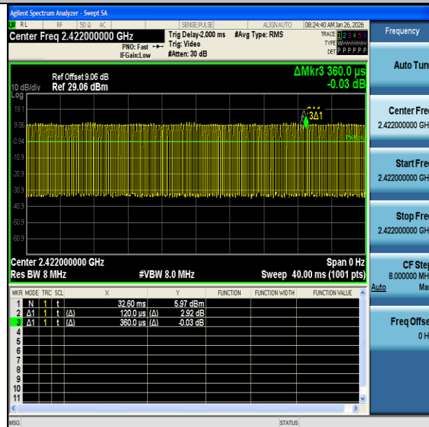
NTNV-11N40MIMO-Ant2-2422
