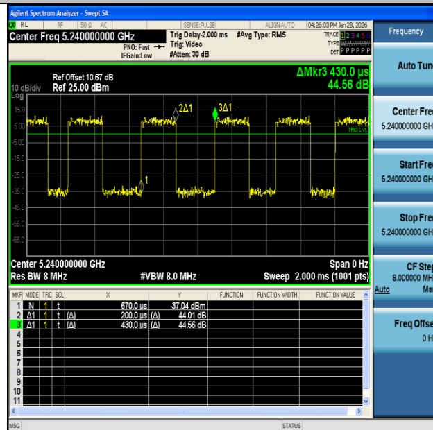
NTNV-11AC20MIMO-Ant2-5240
