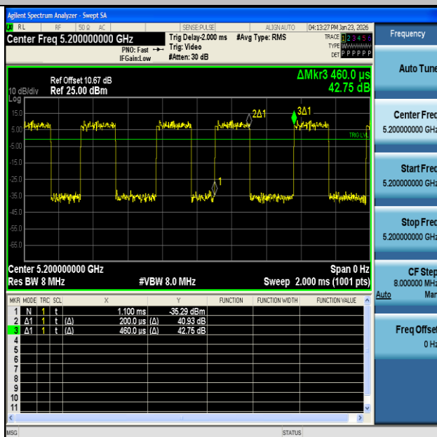
NTNV-11AC20MIMO-Ant2-5200
