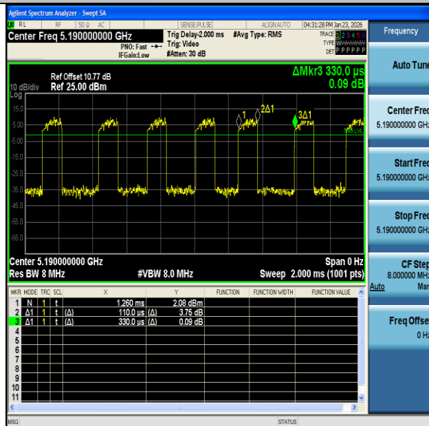
NTNV-11AC40MIMO-Ant2-5190
