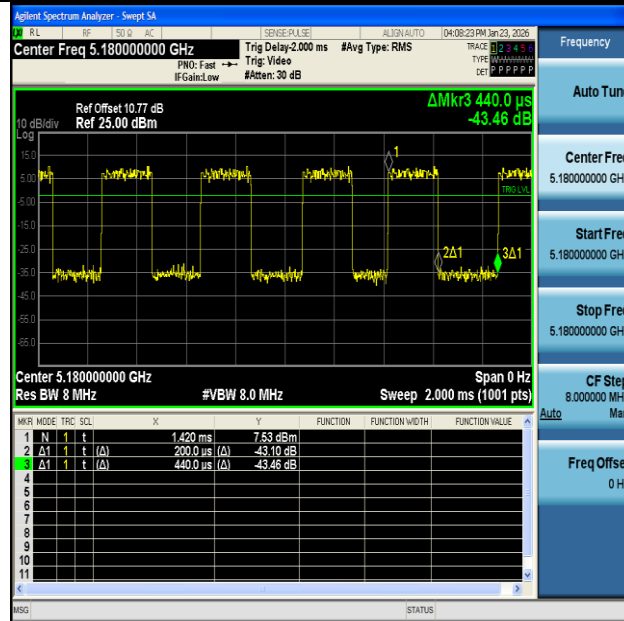
NTNV-11AC20MIMO-Ant1-5180
