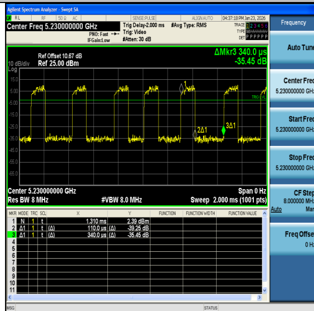
NTNV-11AC40MIMO-Ant2-5230
