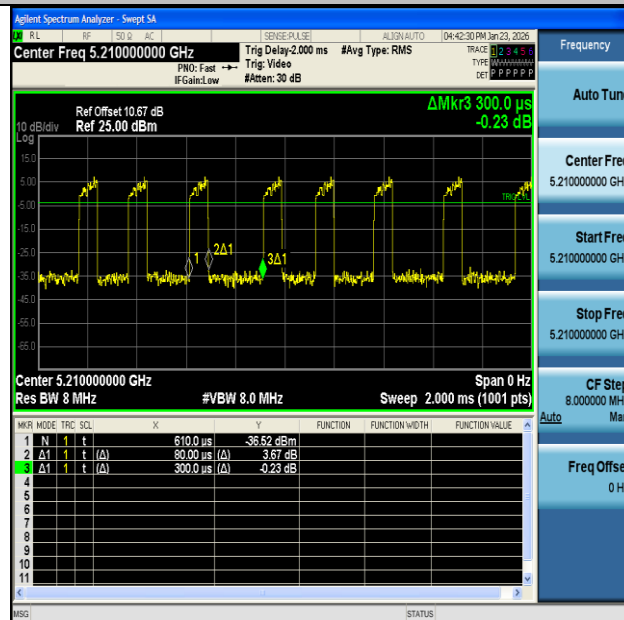
NTNV-11AC80MIMO-Ant2-5210
