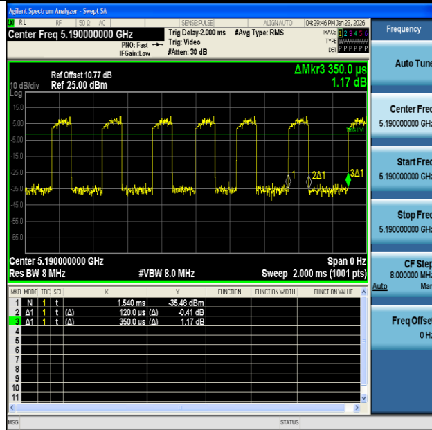
NTNV-11AC40MIMO-Ant1-5190
