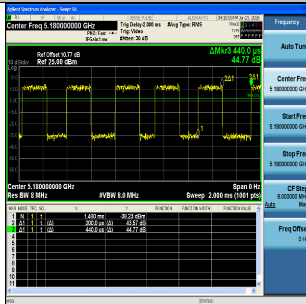
NTNV-11AC20MIMO-Ant2-5180
