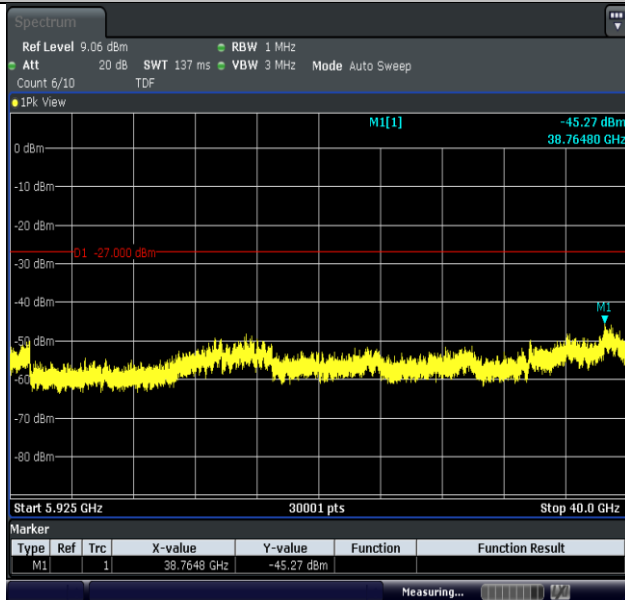
11AC20MIMO-Ant2-5745-5925~40000-PASS
