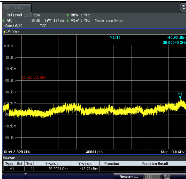
11N20MIMO-Ant1-5825-5925~40000-PASS
