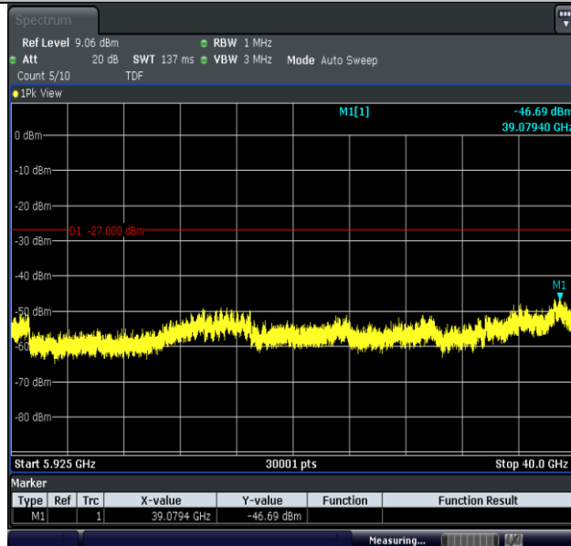
11N40MIMO-Ant2-5755-5925~40000-PASS
