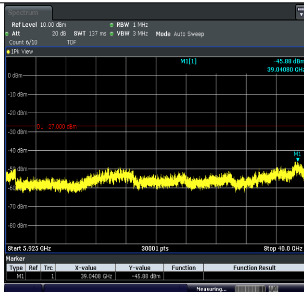
11N40MIMO-Ant1-5755-5925~40000-PASS
