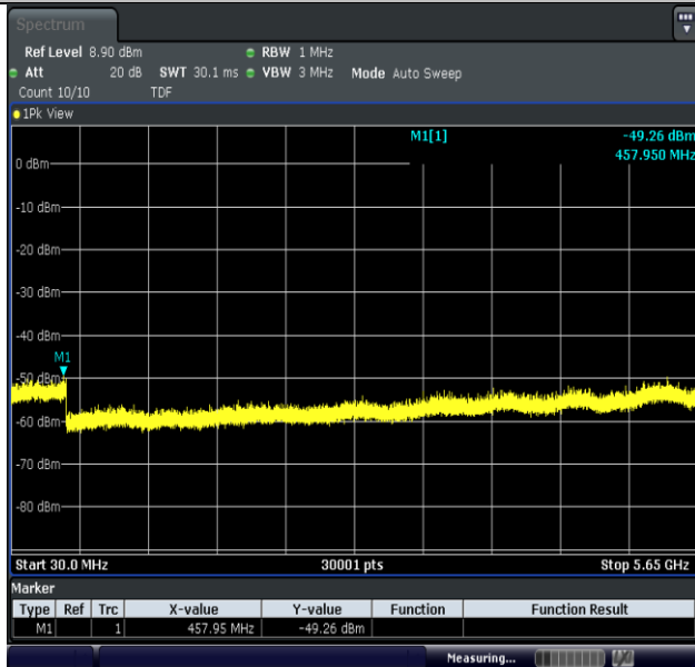
11N20MIMO-Ant2-5825-30~5650-PASS
