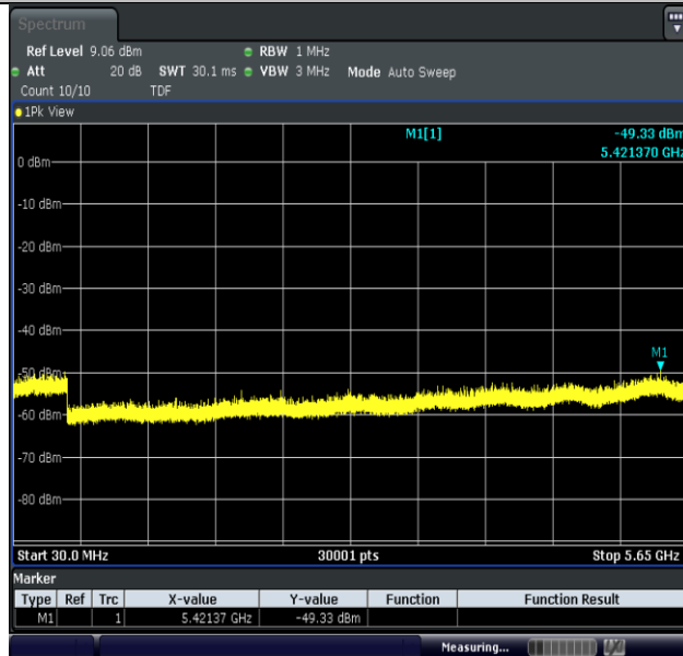
11AC40MIMO-Ant2-5755-30~5650-PASS
