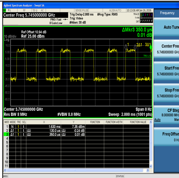
NTNV-11N20MIMO-Ant2-5745
