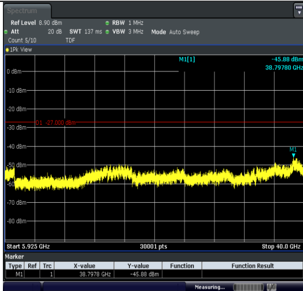
11N20MIMO-Ant2-5825-5925~40000-PASS
