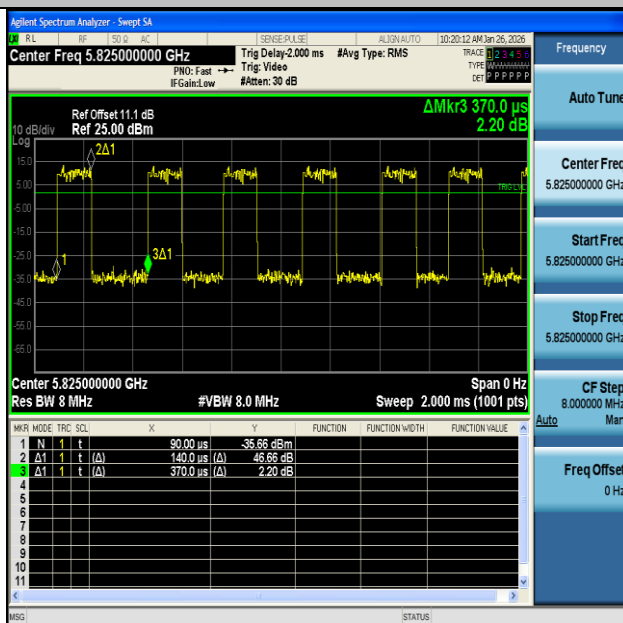
NTNV-11N20MIMO-Ant2-5825
