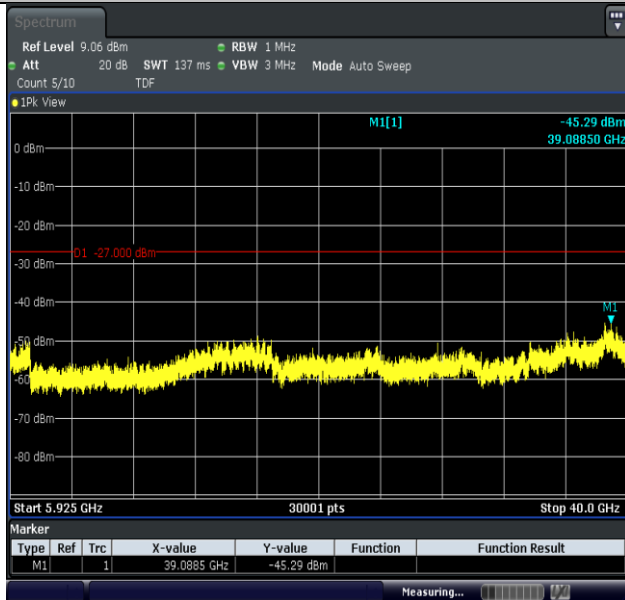
11AC80MIMO-Ant2-5775-5925~40000-PASS
