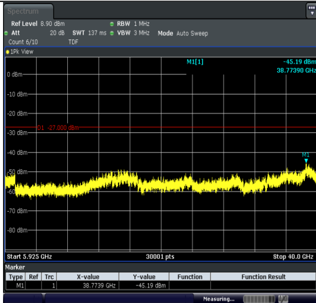
11AC20MIMO-Ant2-5825-5925~40000-PASS
