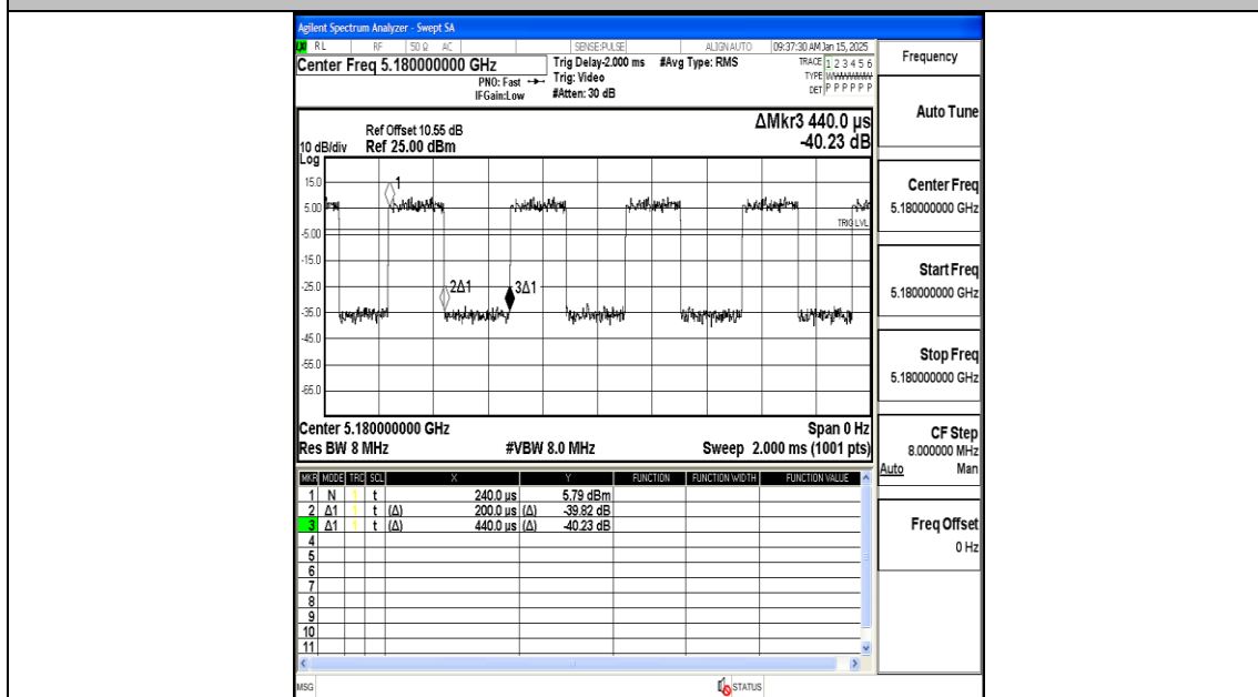
NTNV-11AC20MIMO-Ant1-5180
