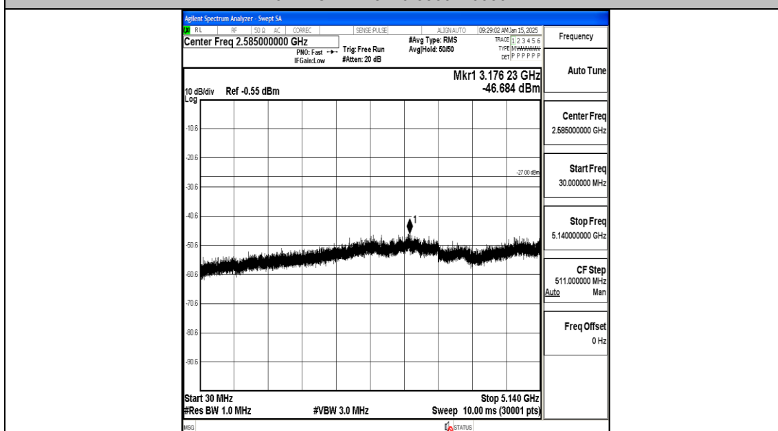
11N40MIMO-Ant1-5190-30~5140-PASS
