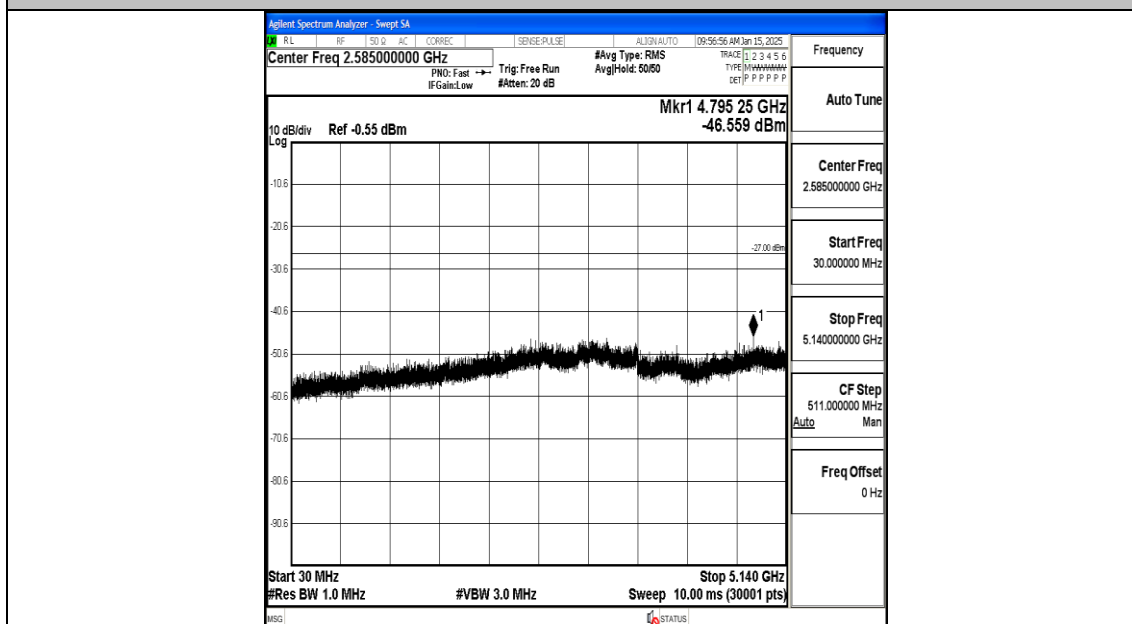
11AC40MIMO-Ant1-5230-30~5140-PASS
