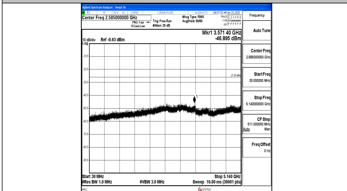
11A-Ant2-5240-30~5140-PASS
