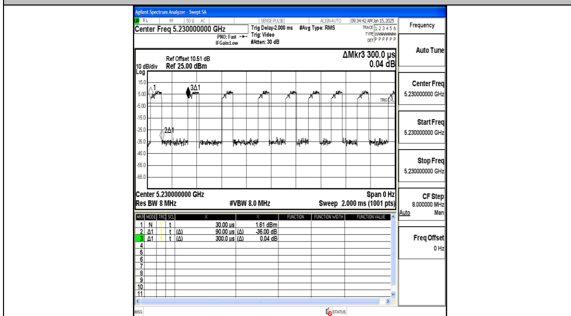
NTNV-11N40MIMO-Ant2-5230
