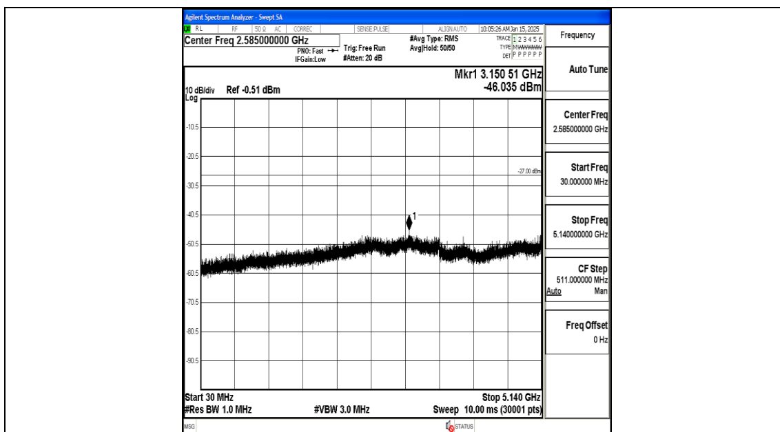
11AC80MIMO-Ant2-5210-30~5140-PASS
