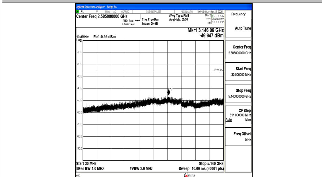
11AC20MIMO-Ant1-5200-30~5140-PASS
