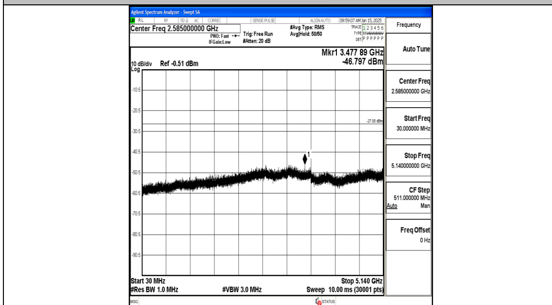
11AC40MIMO-Ant2-5230-30~5140-PASS
