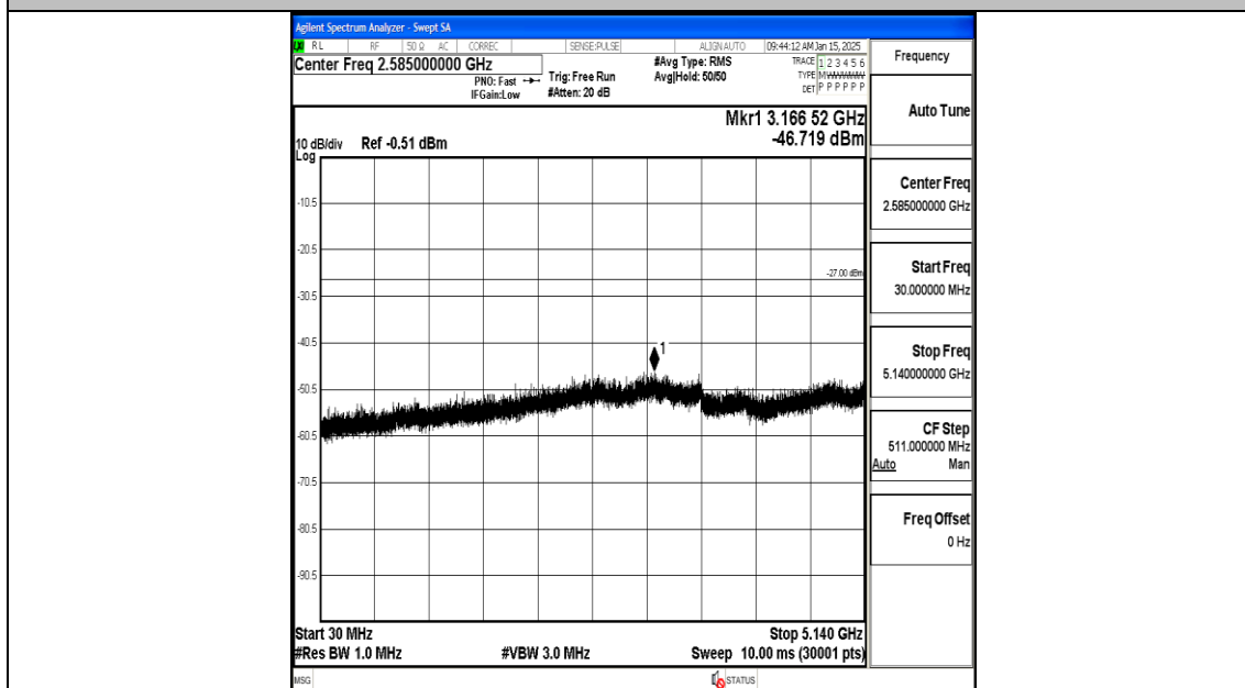
11AC20MIMO-Ant2-5200-30~5140-PASS
