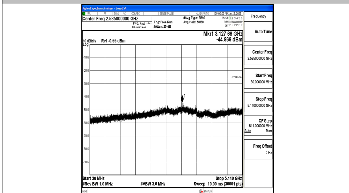
11N20MIMO-Ant1-5180-30~5140-PASS
