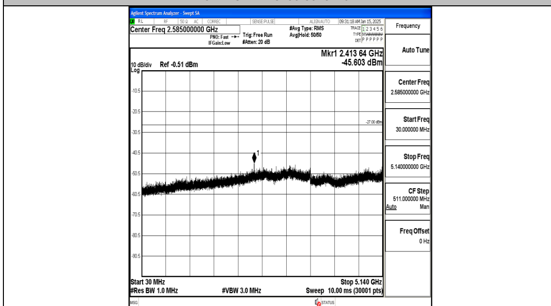
11N40MIMO-Ant2-5190-30~5140-PASS
