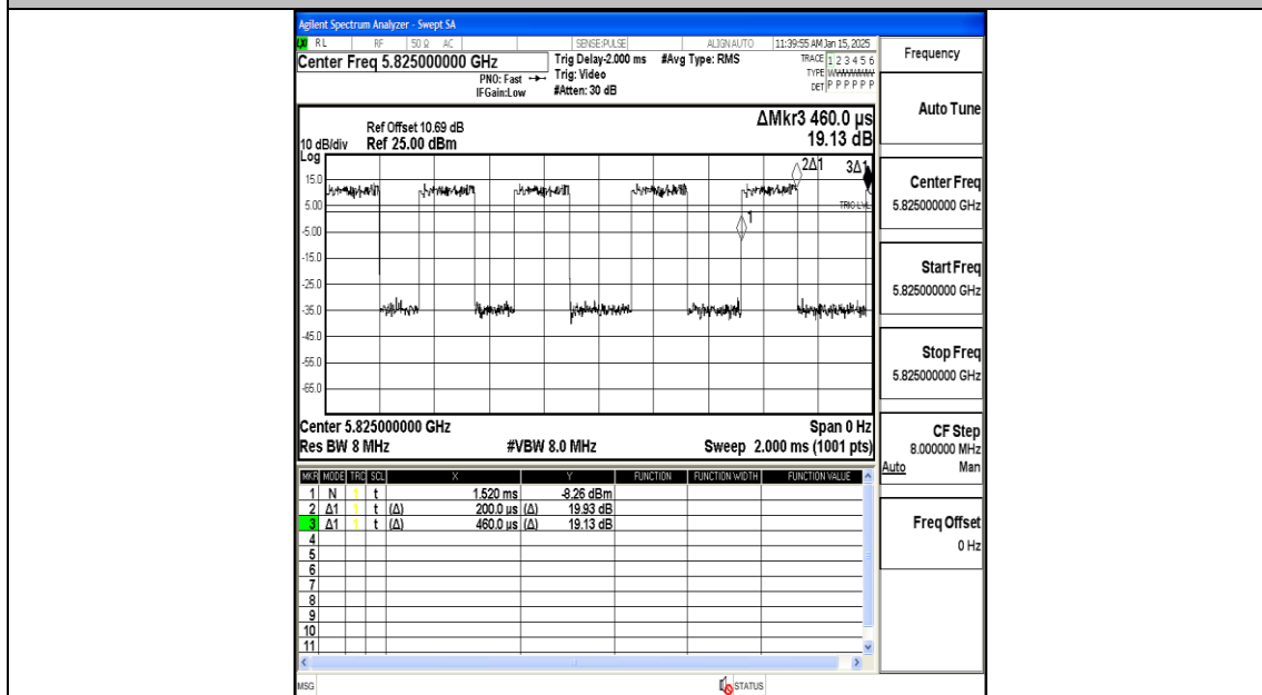
NTNV-11AC20MIMO-Ant2-5825
