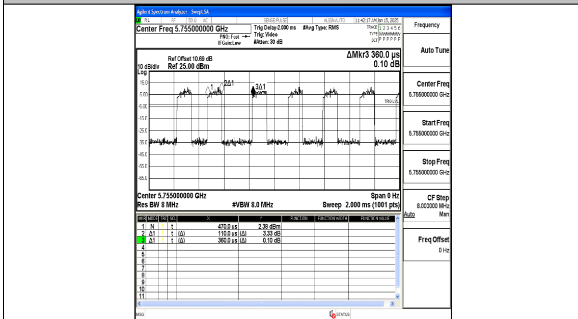
NTNV-11AC40MIMO-Ant1-5755
