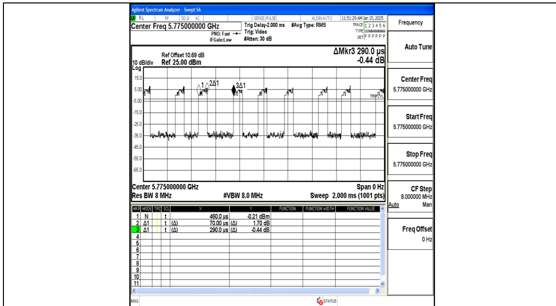
NTNV-11AC80MIMO-Ant1-5775
