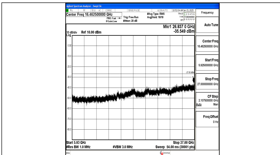
11A-Ant1-5745-5925~40000-PASS
