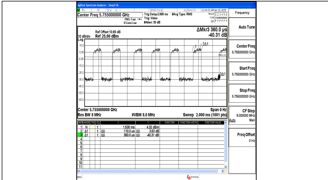
NTNV-11AC40MIMO-Ant2-5755
