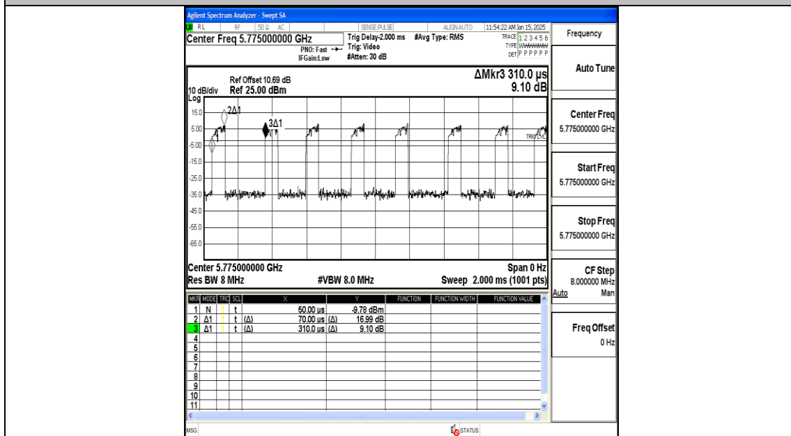
NTNV-11AC80MIMO-Ant2-5775
