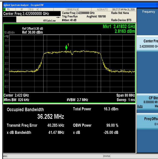
11N40MIMO-Ant2-2422
