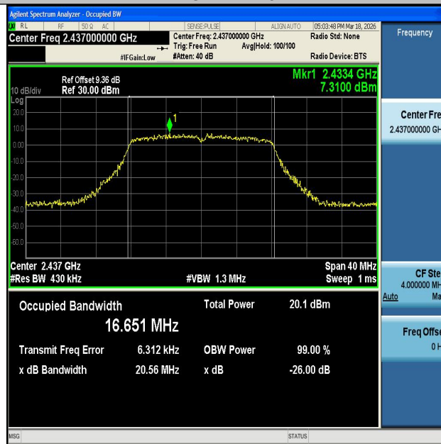
11G-Ant2-2437
