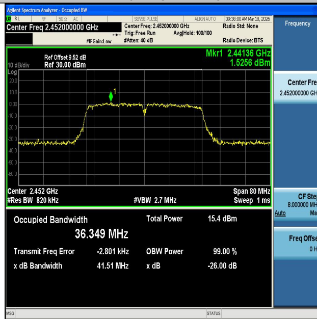
11N40MIMO-Ant2-2452
