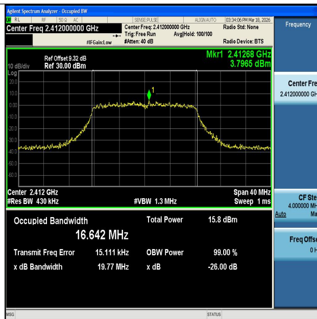
11G-Ant1-2412
