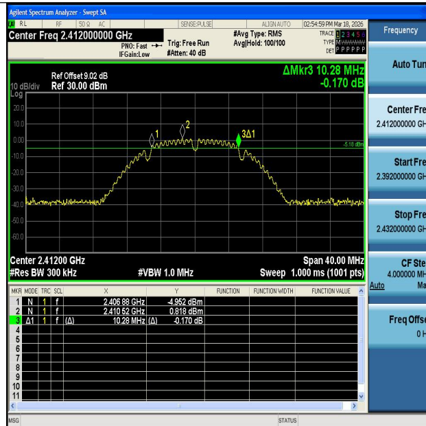
11B-Ant1-2412-PASS
