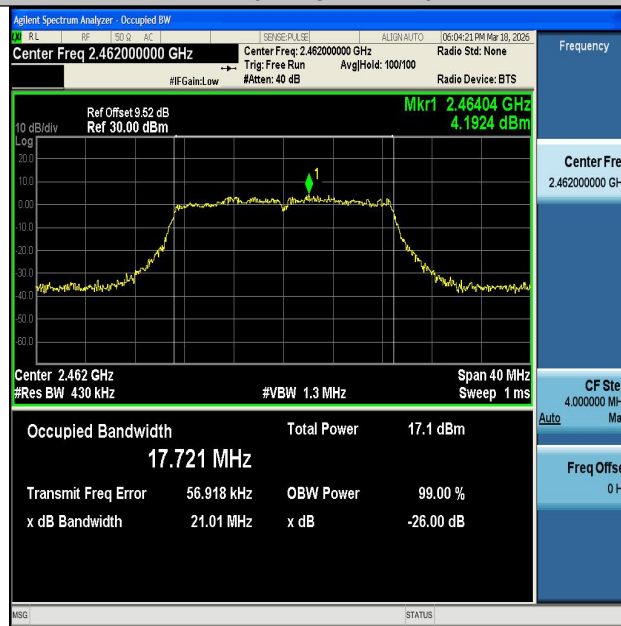
11N20MIMO-Ant2-2462
