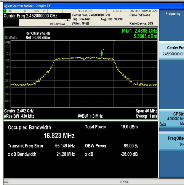
11G-Ant2-2462
