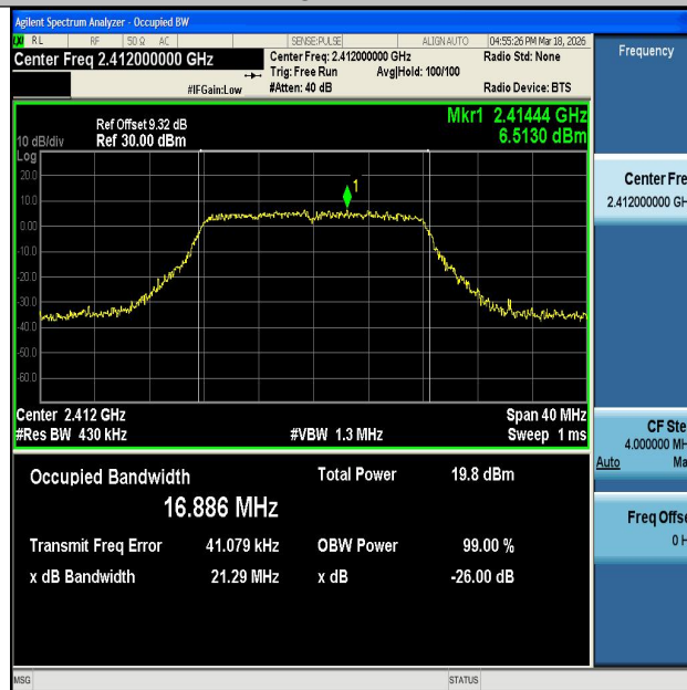
11G-Ant2-2412
