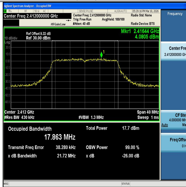
11N20MIMO-Ant2-2412
