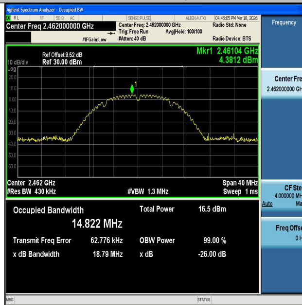
11B-Ant2-2462
