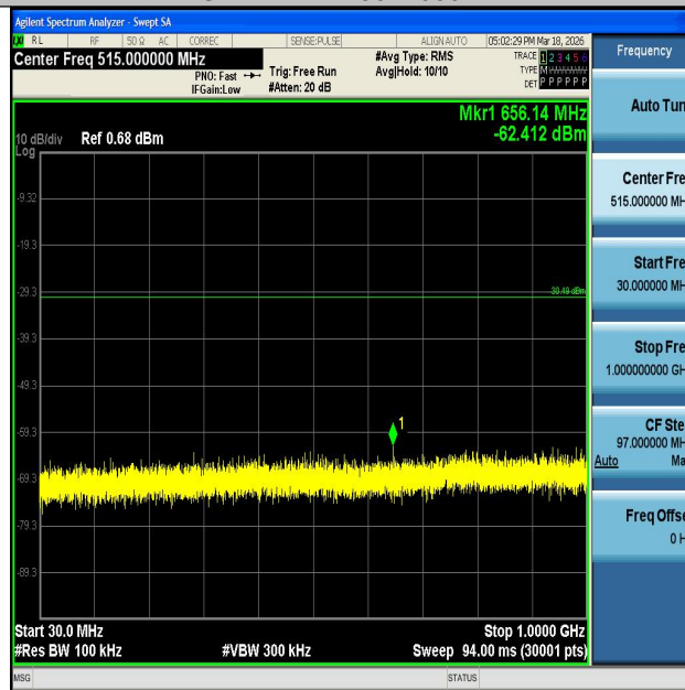
11G-Ant2-2412-30~1000-PASS
