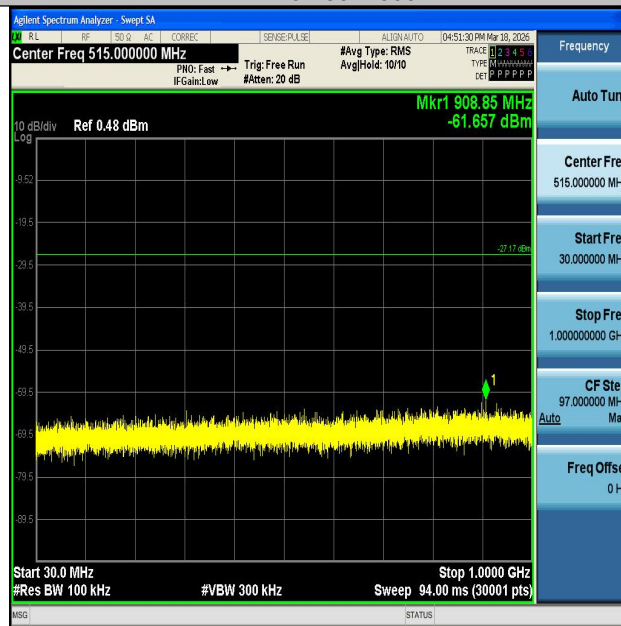
11B-Ant2-2462-30~1000-PASS
