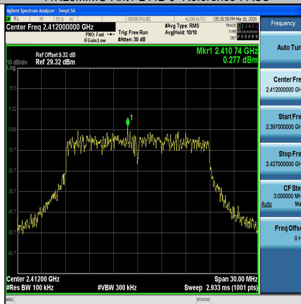
11N20MIMO-Ant2-2412-0~Reference-PASS
