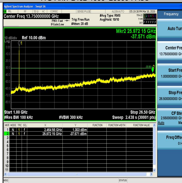
11G-Ant2-2462-1000~26500-PASS
