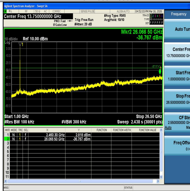
11B-Ant2-2462-1000~26500-PASS
