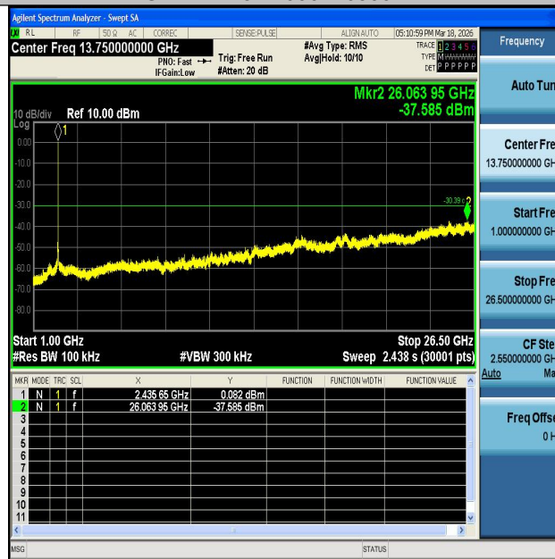
11G-Ant2-2437-1000~26500-PASS
