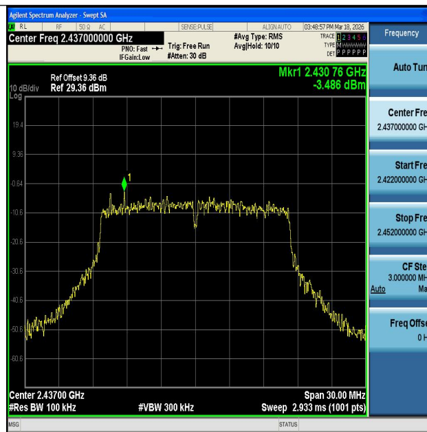
11G-Ant1-2437-0~Reference-PASS
