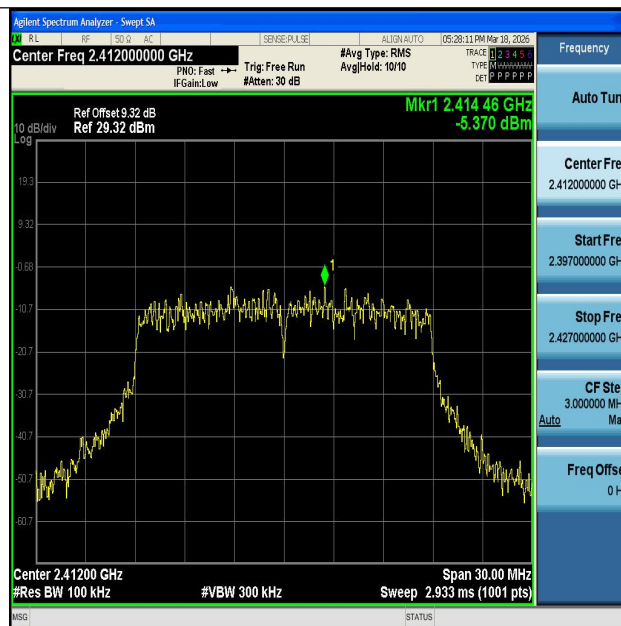
11N20MIMO-Ant1-2412-0~Reference-PASS
