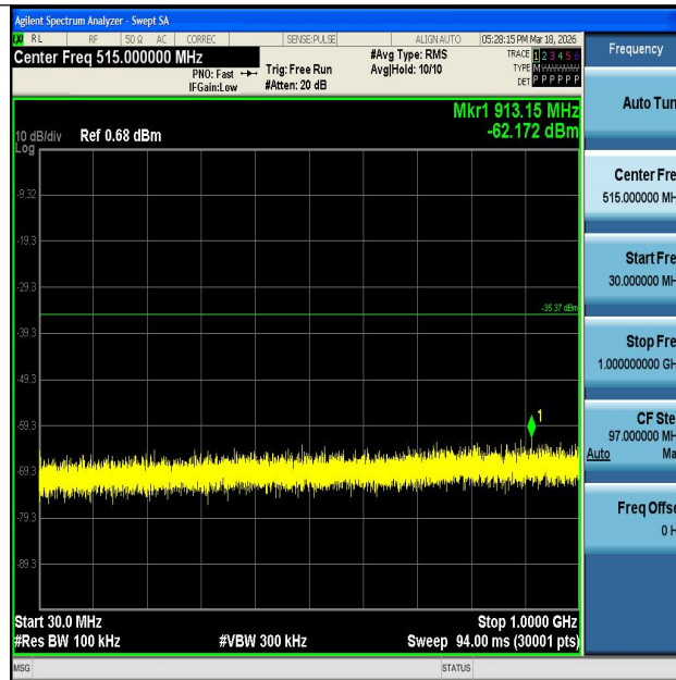
11N20MIMO-Ant1-2412-30~1000-PASS
