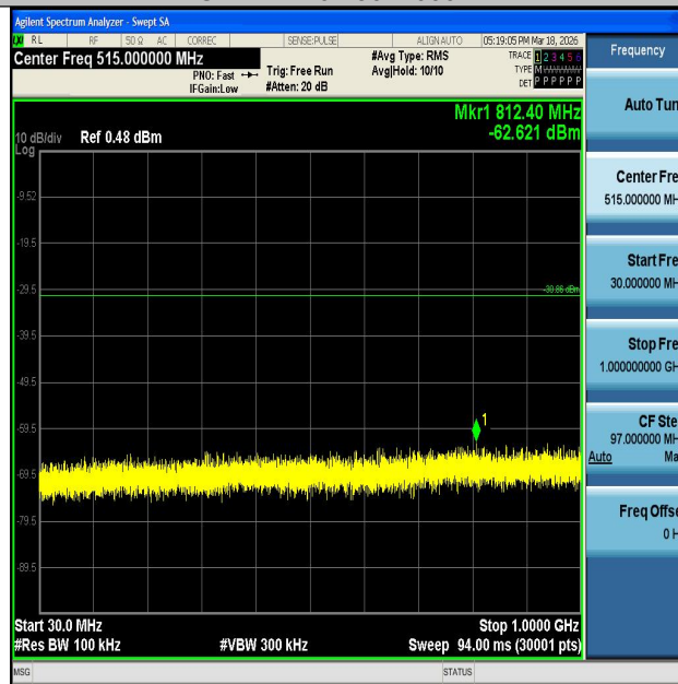
11G-Ant2-2462-30~1000-PASS
