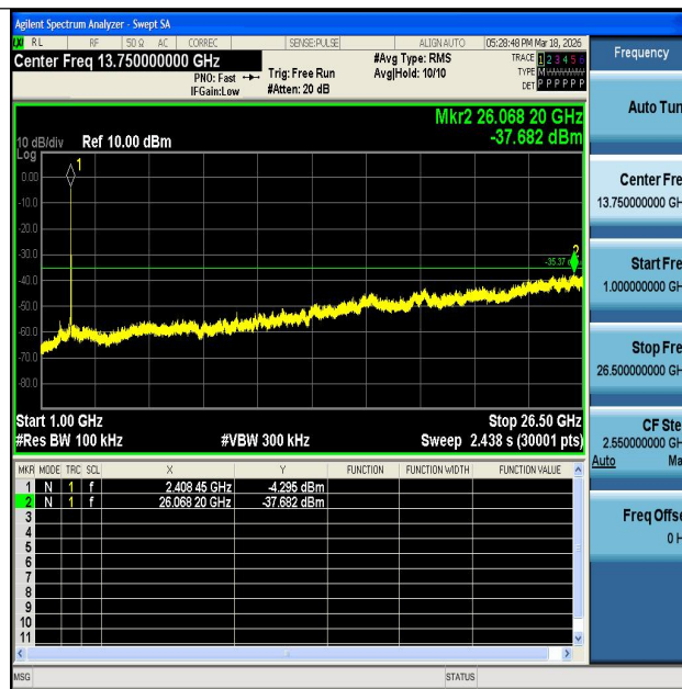
11N20MIMO-Ant1-2412-1000~26500-PASS
