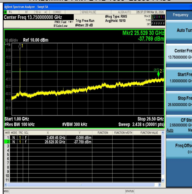
11N20MIMO-Ant2-2412-1000~26500-PASS
