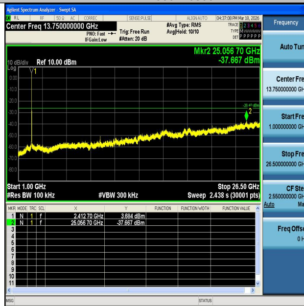
11B-Ant2-2412-1000~26500-PASS
