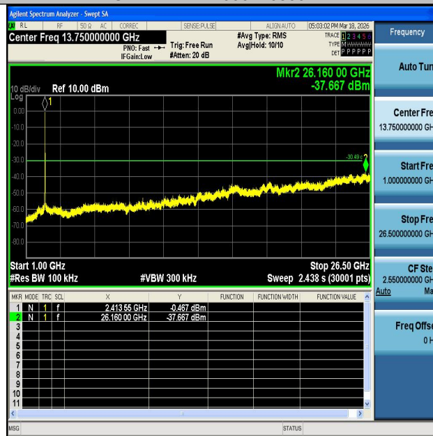
11G-Ant2-2412-1000~26500-PASS
