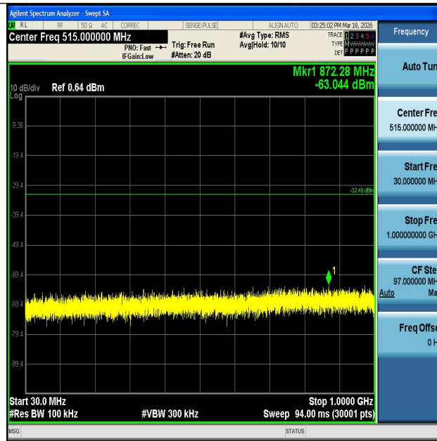
11B-Ant1-2437-30~1000-PASS
