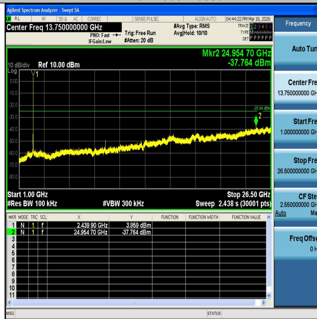
11B-Ant2-2437-1000~26500-PASS
