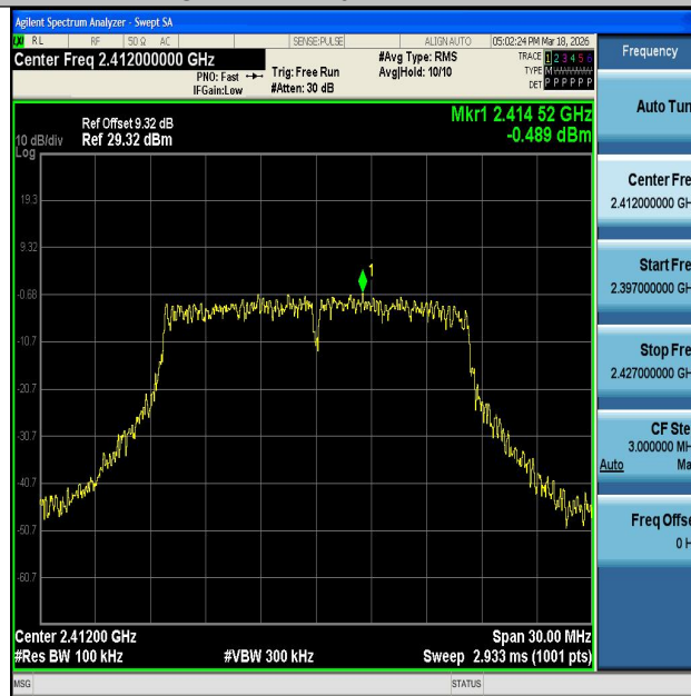
11G-Ant2-2412-0~Reference-PASS
