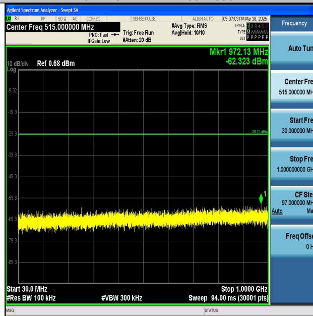
11N20MIMO-Ant2-2412-30~1000-PASS
