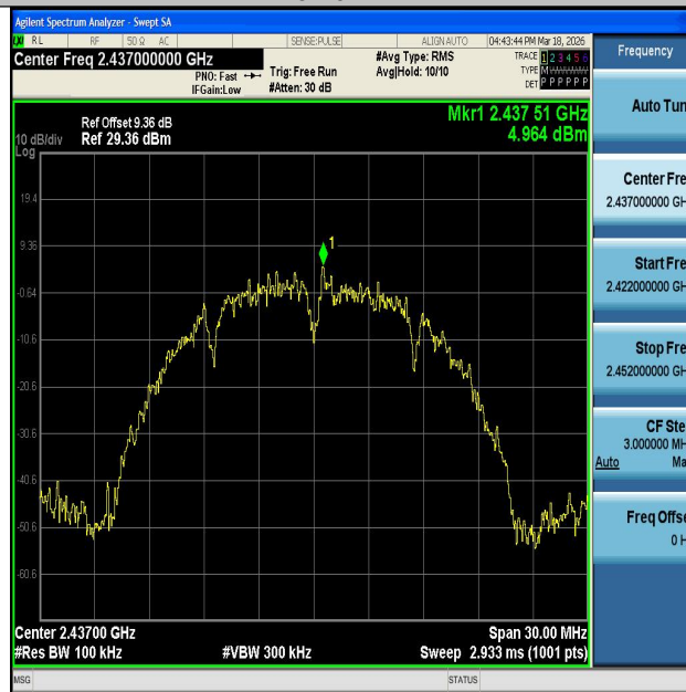
11B-Ant2-2437-0~Reference-PASS
