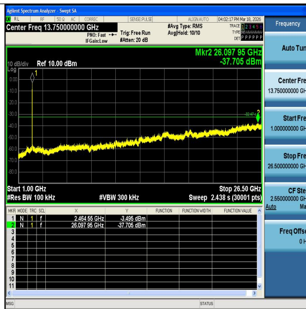
11G-Ant1-2462-1000~26500-PASS
