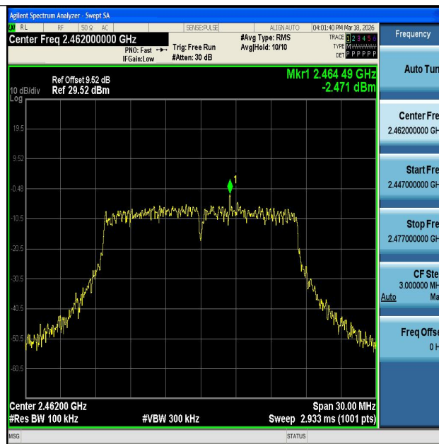
11G-Ant1-2462-0~Reference-PASS
