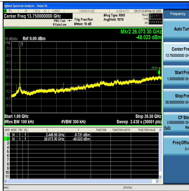
11N40MIMO-Ant1-2452-1000~26500-PASS
