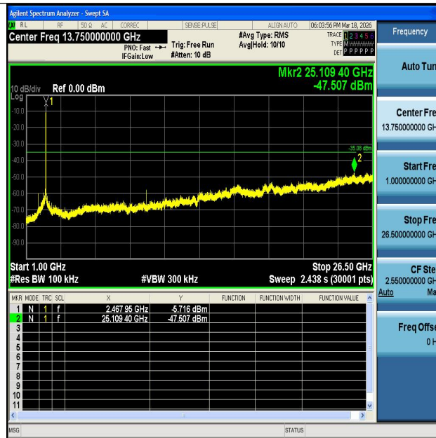
11N20MIMO-Ant1-2462-1000~26500-PASS
