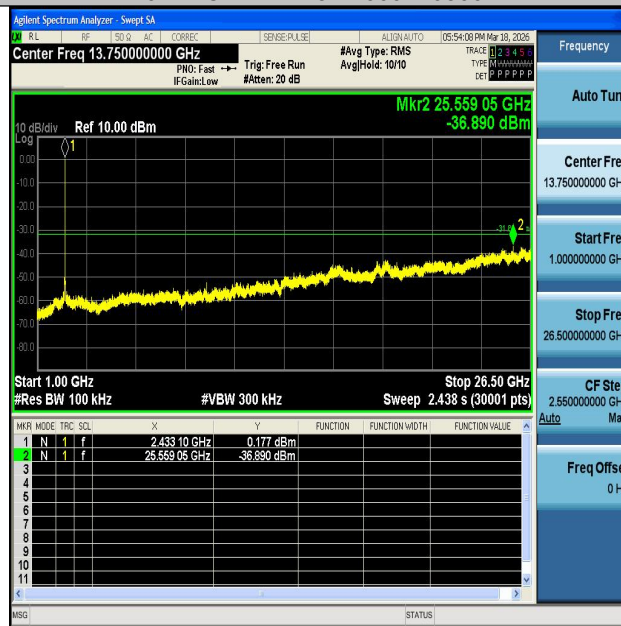
11N20MIMO-Ant2-2437-1000~26500-PASS
