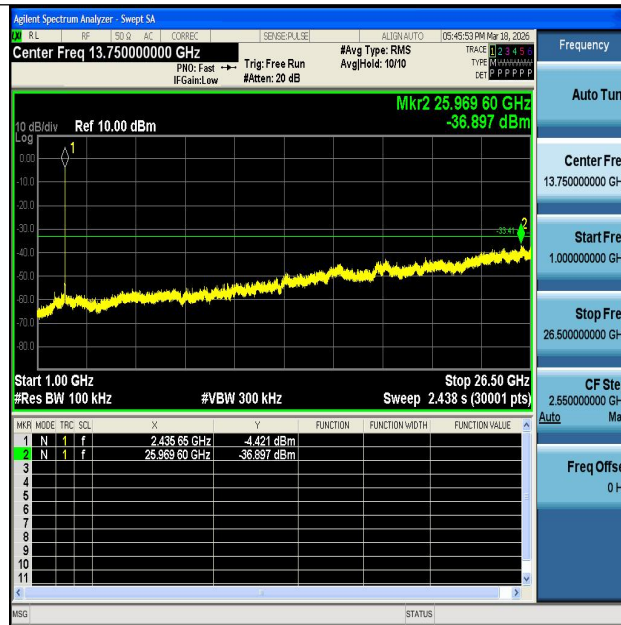
11N20MIMO-Ant1-2437-1000~26500-PASS
