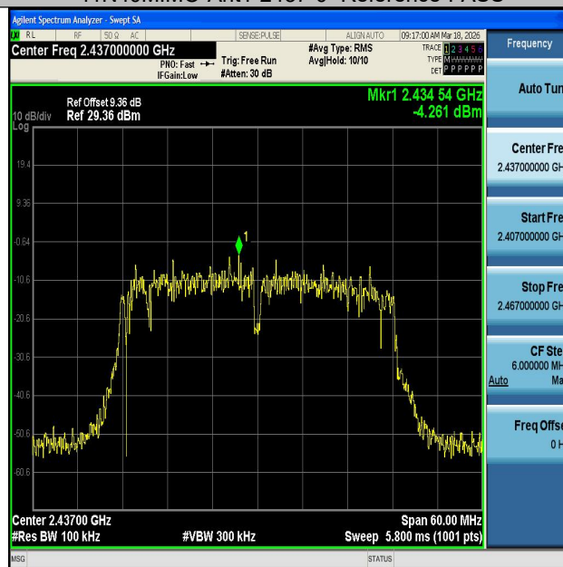
11N40MIMO-Ant2-2437-0~Reference-PASS
