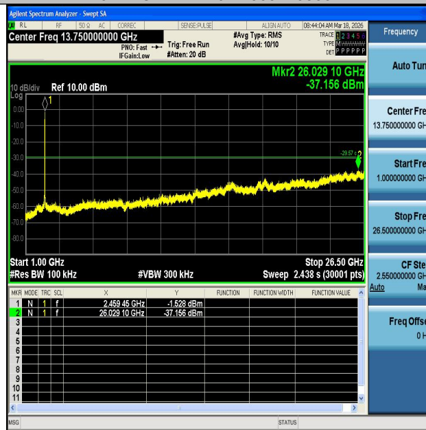
11N20MIMO-Ant2-2462-1000~26500-PASS
