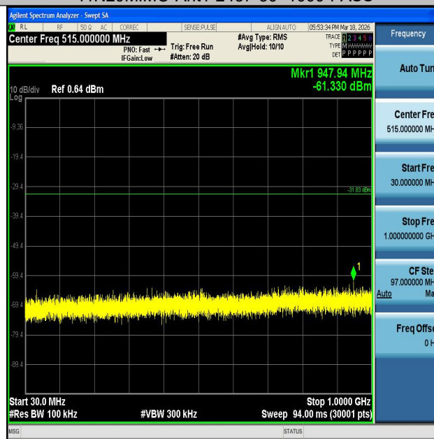
11N20MIMO-Ant2-2437-30~1000-PASS
