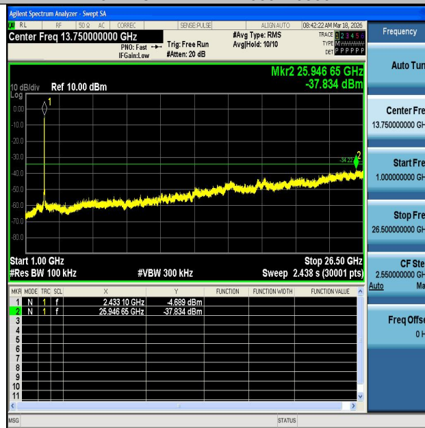
11N40MIMO-Ant2-2422-1000~26500-PASS
