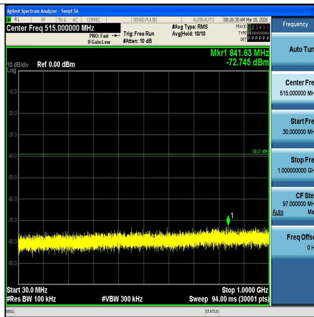
11N40MIMO-Ant1-2422-30~1000-PASS
