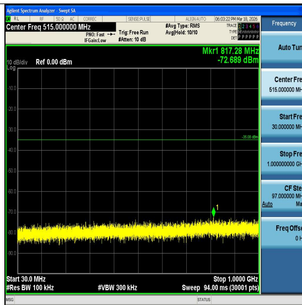
11N20MIMO-Ant1-2462-30~1000-PASS
