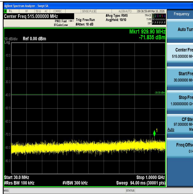
11N40MIMO-Ant1-2452-30~1000-PASS
