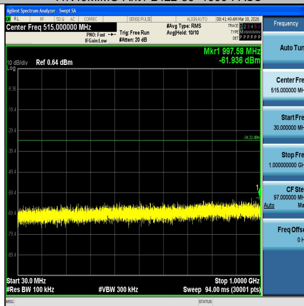
11N40MIMO-Ant2-2422-30~1000-PASS
