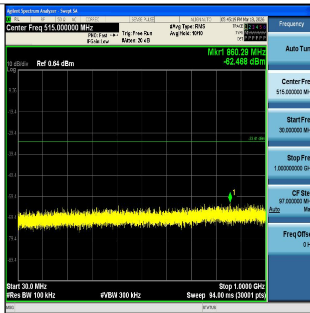
11N20MIMO-Ant1-2437-30~1000-PASS
