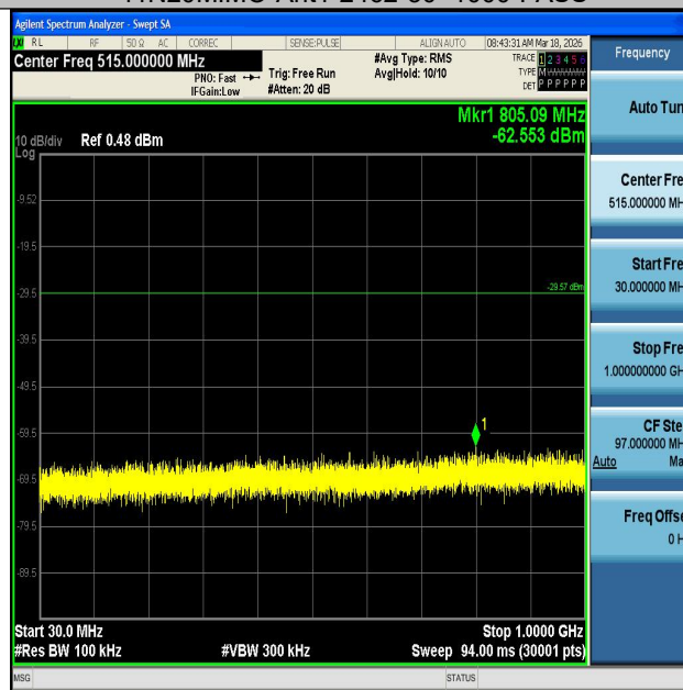
11N20MIMO-Ant2-2462-30~1000-PASS
