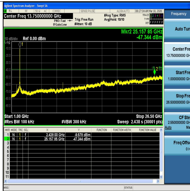
11N40MIMO-Ant1-2422-1000~26500-PASS
