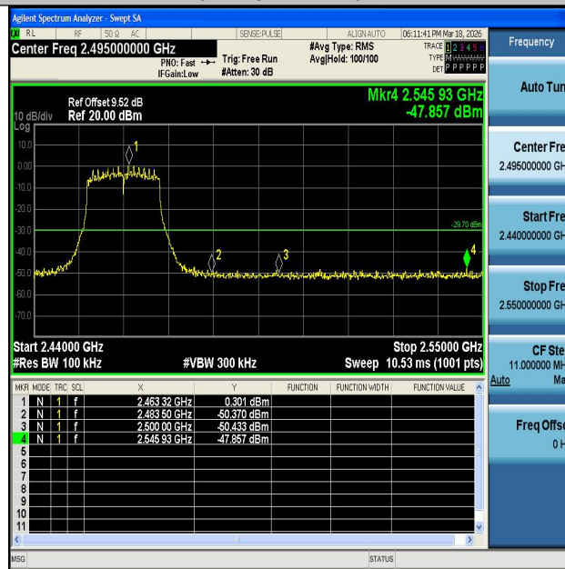
11N20MIMO-Ant2-2462-PASS
