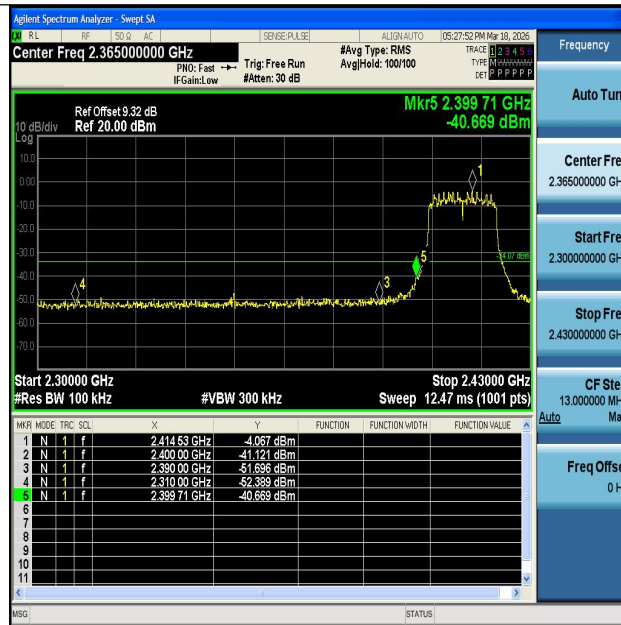
11N20MIMO-Ant1-2412-PASS
