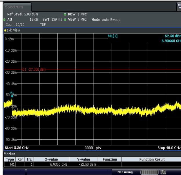
11AC80MIMO-Ant2-5210-5360~40000-PASS
