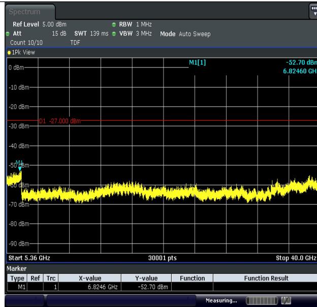
11AC80MIMO-Ant1-5210-5360~40000-PASS
