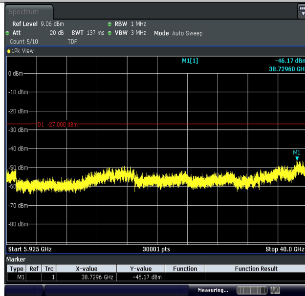
11A-Ant2-5745-5925~40000-PASS
