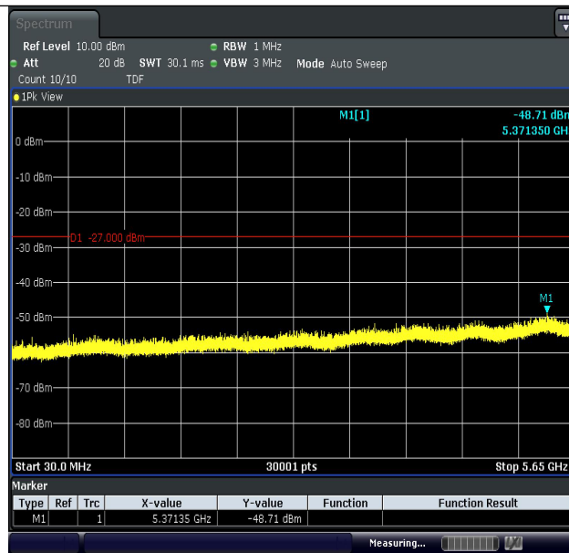
11N40MIMO-Ant1-5755-30~5650-PASS
