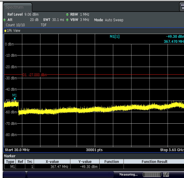
11N40MIMO-Ant2-5795-30~5650-PASS
