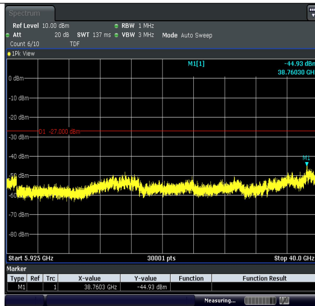
11N40MIMO-Ant1-5755-5925~40000-PASS
