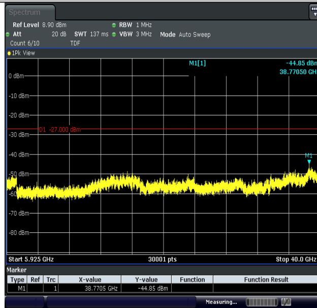
11A-Ant2-5825-5925~40000-PASS
