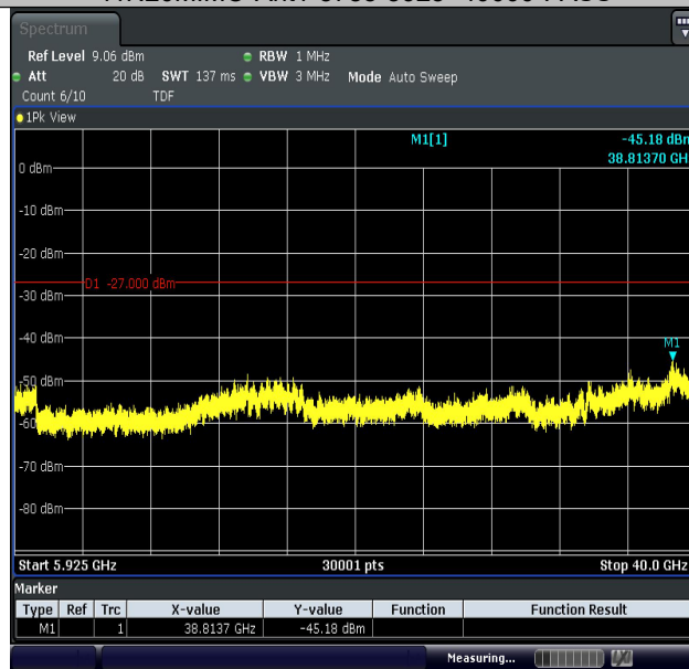
11N20MIMO-Ant2-5785-5925~40000-PASS
