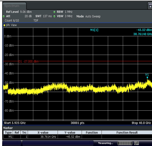
11A-Ant2-5785-5925~40000-PASS
