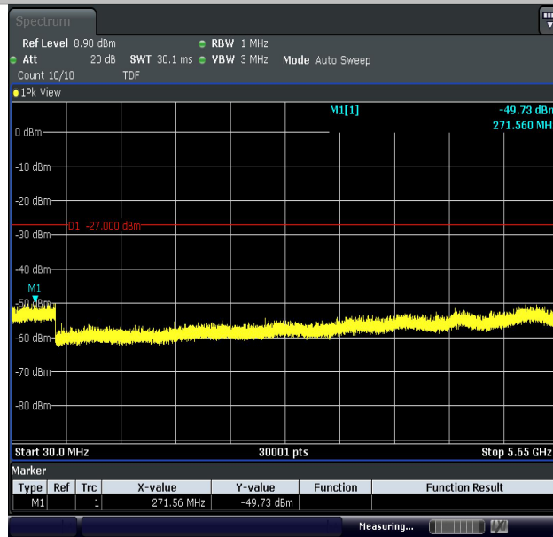
11N20MIMO-Ant2-5825-30~5650-PASS
