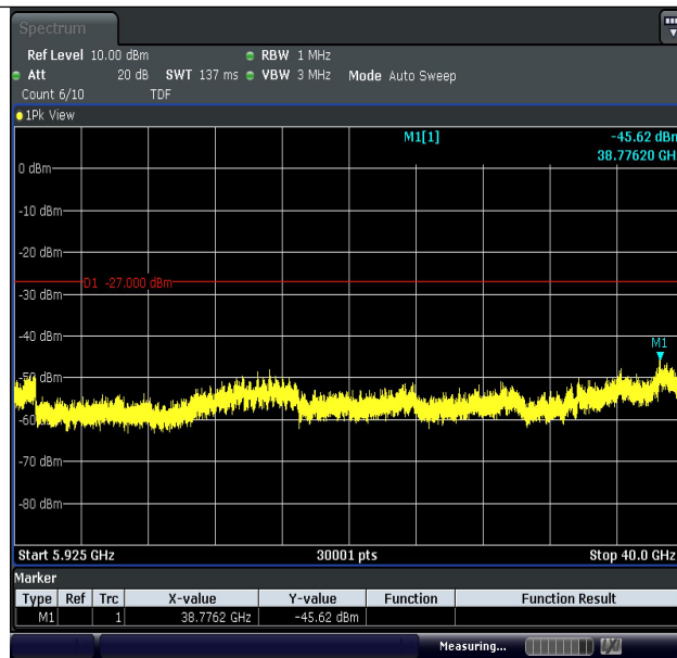
11N20MIMO-Ant1-5785-5925~40000-PASS
