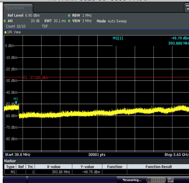
11A-Ant2-5825-30~5650-PASS
