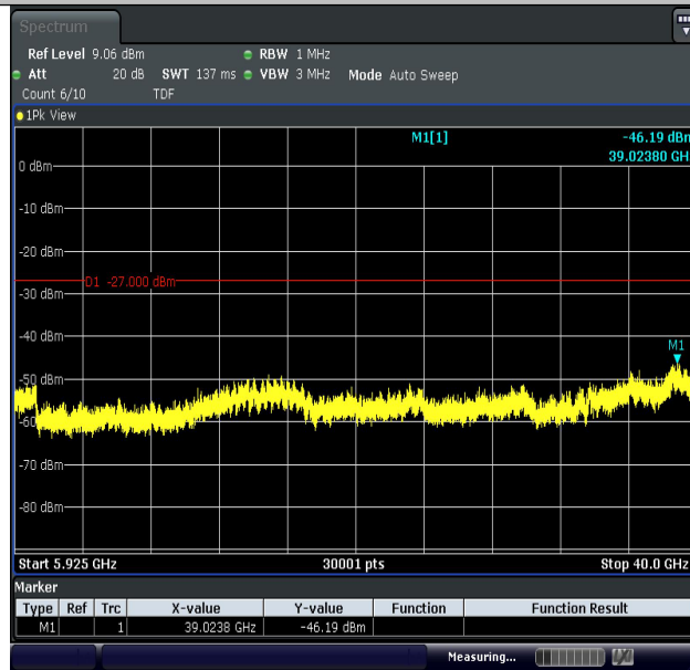
11N20MIMO-Ant2-5745-5925~40000-PASS
