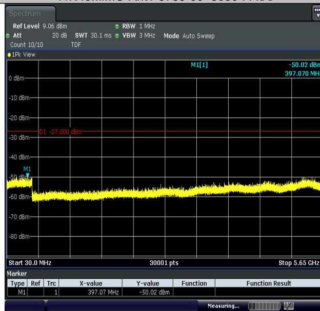
11N40MIMO-Ant2-5755-30~5650-PASS
