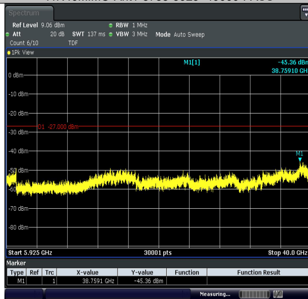
11N40MIMO-Ant2-5755-5925~40000-PASS
