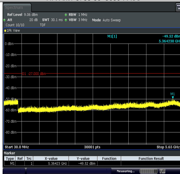
11A-Ant2-5785-30~5650-PASS
