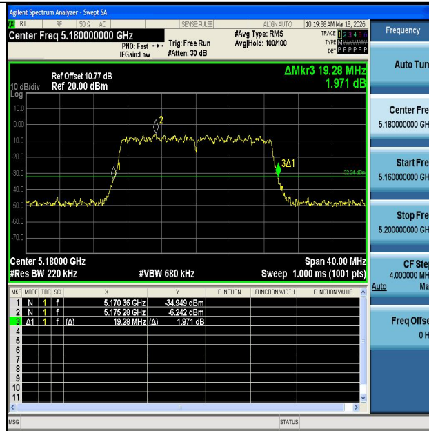
11N20MIMO-Ant1-5180
