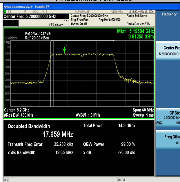
11AC20MIMO-Ant2-5200
