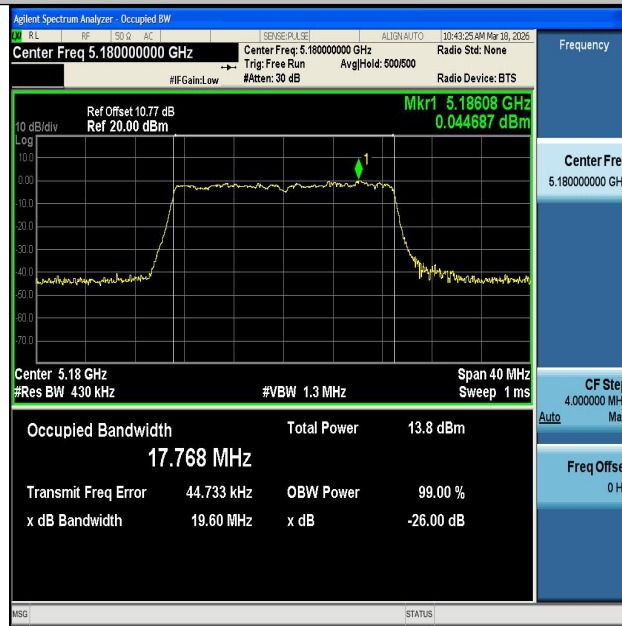
11AC20MIMO-Ant2-5180
