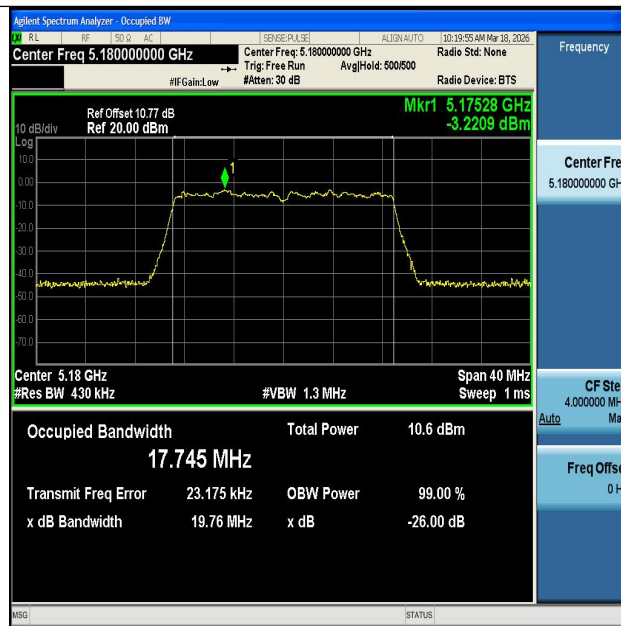
11N20MIMO-Ant1-5180
