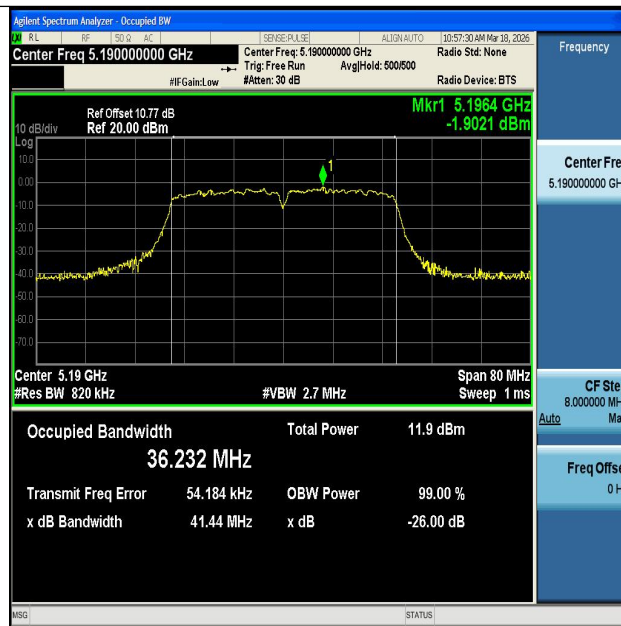
11AC40MIMO-Ant1-5190
