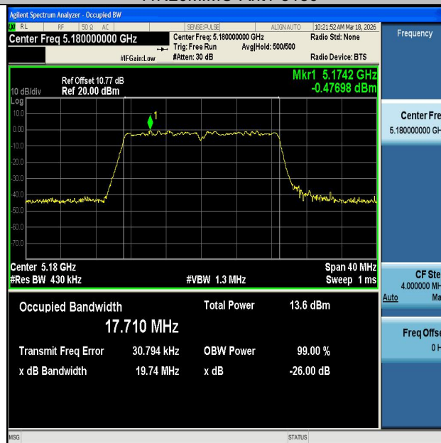
11N20MIMO-Ant2-5180
