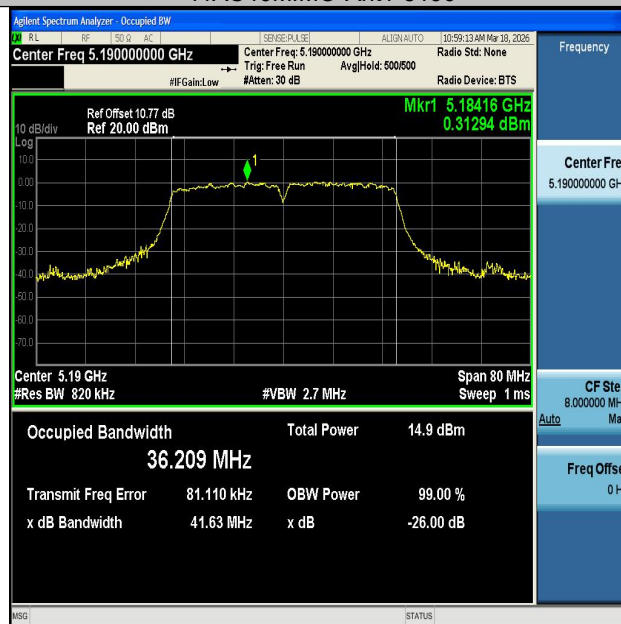
11AC40MIMO-Ant2-5190
