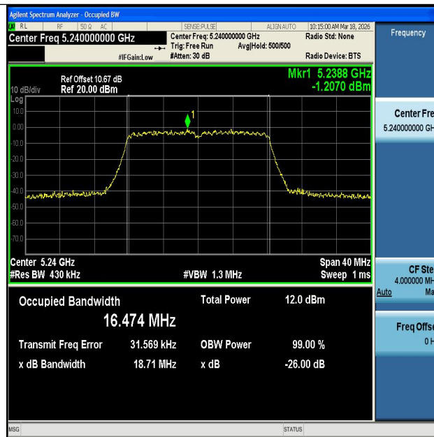
11A-Ant1-5240
