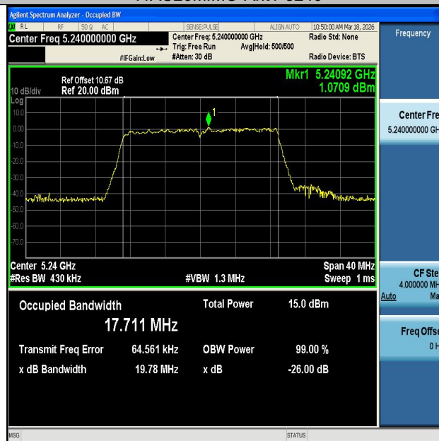
11AC20MIMO-Ant2-5240
