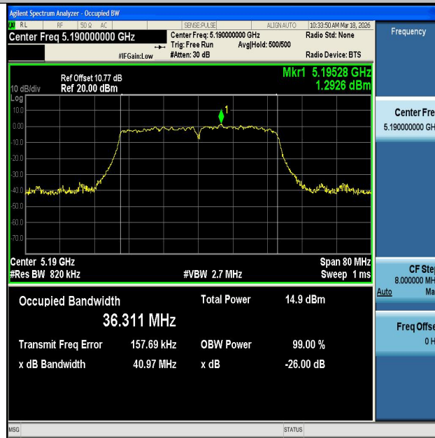
11N40MIMO-Ant2-5190
