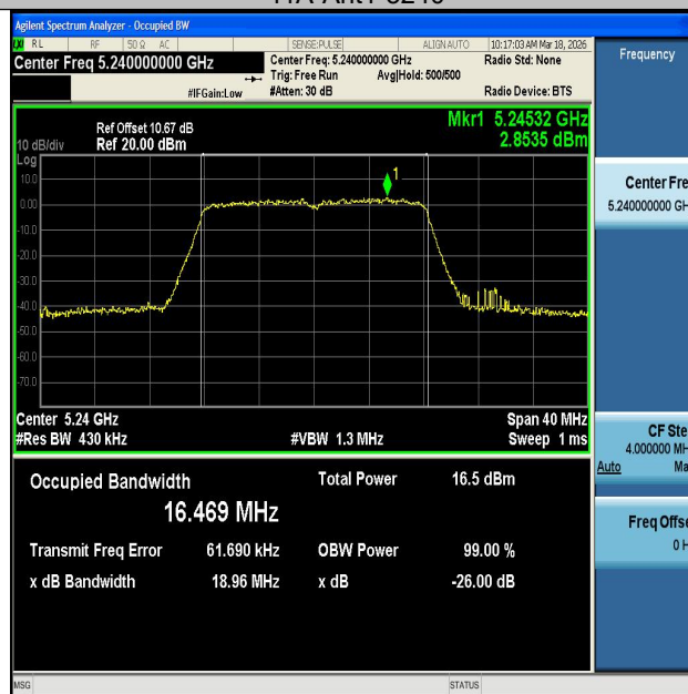
11A-Ant2-5240
