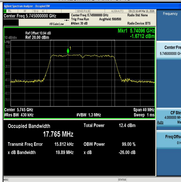
11N20MIMO-Ant2-5745
