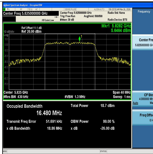
11A-Ant1-5825
