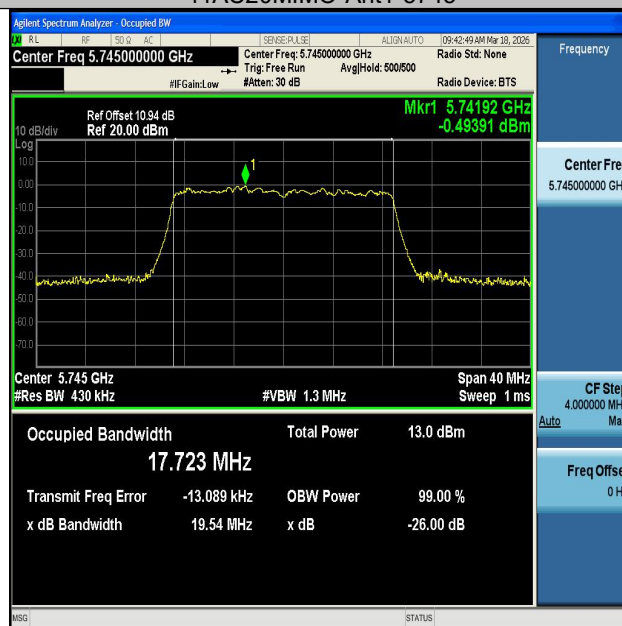
11AC20MIMO-Ant2-5745
