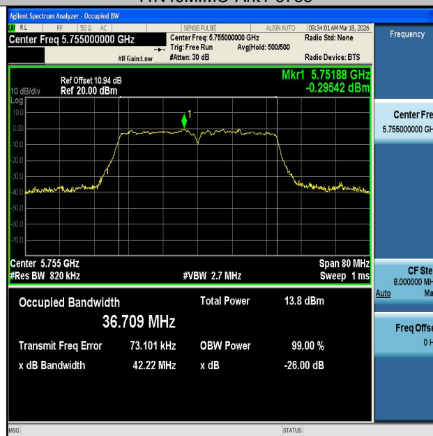
11N40MIMO-Ant2-5755
