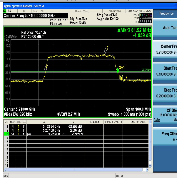
11AC80MIMO-Ant2-5210
