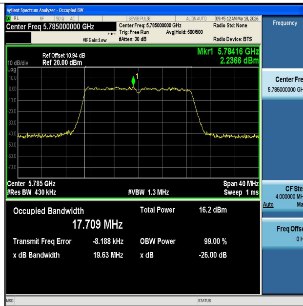
11AC20MIMO-Ant1-5785
