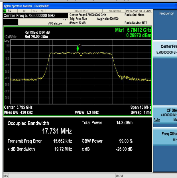
11AC20MIMO-Ant2-5785
