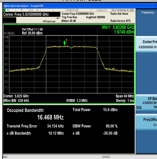
11A-Ant2-5825
