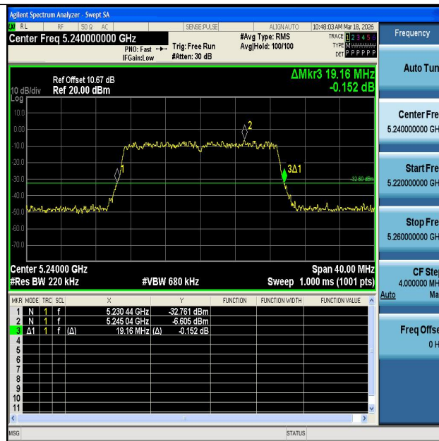
11AC20MIMO-Ant1-5240
