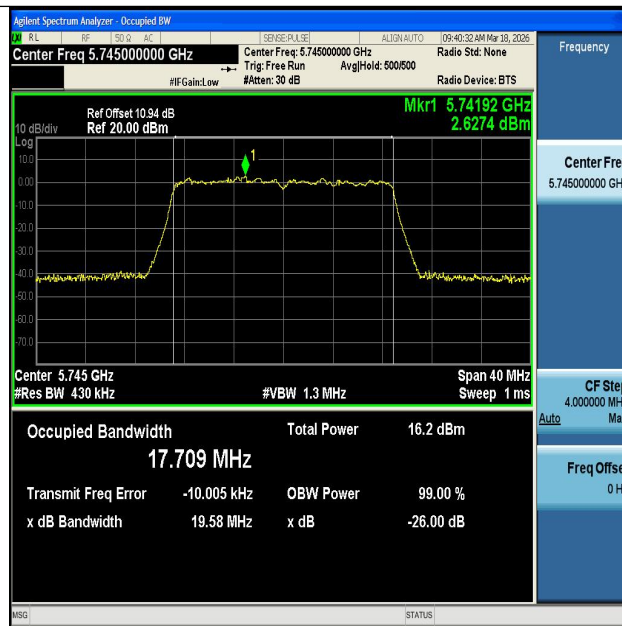
11AC20MIMO-Ant1-5745
