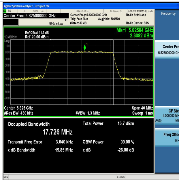
11AC20MIMO-Ant1-5825
