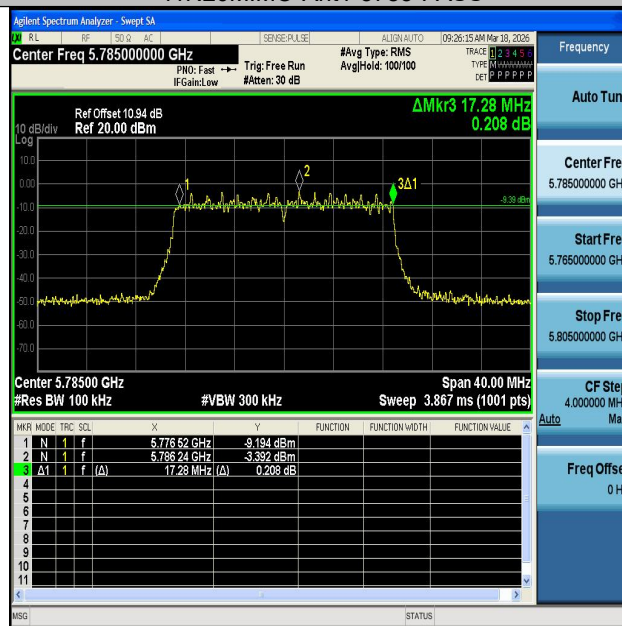
11N20MIMO-Ant2-5785-PASS
