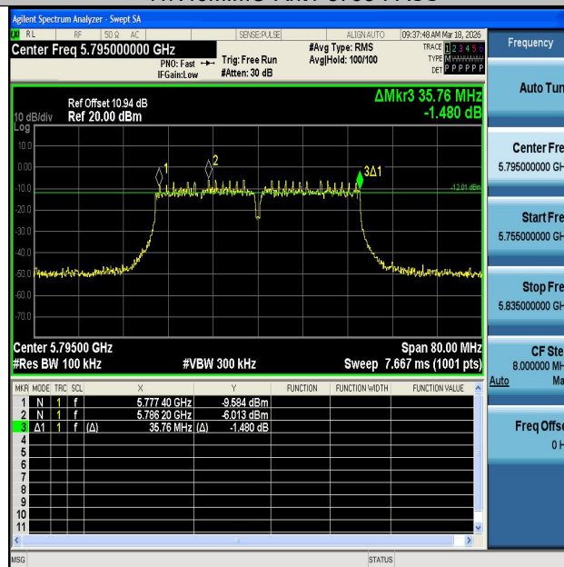
11N40MIMO-Ant2-5795-PASS
