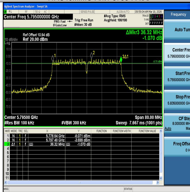
11AC40MIMO-Ant2-5795-PASS
