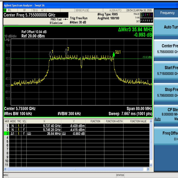
11AC40MIMO-Ant2-5755-PASS
