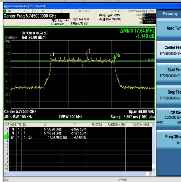
11N20MIMO-Ant2-5745-PASS
