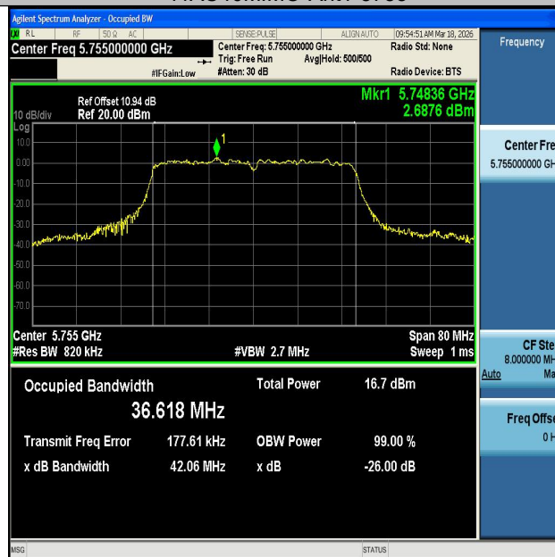
11AC40MIMO-Ant2-5755
