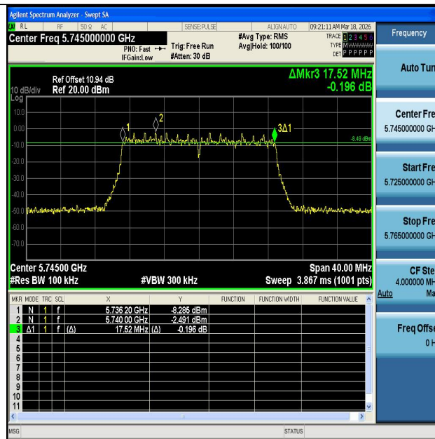
11N20MIMO-Ant1-5745-PASS
