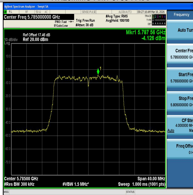
11N20MIMO-Ant2-5785-PASS
