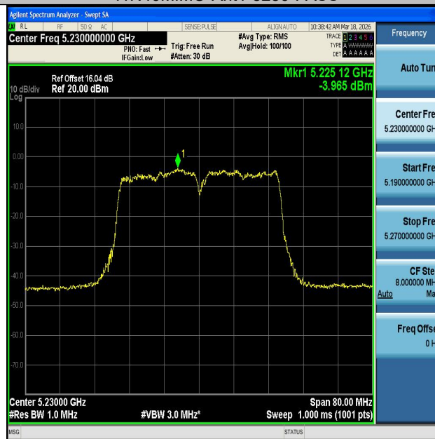
11N40MIMO-Ant2-5230-PASS
