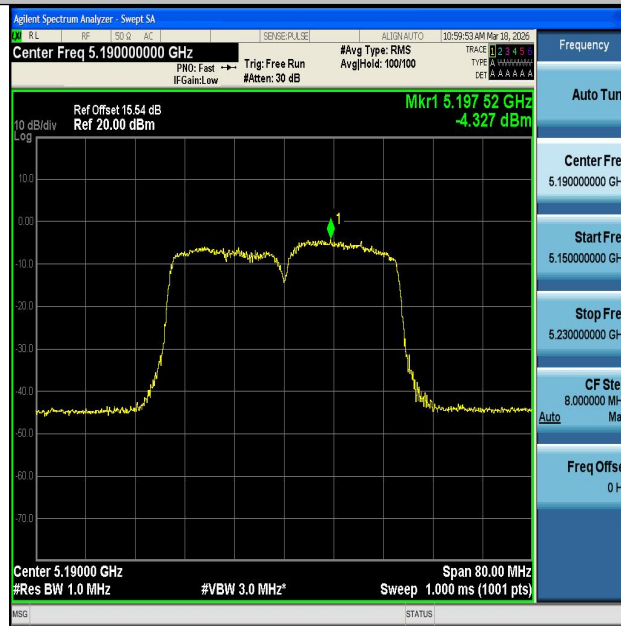
11AC40MIMO-Ant2-5190-PASS
