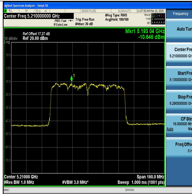
11AC80MIMO-Ant1-5210-PASS
