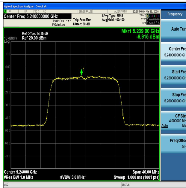
11N20MIMO-Ant1-5240-PASS
