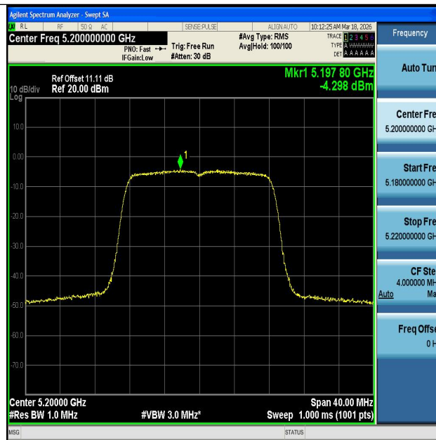
11A-Ant1-5200-PASS
