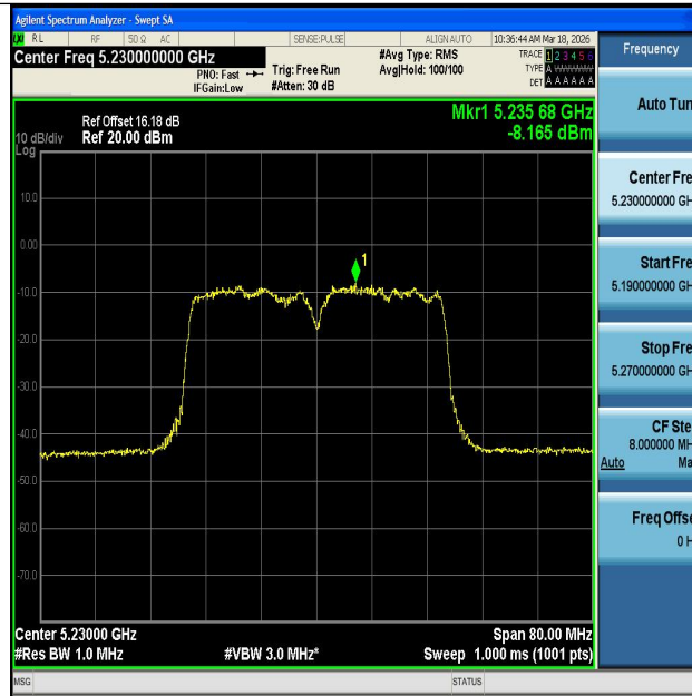
11N40MIMO-Ant1-5230-PASS
