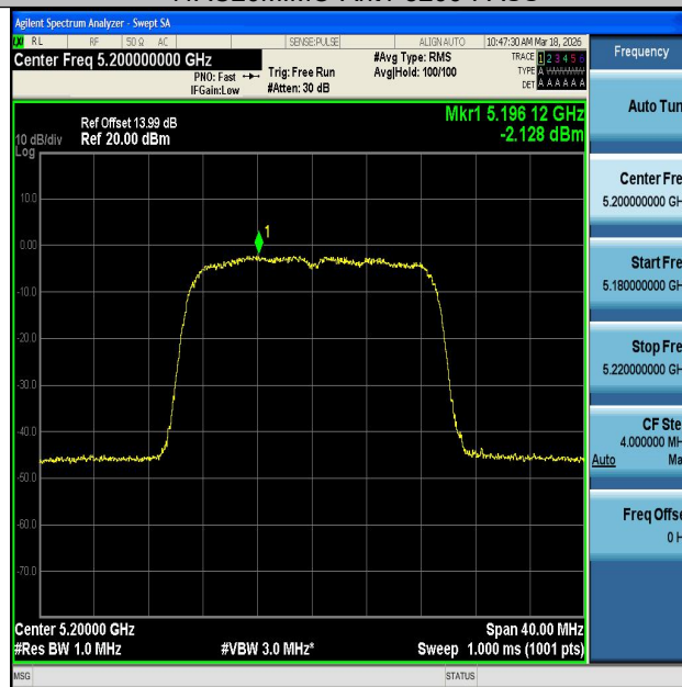
11AC20MIMO-Ant2-5200-PASS
