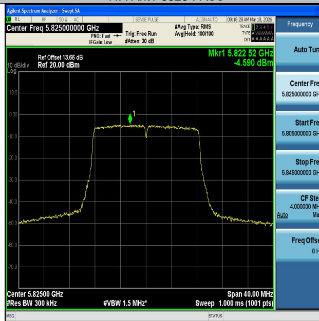
11A-Ant2-5825-PASS
