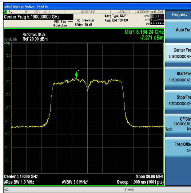
11N40MIMO-Ant1-5190-PASS
