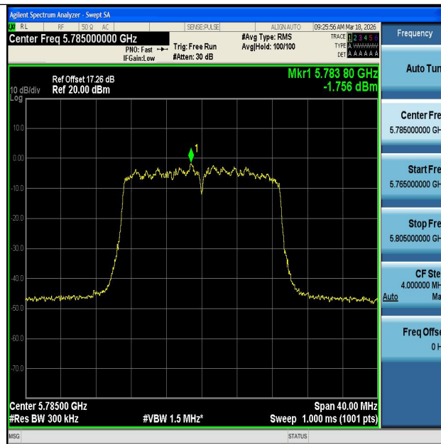
11N20MIMO-Ant1-5785-PASS
