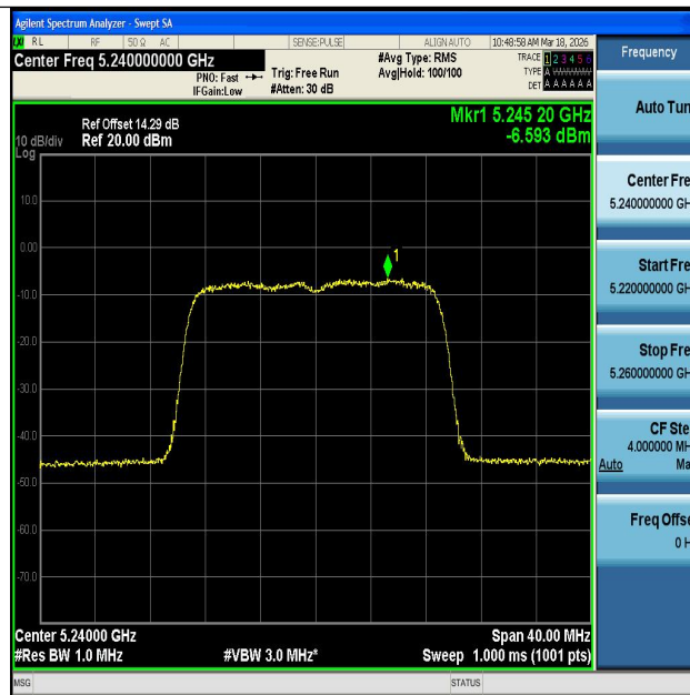
11AC20MIMO-Ant1-5240-PASS
