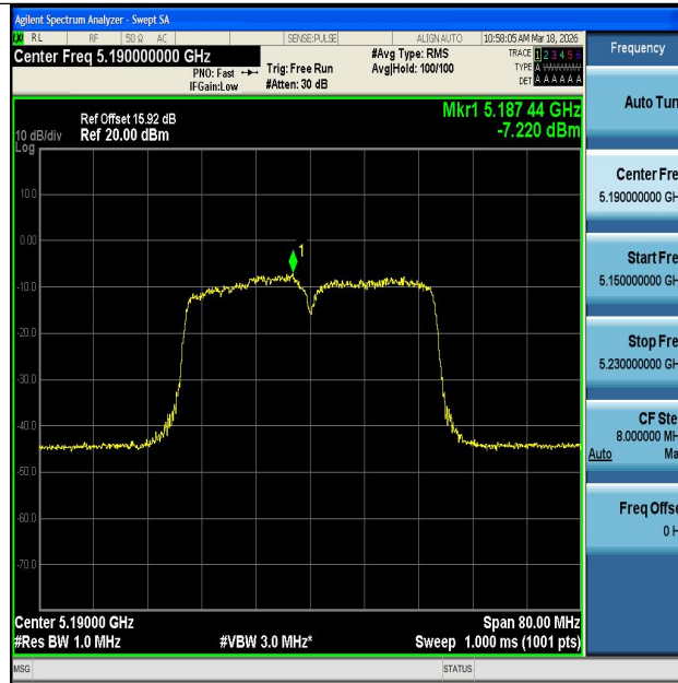
11AC40MIMO-Ant1-5190-PASS
