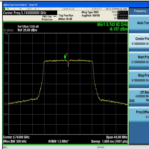
11A-Ant2-5745-PASS
