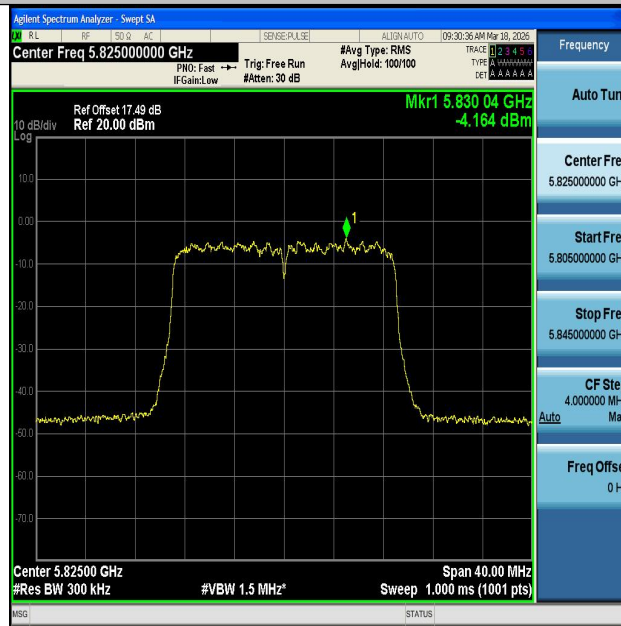
11N20MIMO-Ant2-5825-PASS
