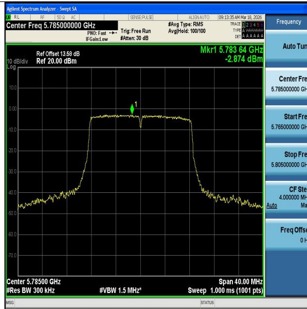
11A-Ant1-5785-PASS
