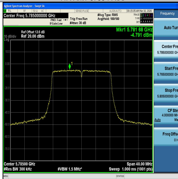
11A-Ant2-5785-PASS
