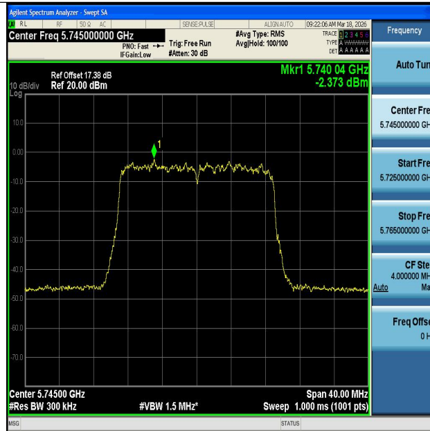
11N20MIMO-Ant1-5745-PASS
