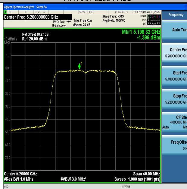
11A-Ant2-5200-PASS
