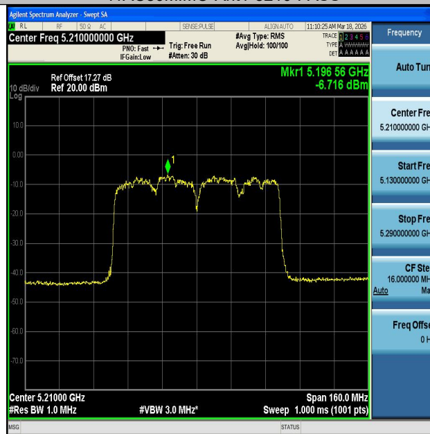
11AC80MIMO-Ant2-5210-PASS
