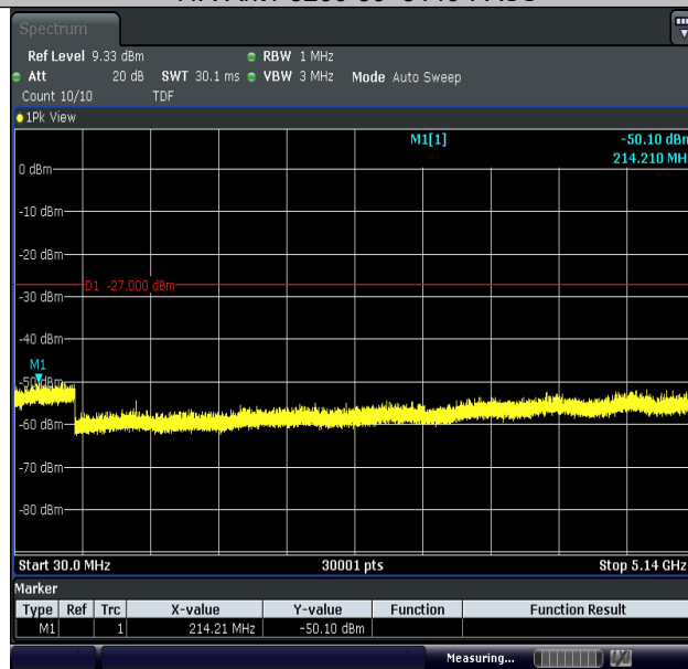
11A-Ant2-5200-30~5140-PASS
