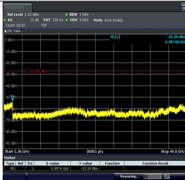
11N20MIMO-Ant2-5240-5360~40000-PASS
