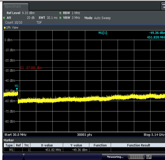
11N20MIMO-Ant2-5200-30~5140-PASS
