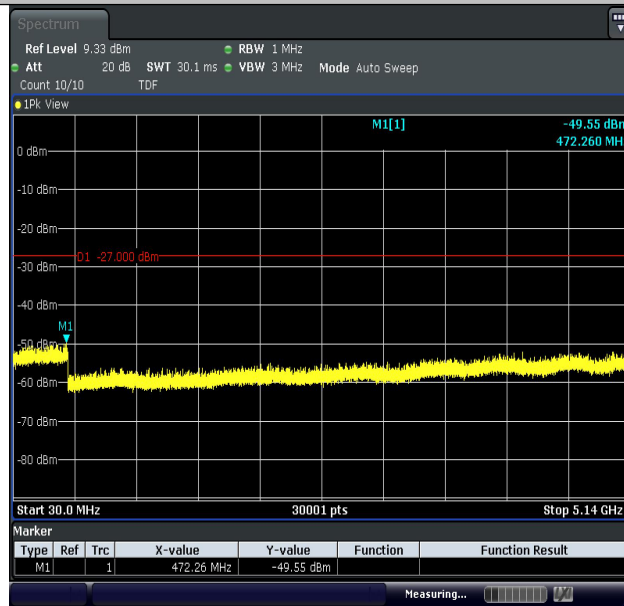
11N20MIMO-Ant2-5240-30~5140-PASS
