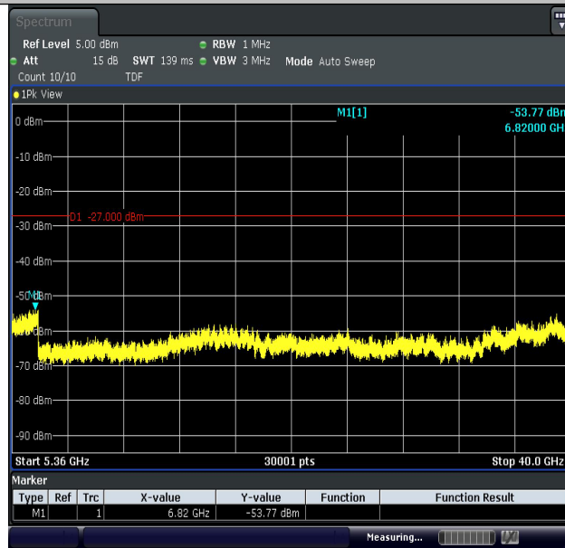
11N20MIMO-Ant2-5200-5360~40000-PASS
