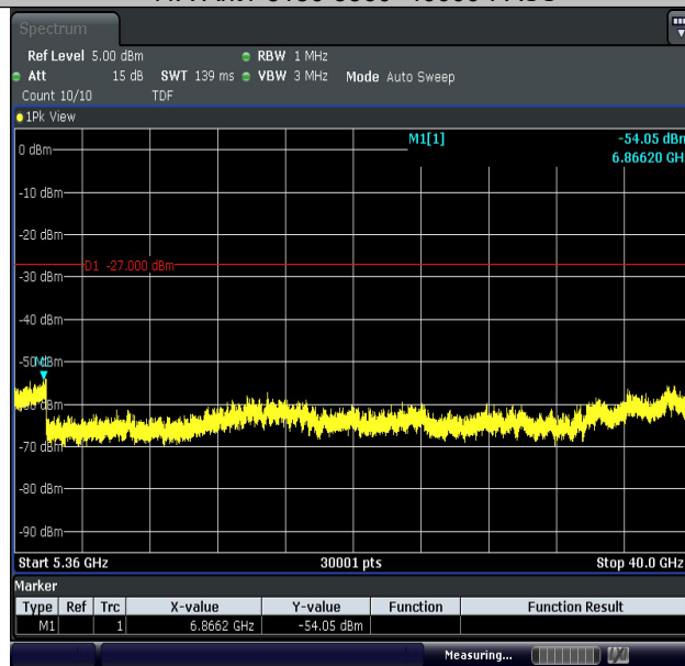
11A-Ant2-5180-5360~40000-PASS
