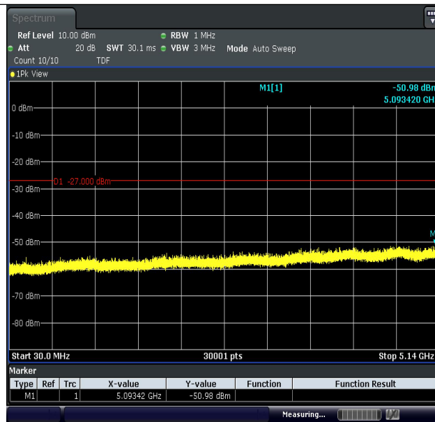
11A-Ant1-5200-30~5140-PASS
