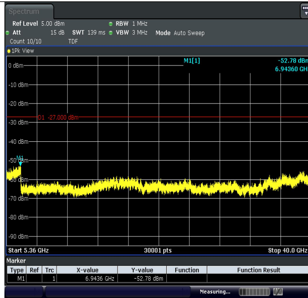
11N20MIMO-Ant1-5240-5360~40000-PASS
