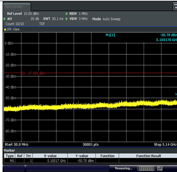
11N20MIMO-Ant1-5180-30~5140-PASS
