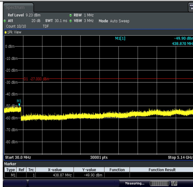
11N20MIMO-Ant2-5180-30~5140-PASS
