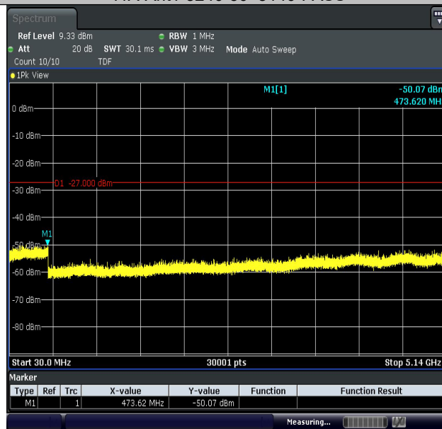
11A-Ant2-5240-30~5140-PASS
