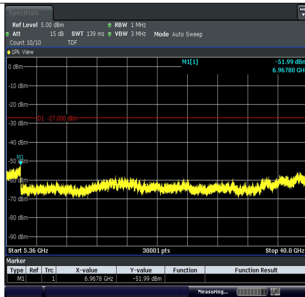
11A-Ant1-5180-5360~40000-PASS
