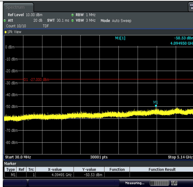
11AC40MIMO-Ant1-5190-30~5140-PASS
