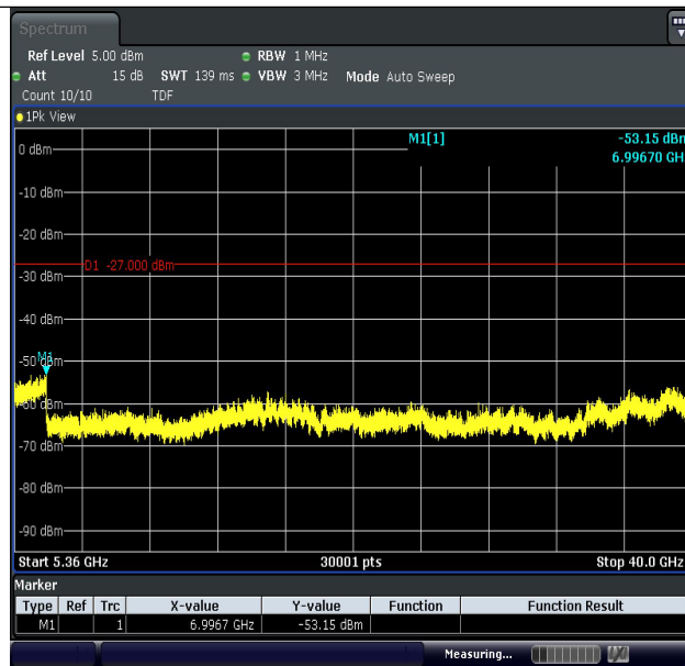
11AC40MIMO-Ant1-5190-5360~40000-PASS
