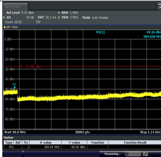
11AC20MIMO-Ant2-5240-30~5140-PASS
