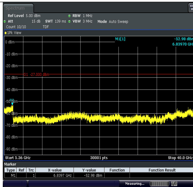
11AC40MIMO-Ant1-5230-5360~40000-PASS
