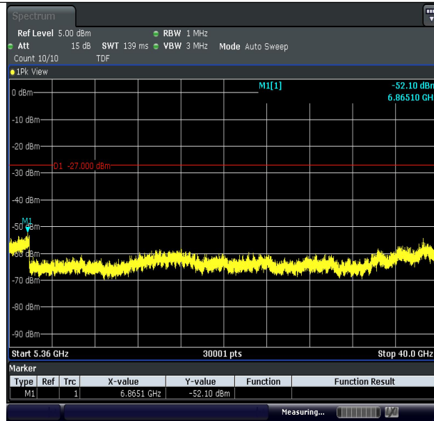
11N40MIMO-Ant1-5230-5360~40000-PASS
