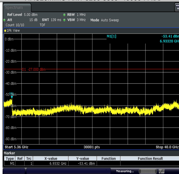
11AC20MIMO-Ant2-5200-5360~40000-PASS
