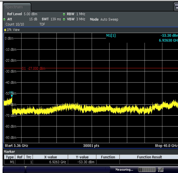
11AC20MIMO-Ant2-5240-5360~40000-PASS
