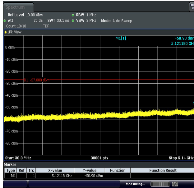
11N40MIMO-Ant1-5230-30~5140-PASS
