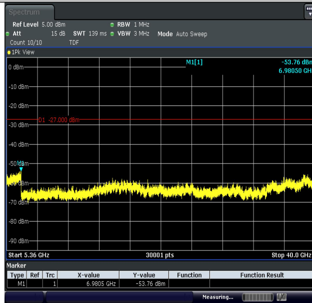
11N40MIMO-Ant2-5230-5360~40000-PASS
