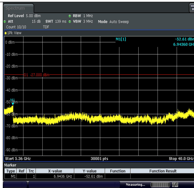
11AC20MIMO-Ant1-5200-5360~40000-PASS
