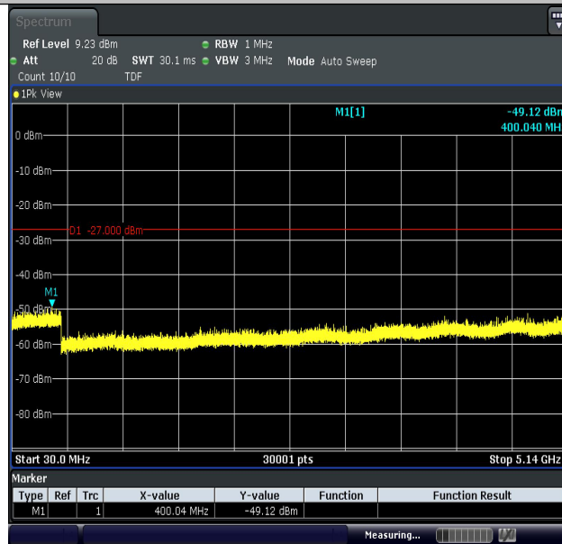
11AC40MIMO-Ant2-5190-30~5140-PASS
