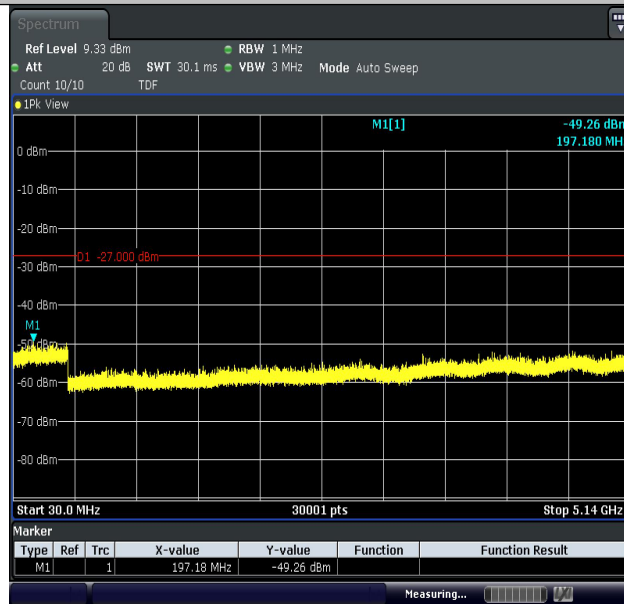
11N40MIMO-Ant2-5230-30~5140-PASS
