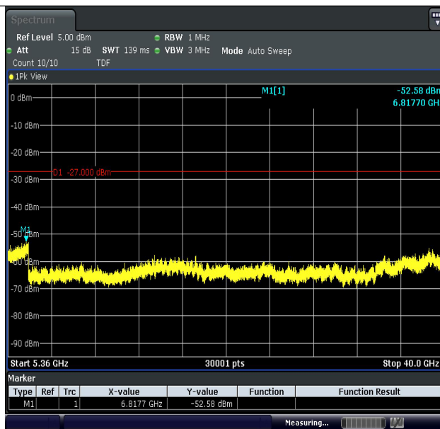
11N40MIMO-Ant1-5190-5360~40000-PASS
