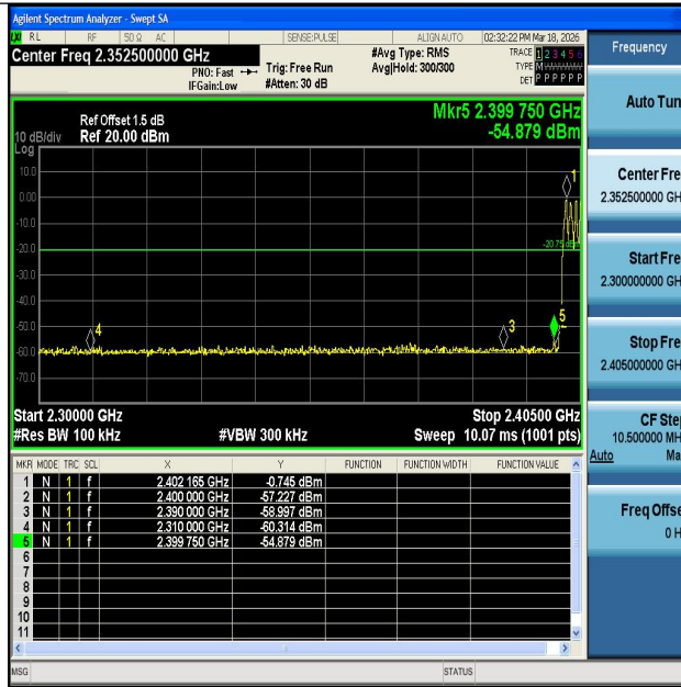
DH5-Ant1-Hop_2402-PASS
