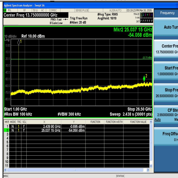
BLE_1M-Ant1-2440-1000~26500-PASS
