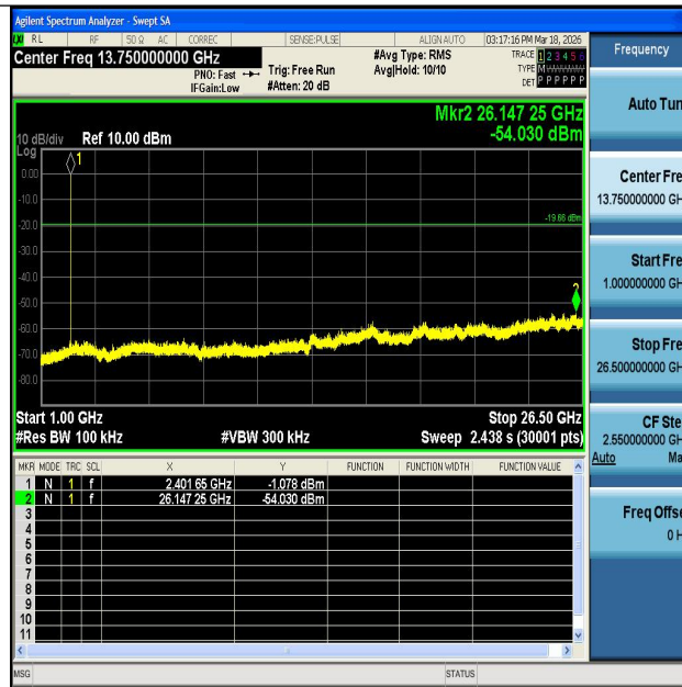
BLE_1M-Ant1-2402-1000~26500-PASS
