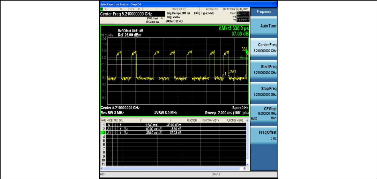
NTNV-11AC80MIMO-Ant2-5210
