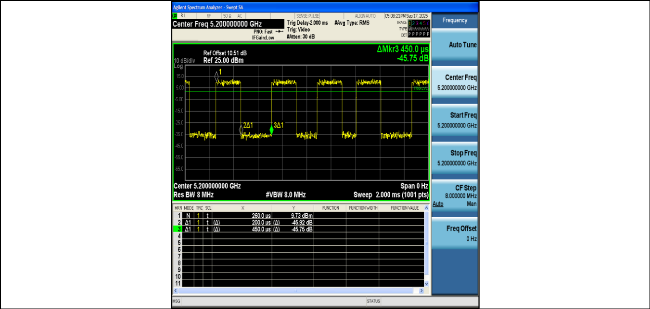
NTNV-11AC20MIMO-Ant2-5200
