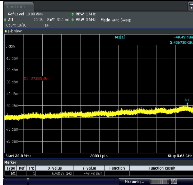
11AC20MIMO-Ant1-5745-30~5650-PASS
