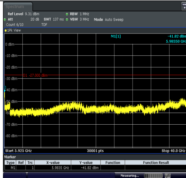
11N40MIMO-Ant2-5755-5925~40000-PASS
