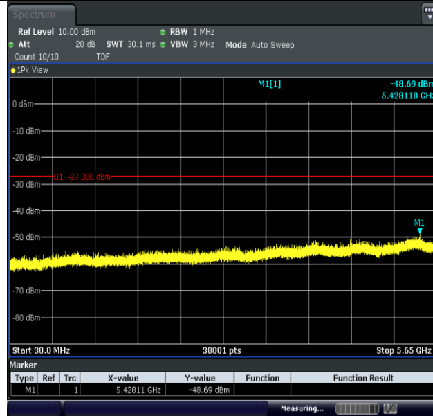
11AC40MIMO-Ant1-5755-30~5650-PASS
