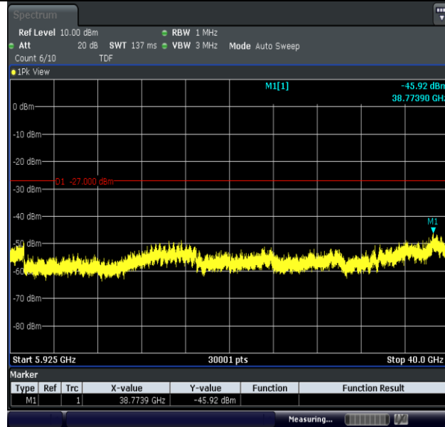
11N20MIMO-Ant1-5785-5925~40000-PASS
