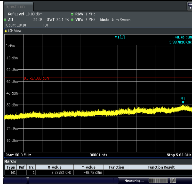
11N40MIMO-Ant1-5755-30~5650-PASS
