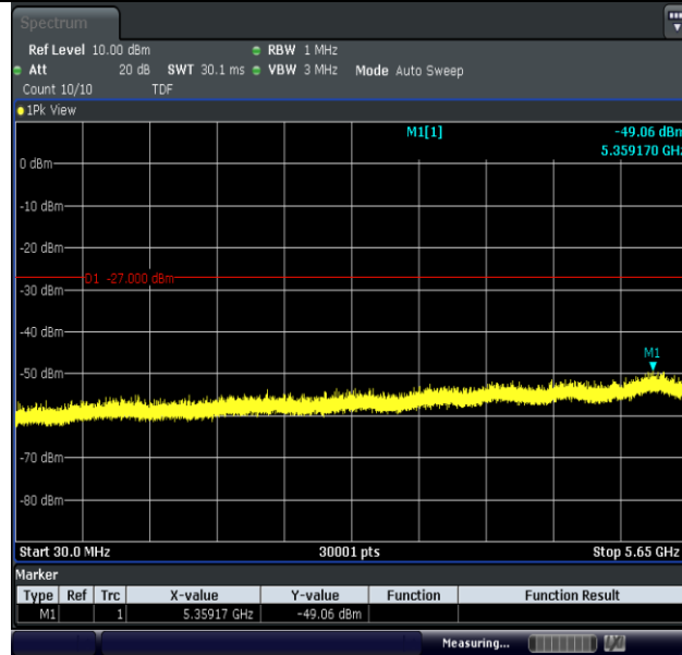
11AC20MIMO-Ant1-5825-30~5650-PASS
