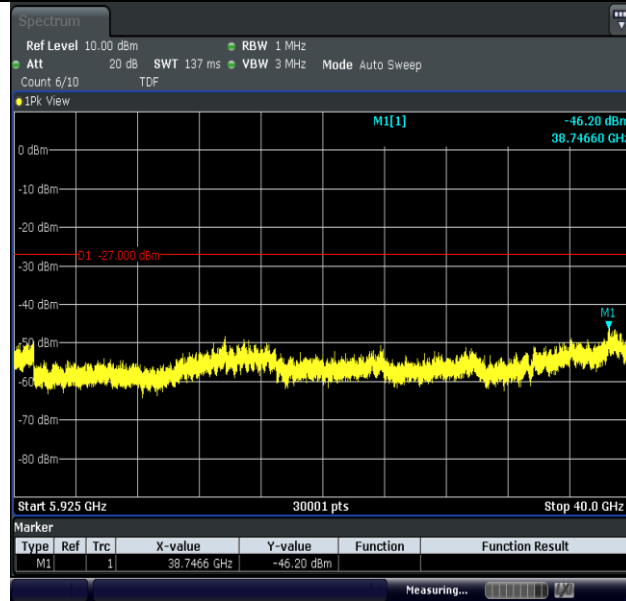
11AC40MIMO-Ant1-5795-5925~40000-PASS
