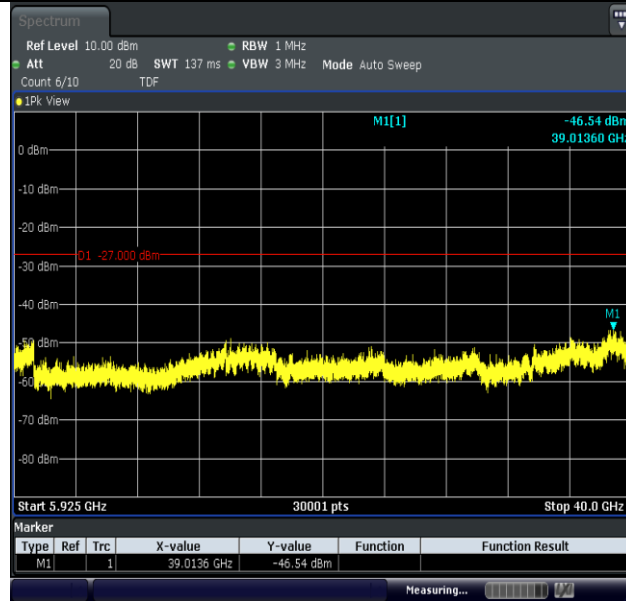
11AC20MIMO-Ant1-5785-5925~40000-PASS
