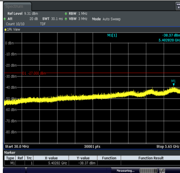
11AC20MIMO-Ant2-5825-30~5650-PASS
