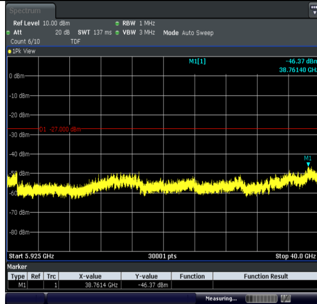
11N40MIMO-Ant1-5795-5925~40000-PASS
