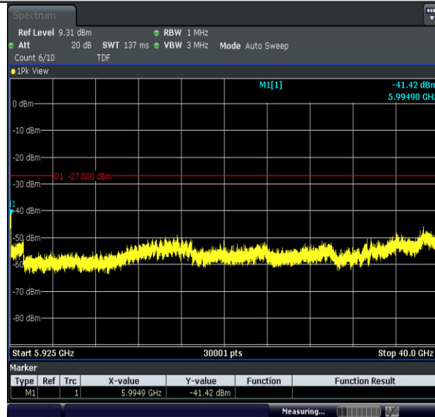
11AC80MIMO-Ant2-5775-5925~40000-PASS
