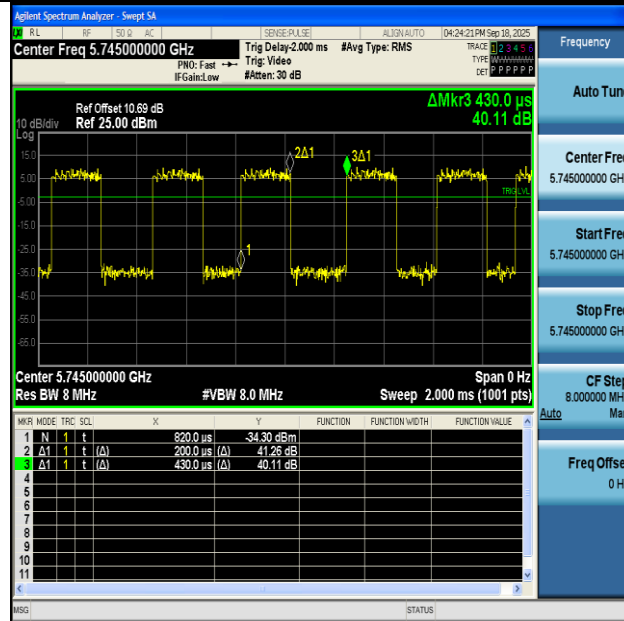
NTNV-11AC20MIMO-Ant1-5745
