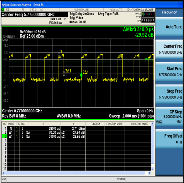
NTNV-11AC80MIMO-Ant1-5775
