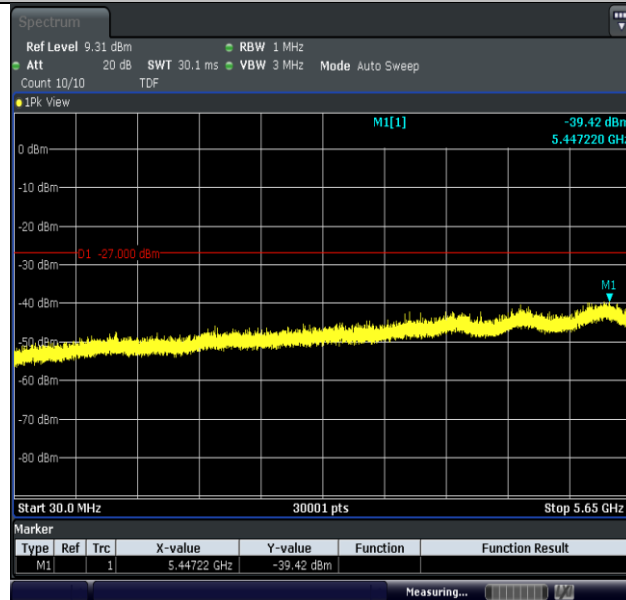
11N20MIMO-Ant2-5745-30~5650-PASS
