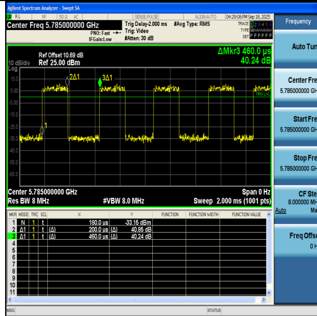
NTNV-11AC20MIMO-Ant1-5785
