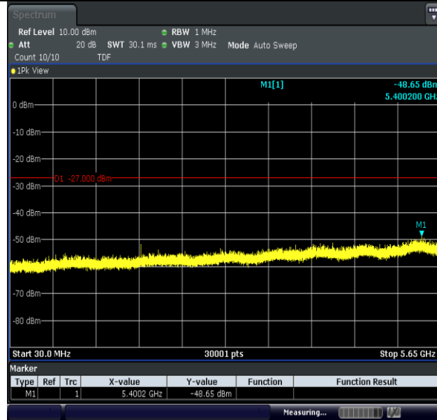
11N20MIMO-Ant1-5785-30~5650-PASS
