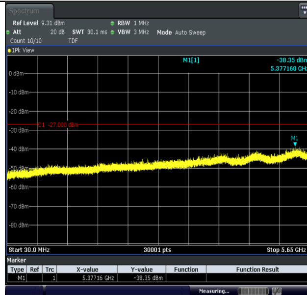
11AC20MIMO-Ant2-5785-30~5650-PASS
