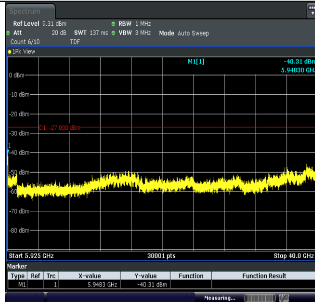
11AC20MIMO-Ant2-5825-5925~40000-PASS
