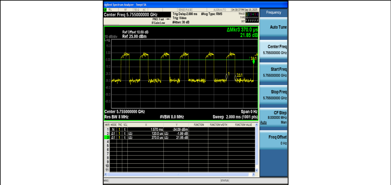
NTNV-11AC40MIMO-Ant1-5755
