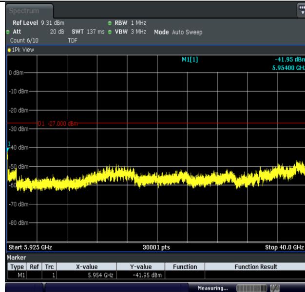
11AC40MIMO-Ant2-5755-5925~40000-PASS
