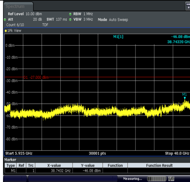
11AC80MIMO-Ant1-5775-5925~40000-PASS
