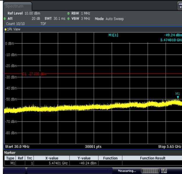
11AC20MIMO-Ant1-5785-30~5650-PASS
