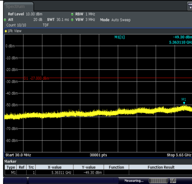
11N20MIMO-Ant1-5825-30~5650-PASS
