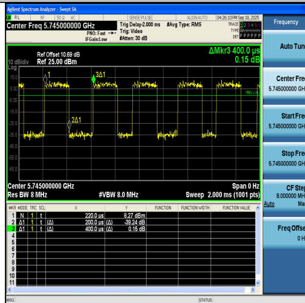
NTNV-11AC20MIMO-Ant2-5745
