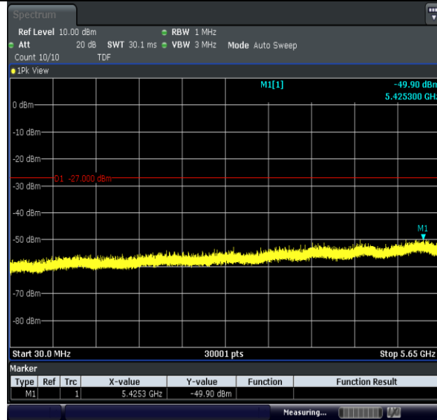
11N20MIMO-Ant1-5745-30~5650-PASS
