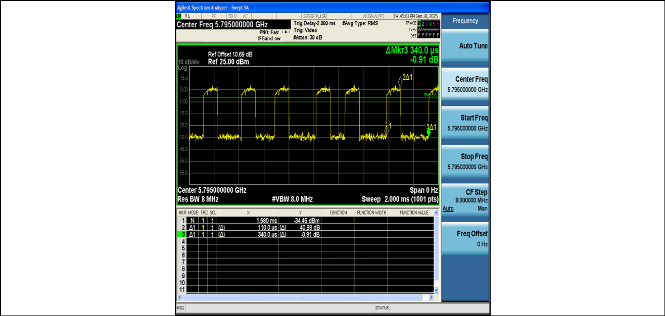
NTNV-11AC40MIMO-Ant2-5795
