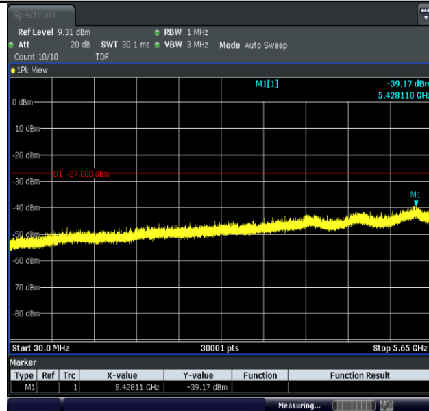
11N20MIMO-Ant2-5785-30~5650-PASS
