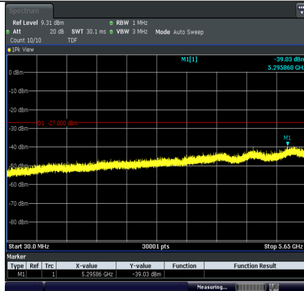
11AC80MIMO-Ant2-5775-30~5650-PASS
