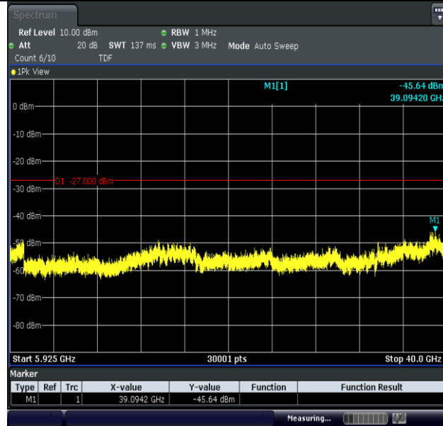
11N20MIMO-Ant1-5825-5925~40000-PASS
