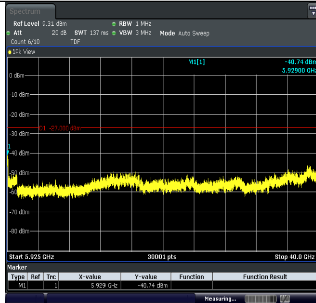
11N20MIMO-Ant2-5745-5925~40000-PASS
