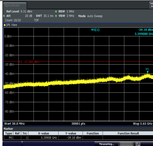
11AC20MIMO-Ant2-5745-30~5650-PASS
