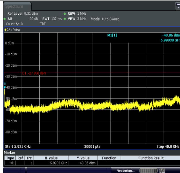
11N20MIMO-Ant2-5785-5925~40000-PASS
