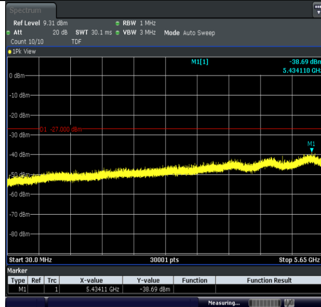
11N40MIMO-Ant2-5755-30~5650-PASS
