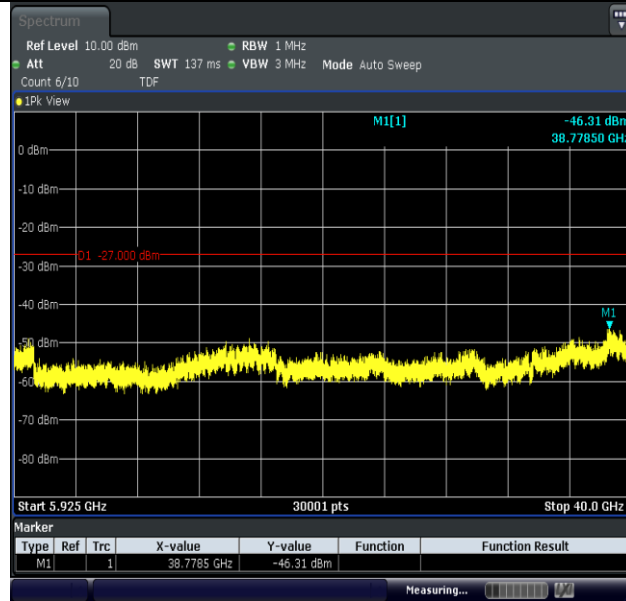
11AC20MIMO-Ant1-5825-5925~40000-PASS
