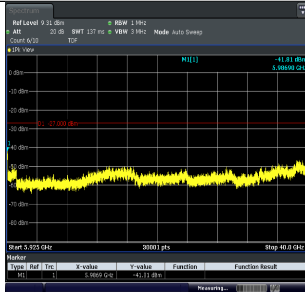
11N20MIMO-Ant2-5825-5925~40000-PASS
