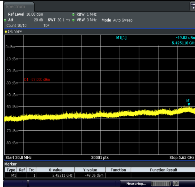
11AC40MIMO-Ant1-5795-30~5650-PASS
