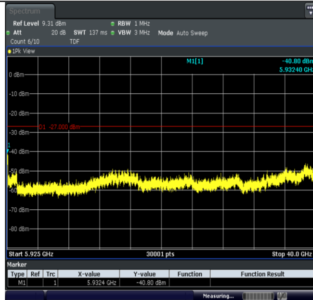
11N40MIMO-Ant2-5795-5925~40000-PASS
