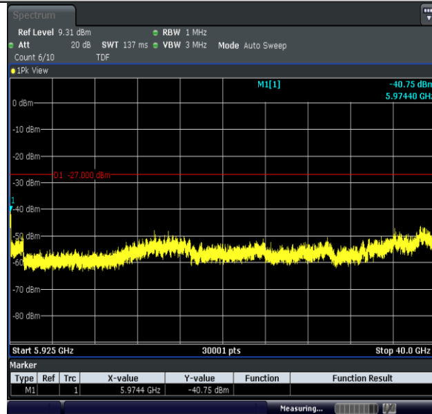
11AC20MIMO-Ant2-5785-5925~40000-PASS
