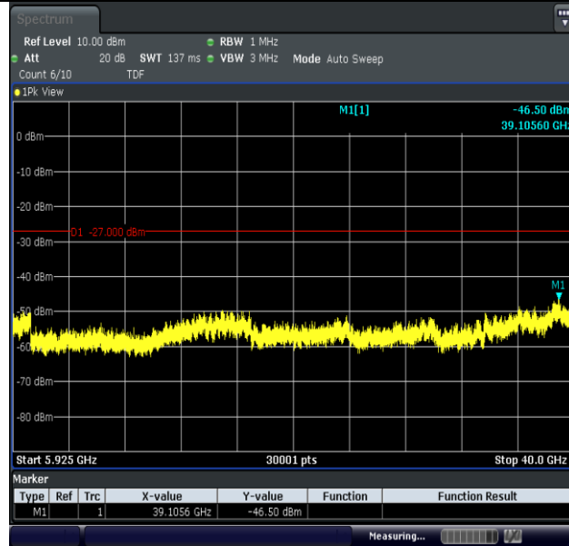
11AC20MIMO-Ant1-5745-5925~40000-PASS
