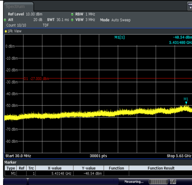
11N40MIMO-Ant1-5795-30~5650-PASS
