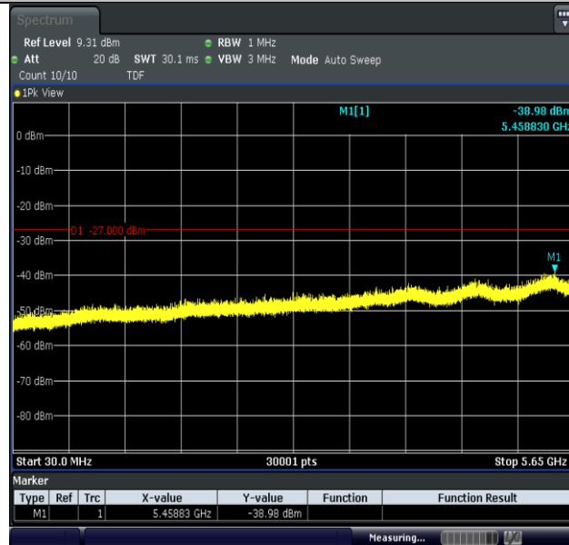
11N40MIMO-Ant2-5795-30~5650-PASS
