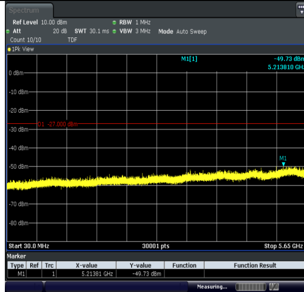
11AC80MIMO-Ant1-5775-30~5650-PASS
