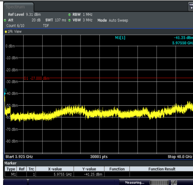
11AC40MIMO-Ant2-5795-5925~40000-PASS
