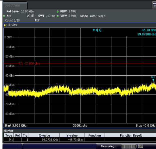
11N40MIMO-Ant1-5755-5925~40000-PASS
