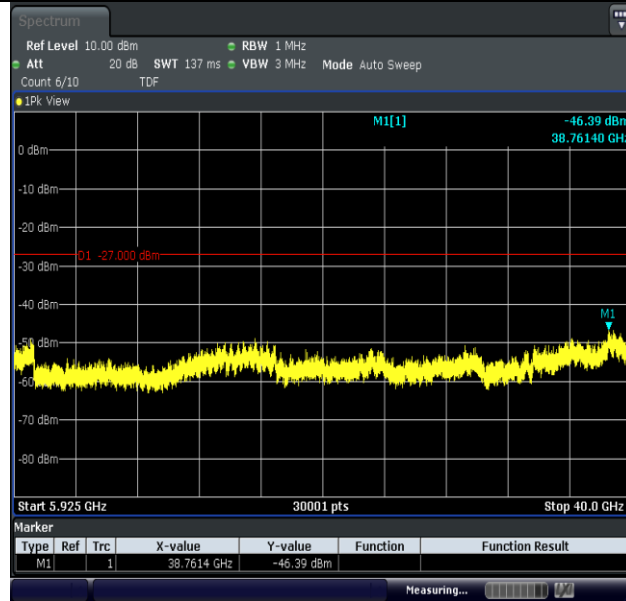
11AC40MIMO-Ant1-5755-5925~40000-PASS
