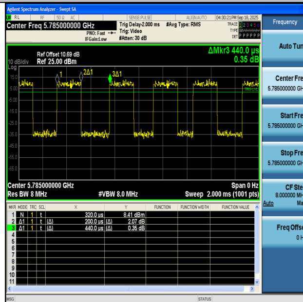
NTNV-11AC20MIMO-Ant2-5785
