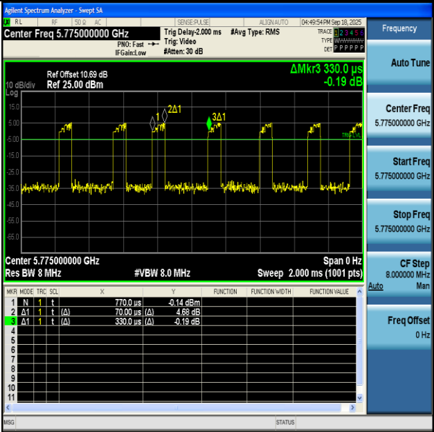
NTNV-11AC80MIMO-Ant2-5775
