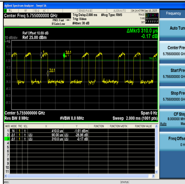
NTNV-11N40MIMO-Ant2-5755
