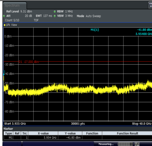
11AC20MIMO-Ant2-5745-5925~40000-PASS
