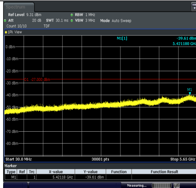
11AC40MIMO-Ant2-5755-30~5650-PASS
