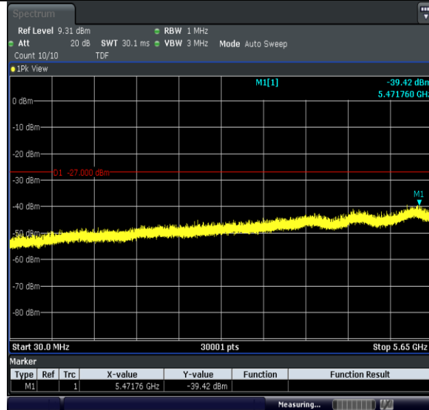
11N20MIMO-Ant2-5825-30~5650-PASS
