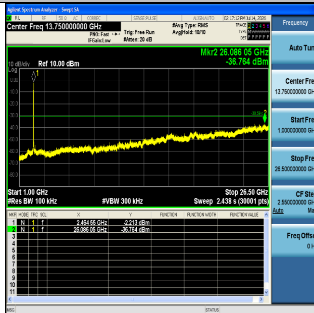
11N20MIMO-Ant2-2462-1000~26500-PASS
