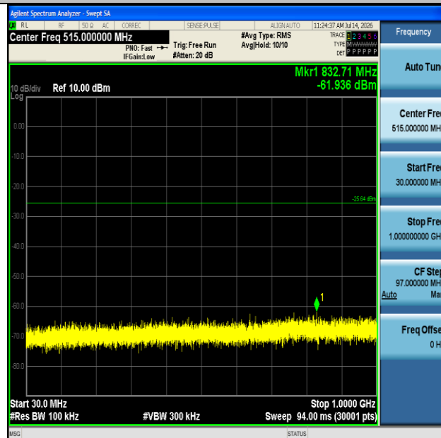
11B-Ant2-2437-30~1000-PASS
