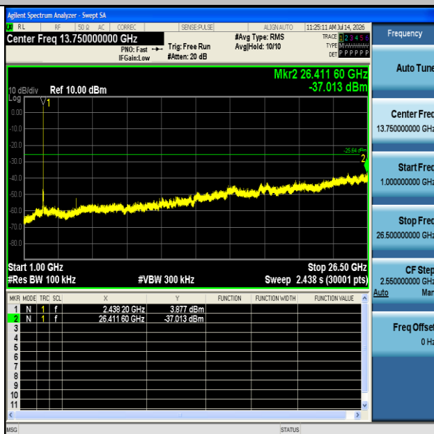
11B-Ant2-2437-1000~26500-PASS
