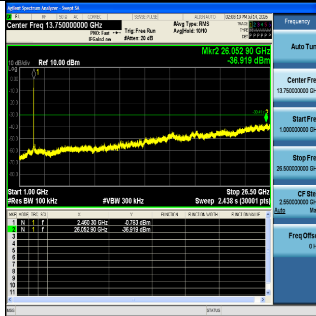
11N20MIMO-Ant1-2462-1000~26500-PASS
