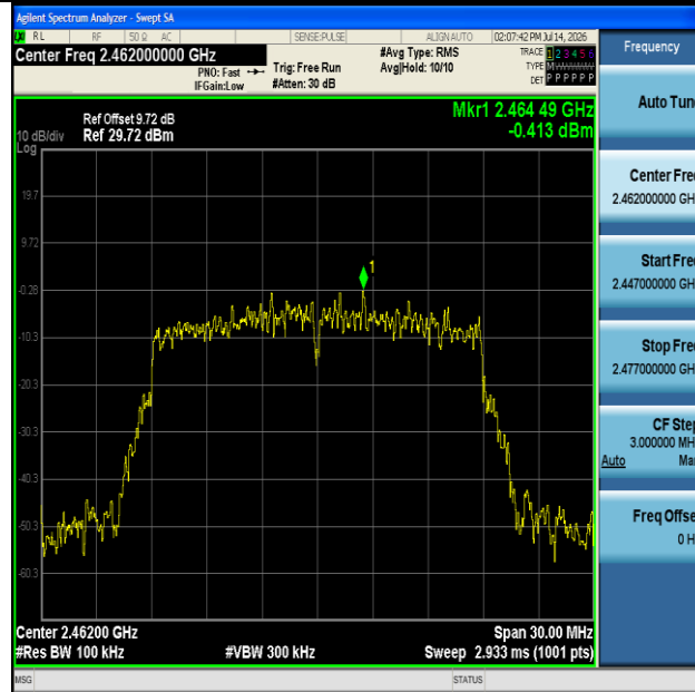
11N20MIMO-Ant1-2462-0~Reference-PASS
