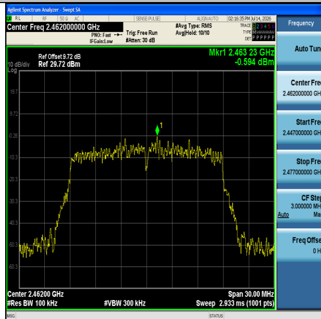
11N20MIMO-Ant2-2462-0~Reference-PASS
