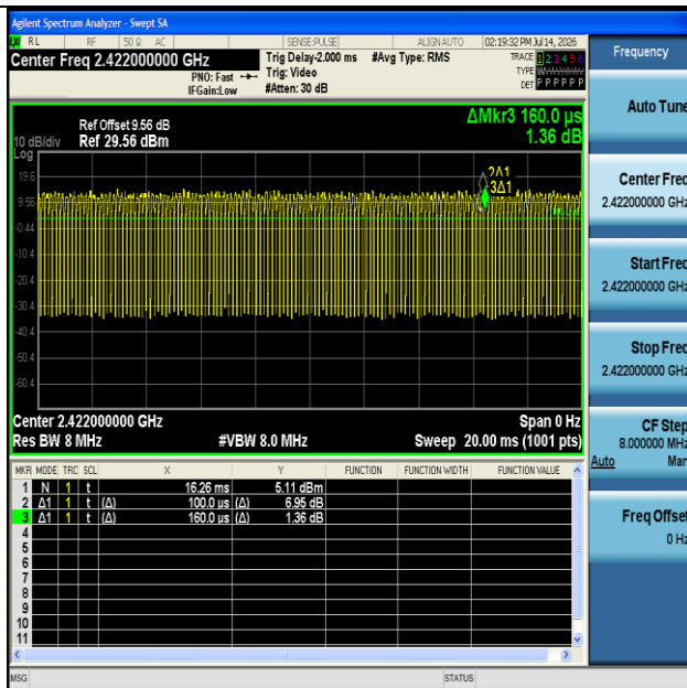
NTNV-11N40MIMO-Ant1-2422
