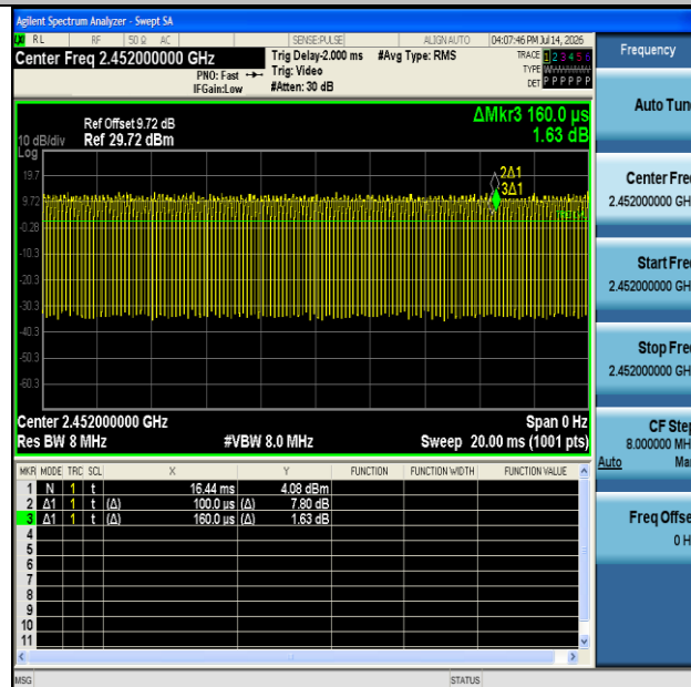
NTVN-11N40MIMO-Ant2-2452
