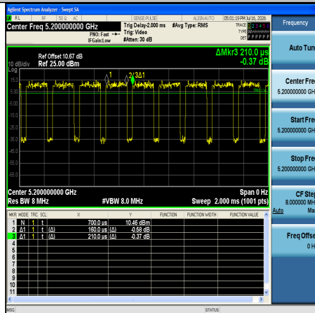
NTNV-11AC20MIMO-Ant2-5200
