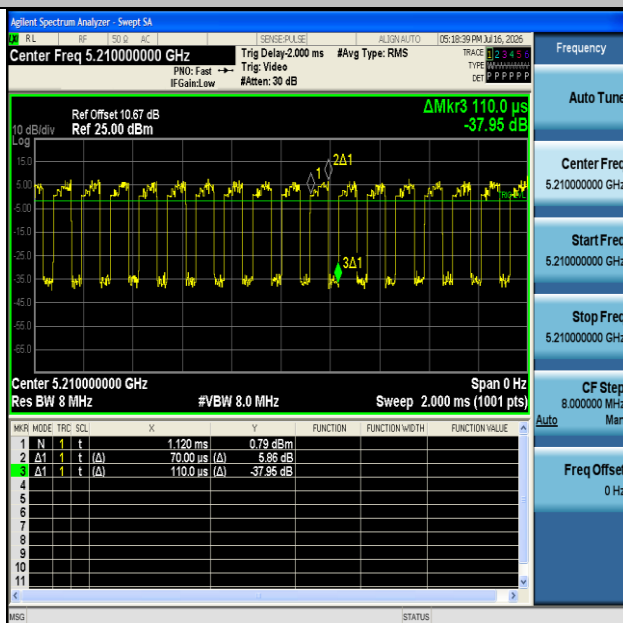
NTNV-11AC80MIMO-Ant2-5210
