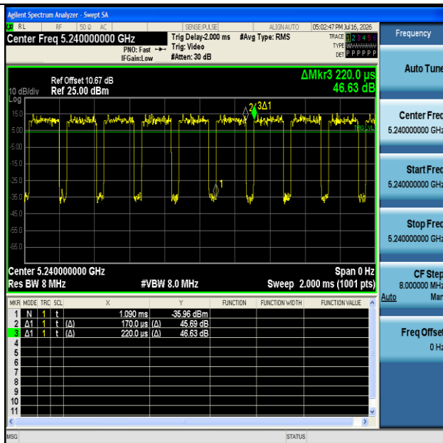
NTNV-11AC20MIMO-Ant1-5240
