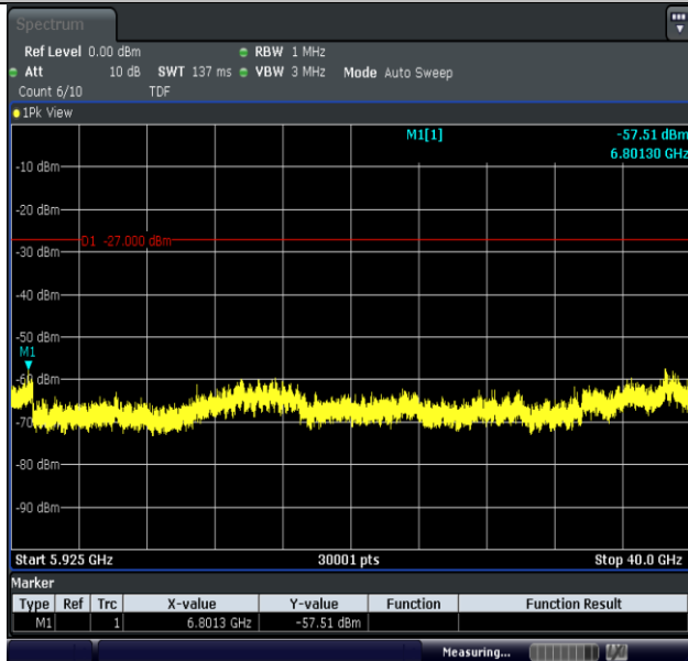
11AC40MIMO-Ant2-5755-5925~40000-PASS
