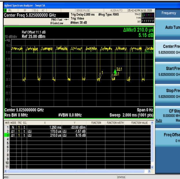
NTNV-11N20MIMO-Ant2-5825
