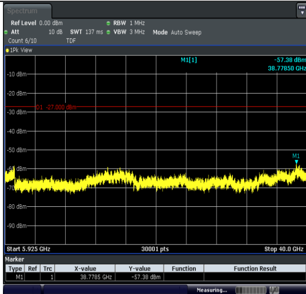
11AC20MIMO-Ant2-5785-5925~40000-PASS
