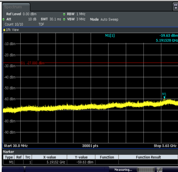
11A-Ant2-5825-30~5650-PASS
