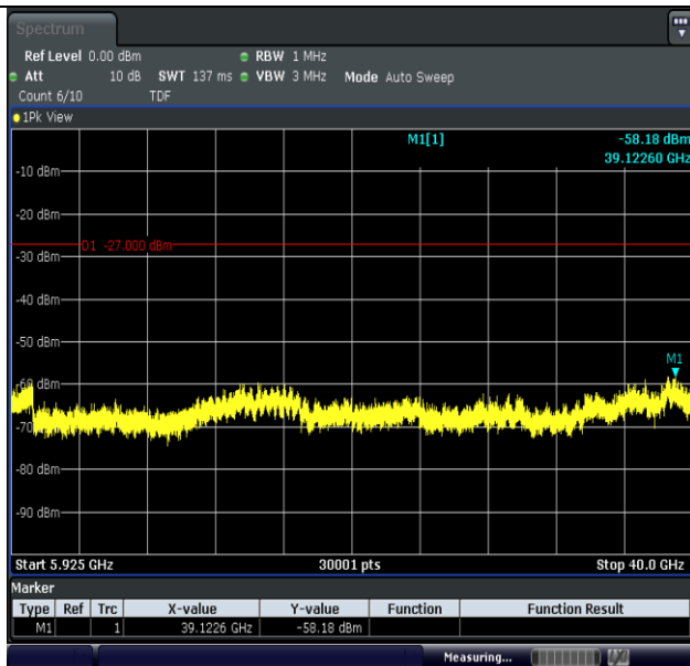
11A-Ant1-5785-5925~40000-PASS
