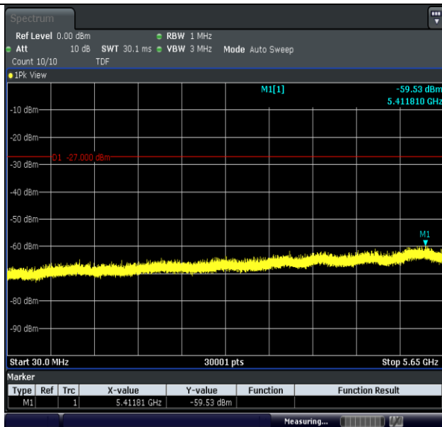
11N40MIMO-Ant1-5795-30~5650-PASS
