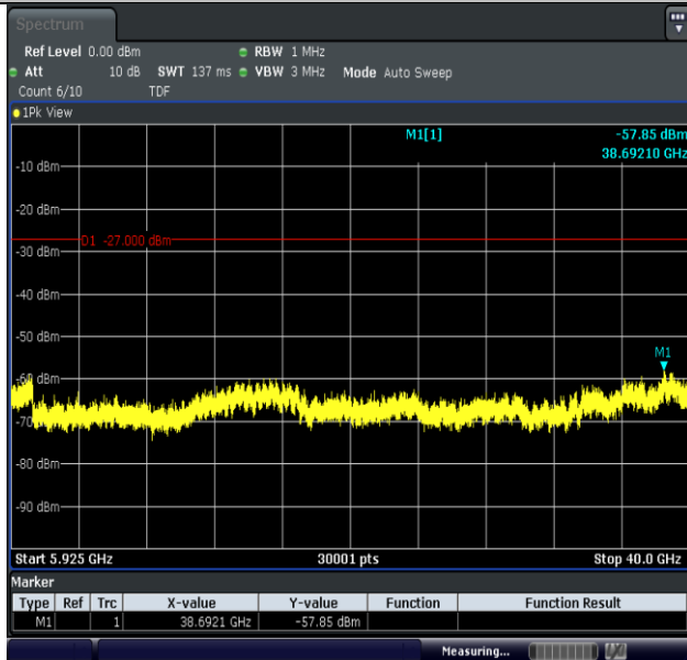
11AC40MIMO-Ant2-5795-5925~40000-PASS
