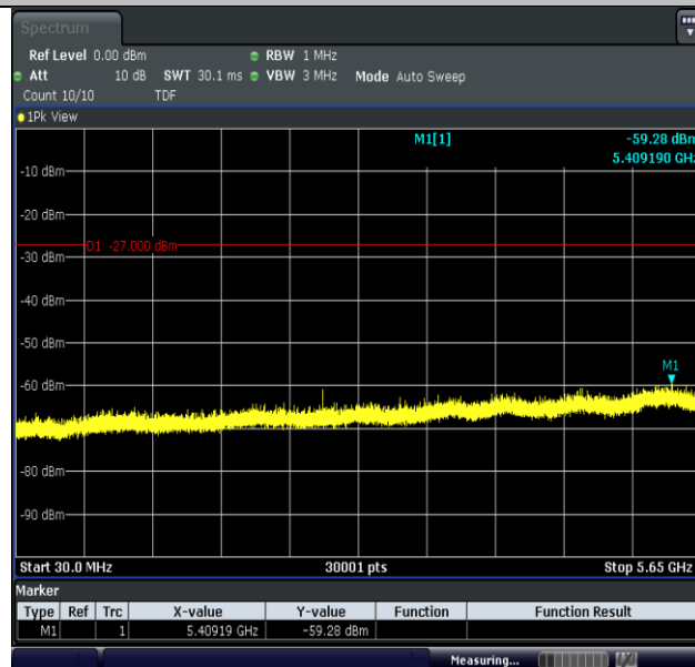
11A-Ant1-5745-30~5650-PASS
