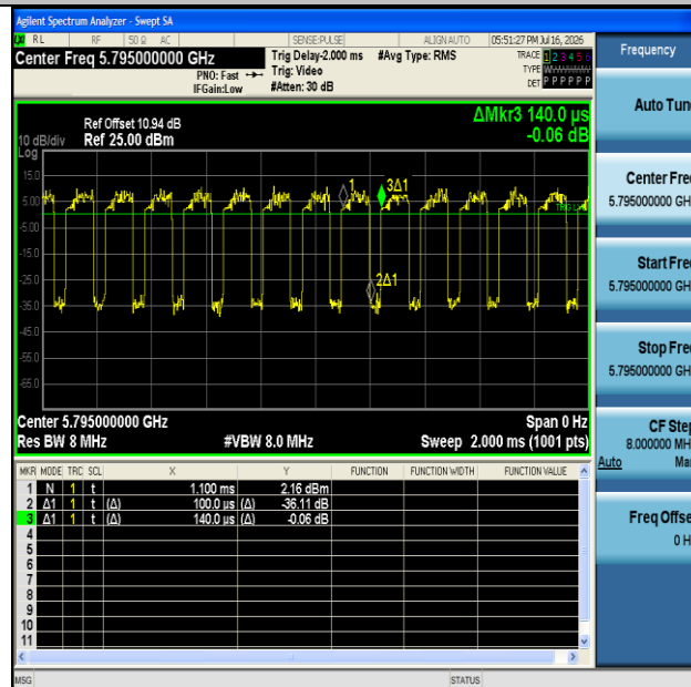
NTNV-11N40MIMO-Ant2-5795
