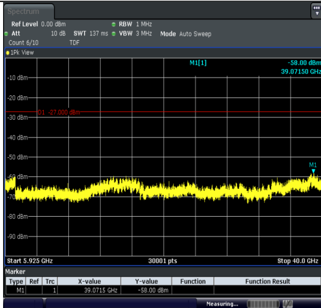
11N20MIMO-Ant2-5745-5925~40000-PASS
