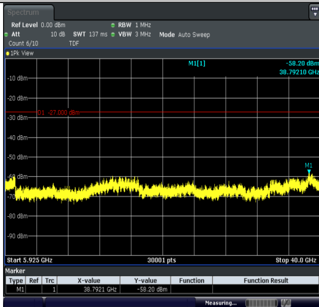
11A-Ant2-5745-5925~40000-PASS
