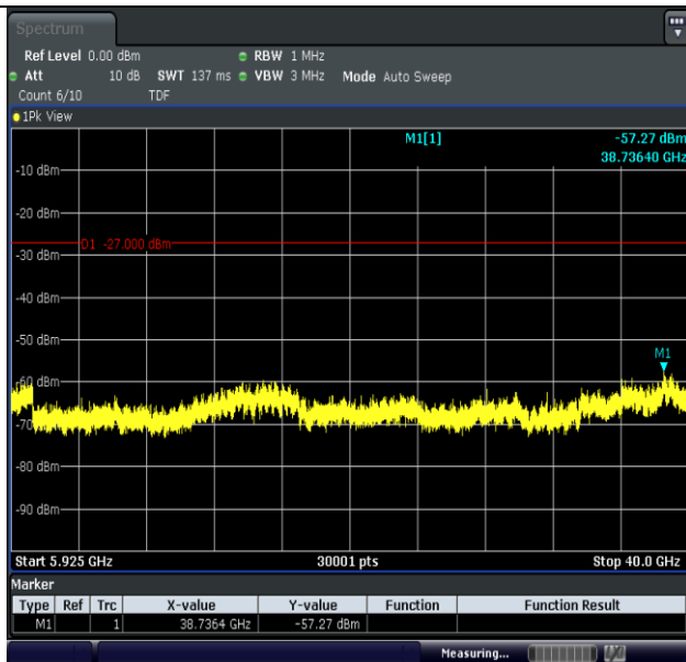
11AC40MIMO-Ant1-5795-5925~40000-PASS
