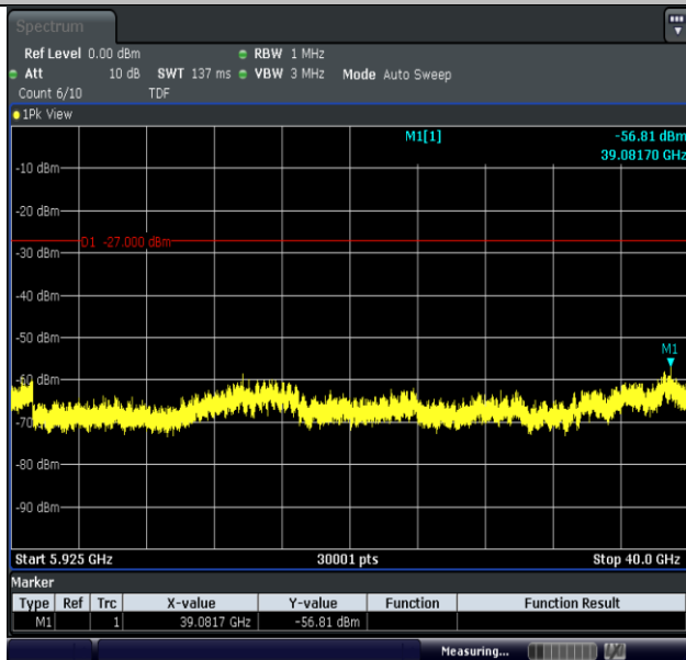
11A-Ant2-5785-5925~40000-PASS
