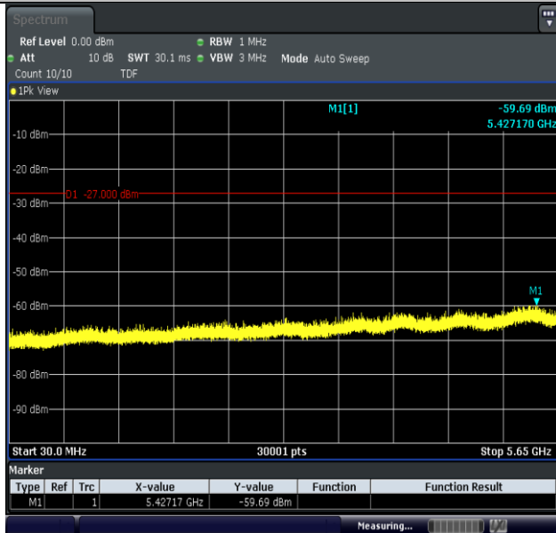
11N40MIMO-Ant2-5795-30~5650-PASS
