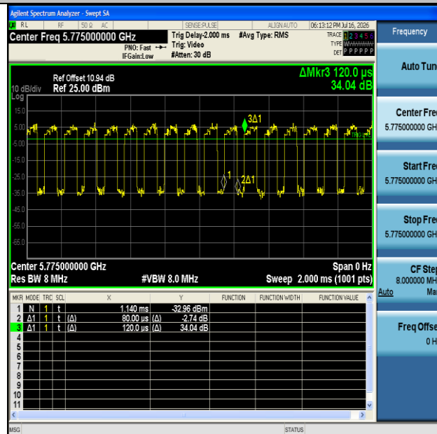
NTNV-11AC80MIMO-Ant2-5775
