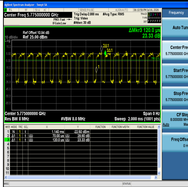
NTNV-11AC80MIMO-Ant1-5775
