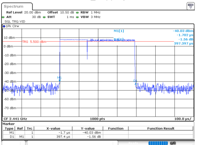
2DH1_Hopping
