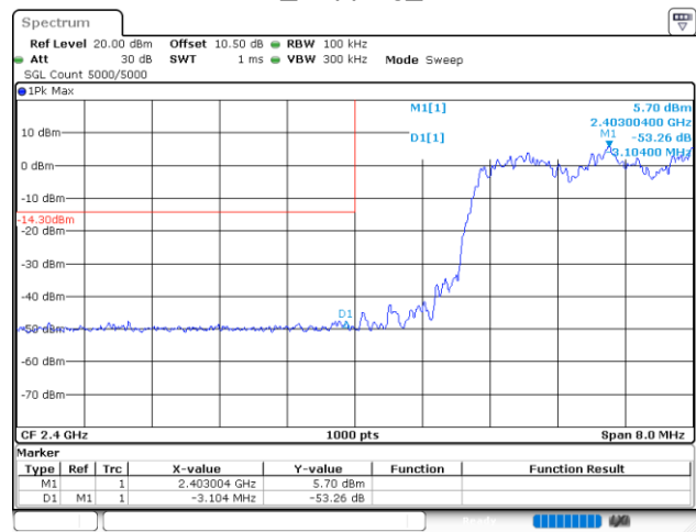
2DH1_Hopping_Lower
