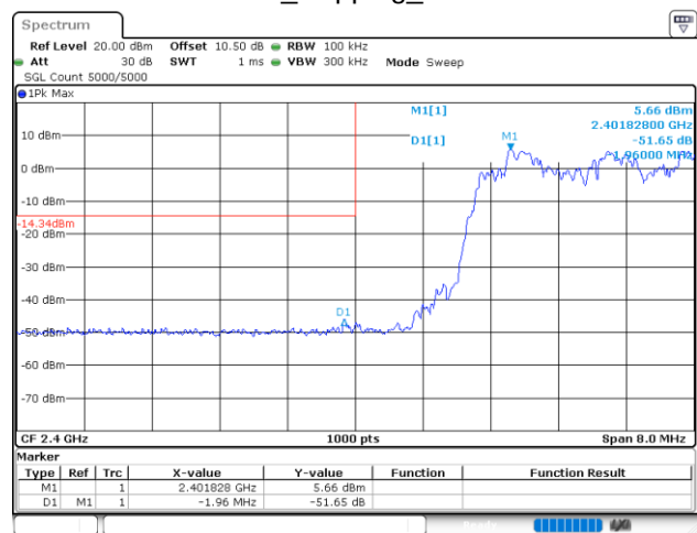
3DH1_Hopping_Lower
