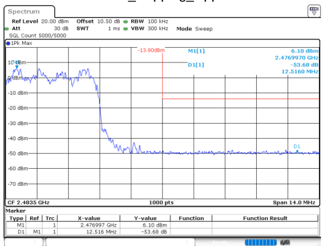
3DH1_Hopping_Upper
