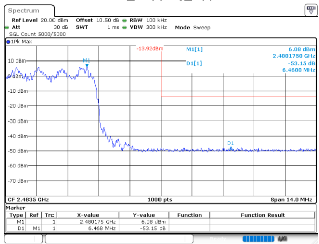
2DH1_Hopping_Upper
