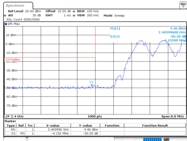
DH1_Hopping_Lower
