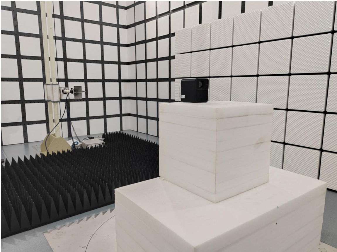
Radiated Spurious Emissions Test Side View (18GHz-40GHz)
