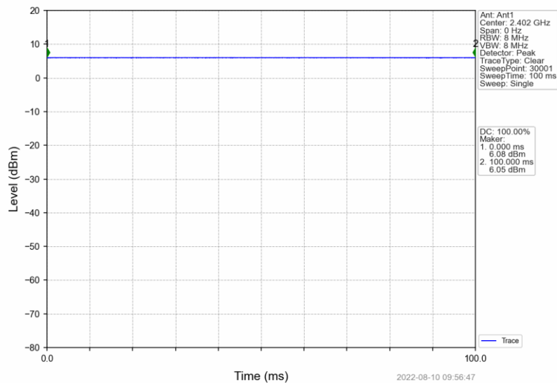
2M_LCH_2402MHz_Ant1_NTNV
