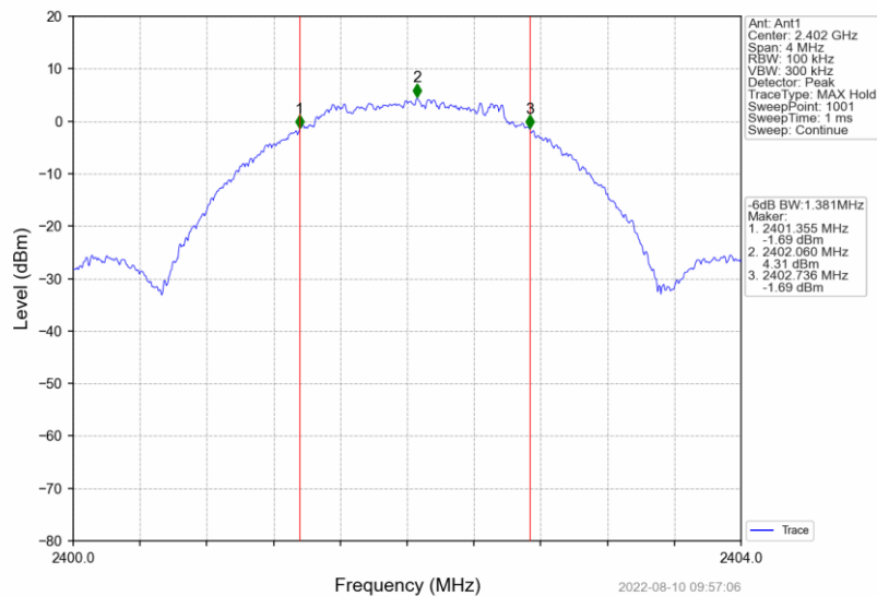
2M_LCH_2402MHz_Ant1_NTNV
