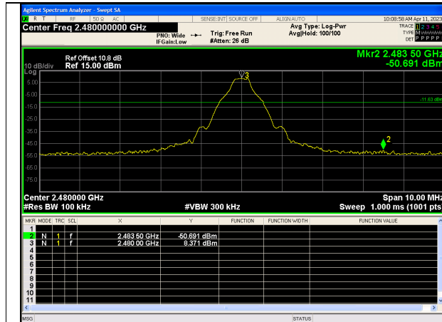
Out Of Band Emission GFSK_DH5_Channel 78
