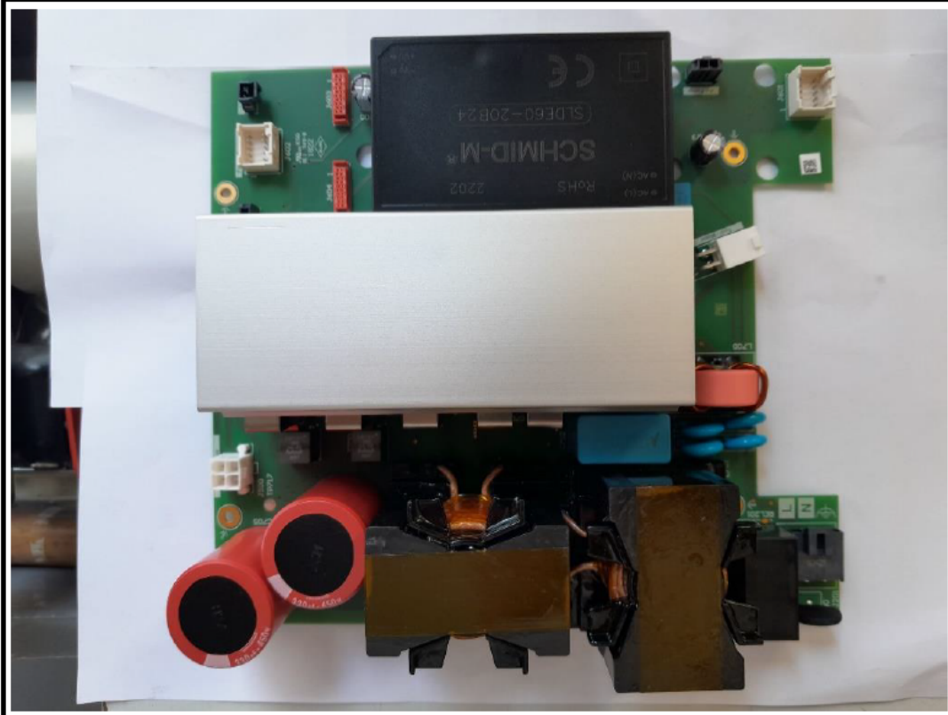
EUT MAIN PCB TOP SIDE
