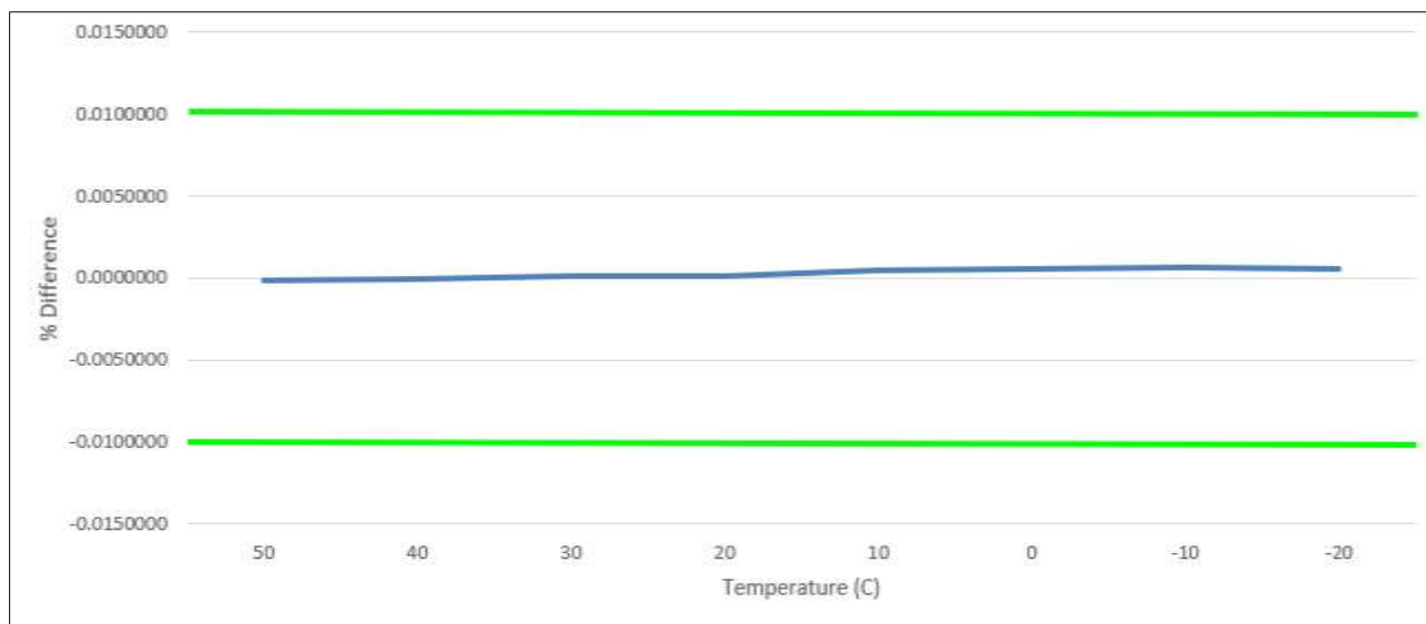
Plot 13. Frequency Stability vs Temperature
